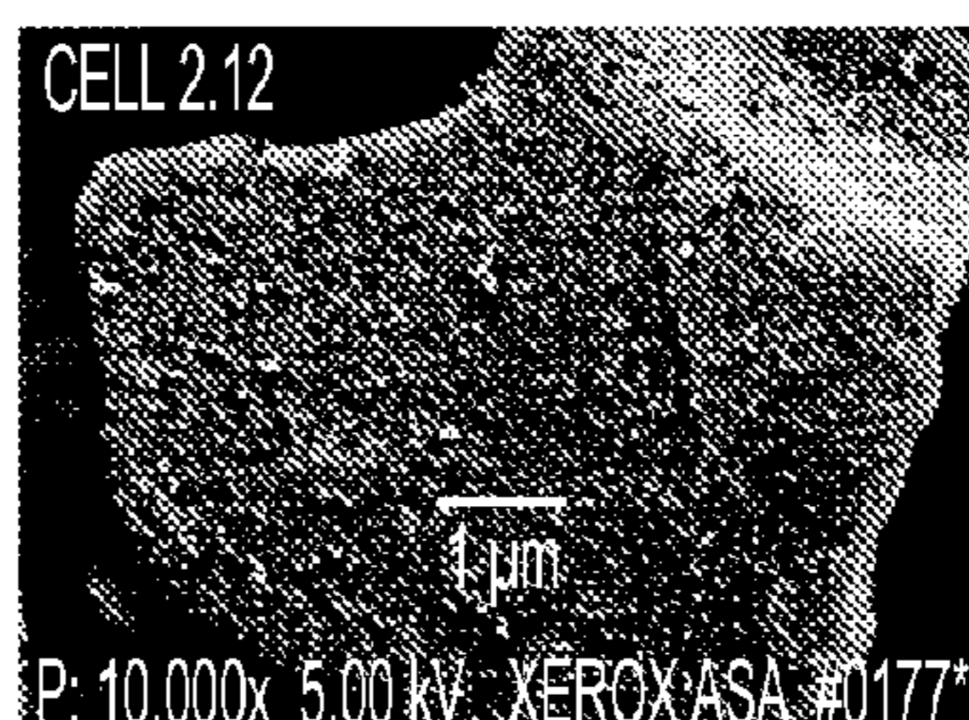
FRESH TONER PARTICLE WITH SURFACE ADDITIVES
