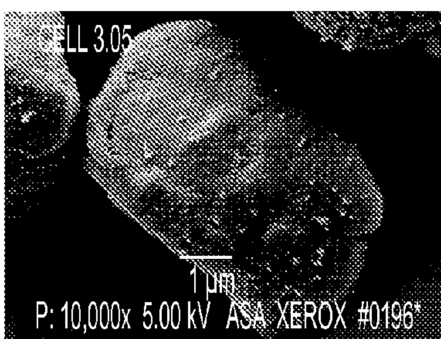
OLD TONER PARTICLE TWO MINUTES AFTER ADDITION OF FRESH TONER
