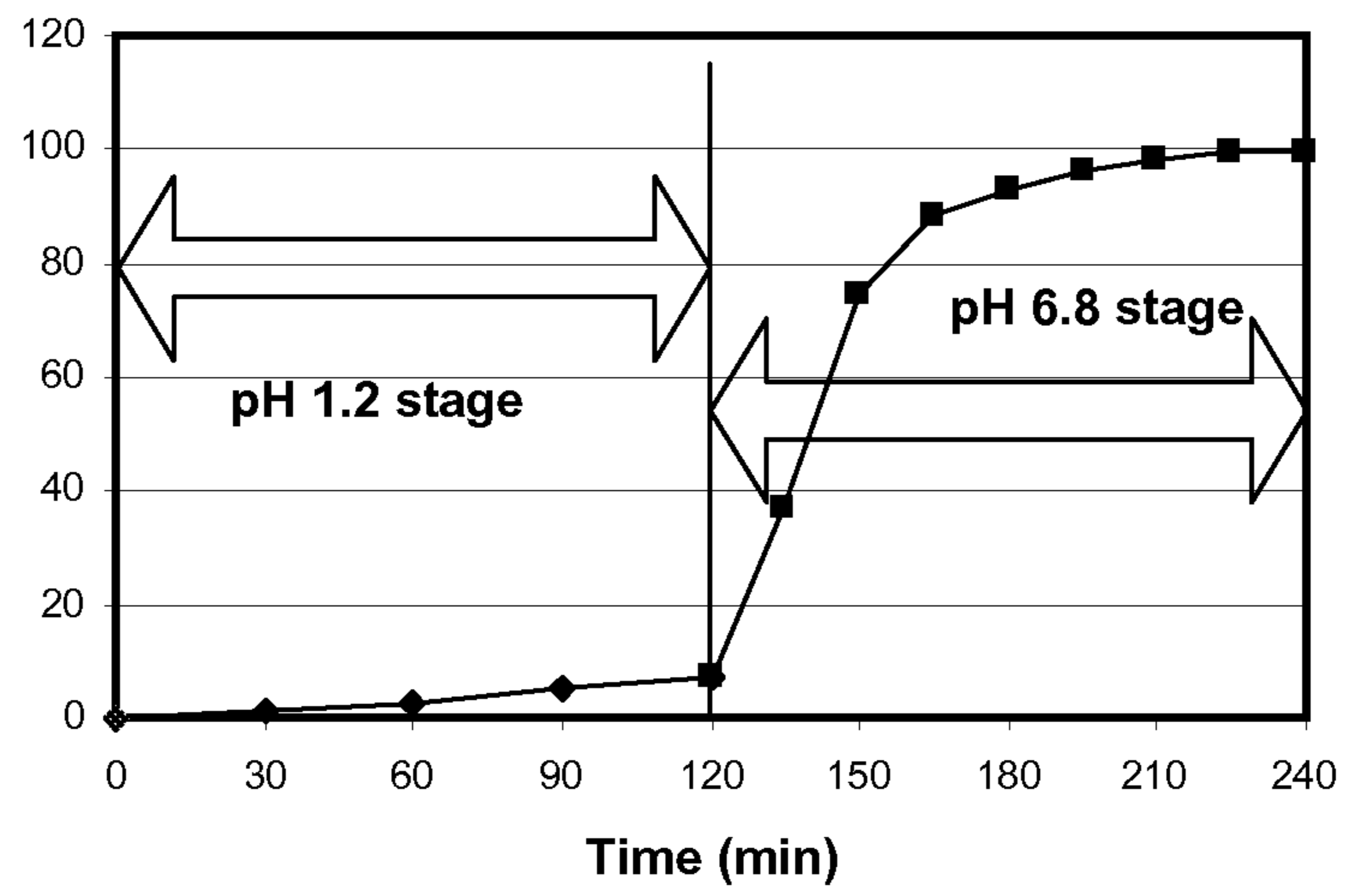
% APAP dissolved
