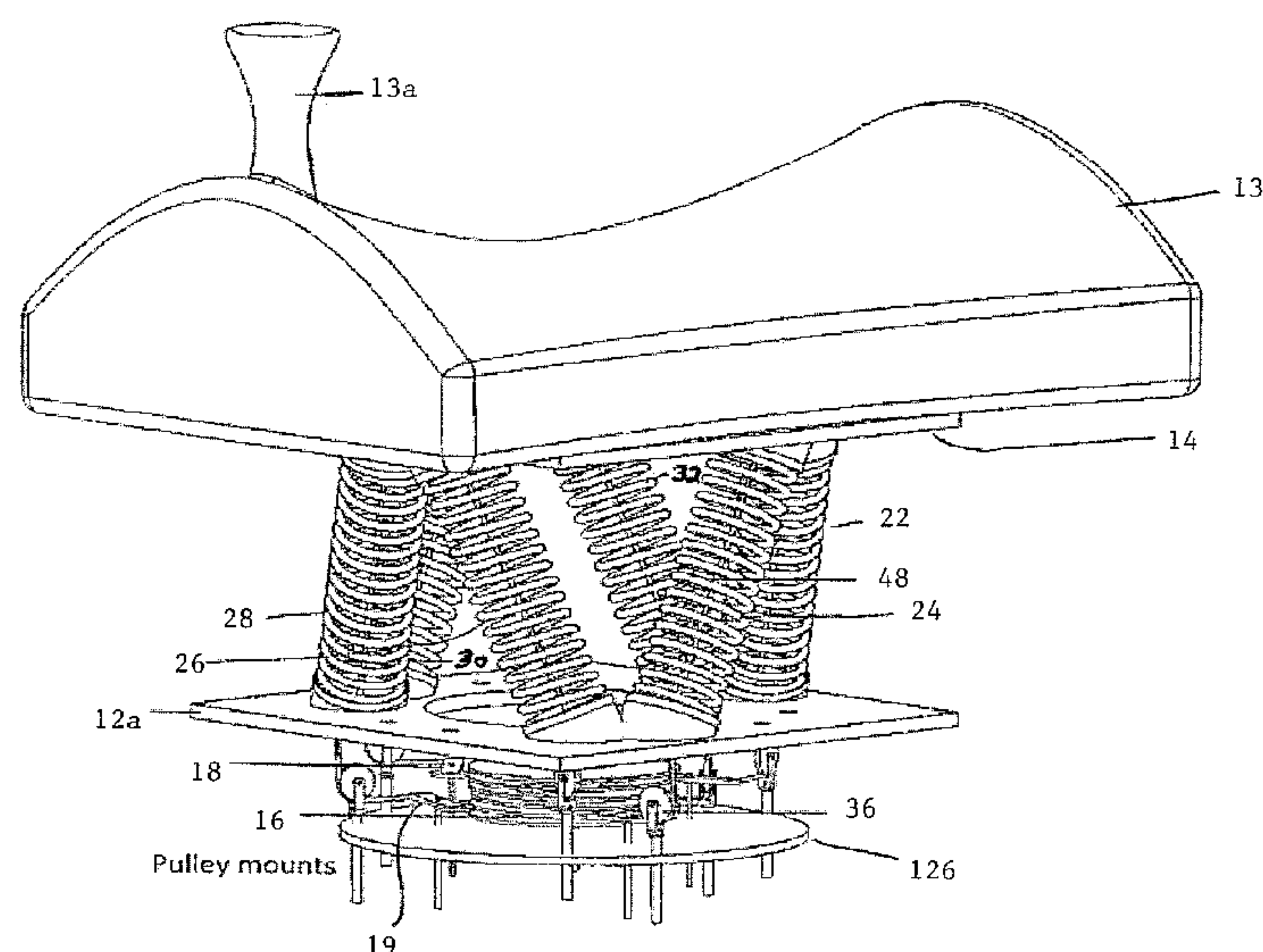
Spring And Cam (SNC) Configuration
