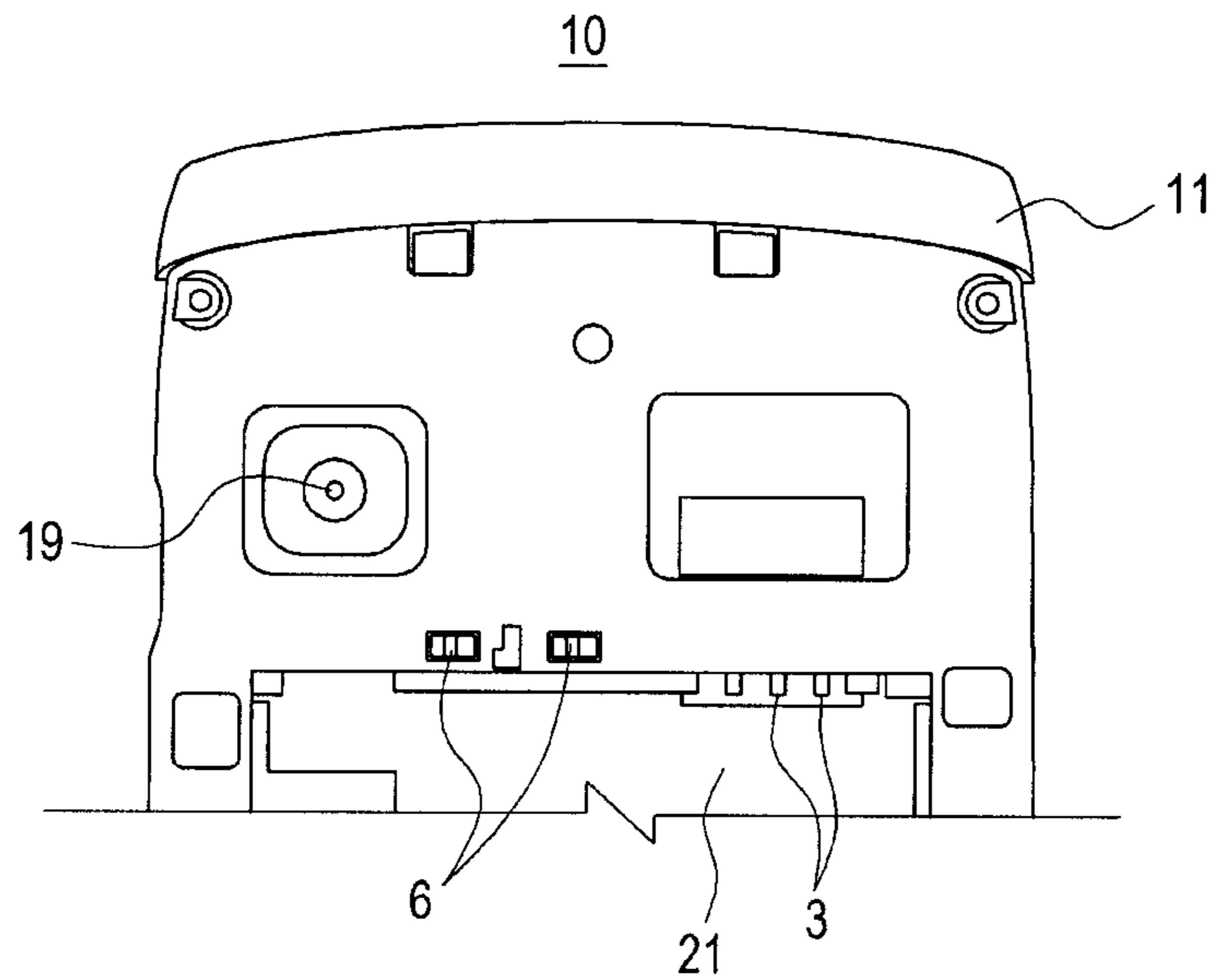
FIG. 4 (PRIOR ART)
