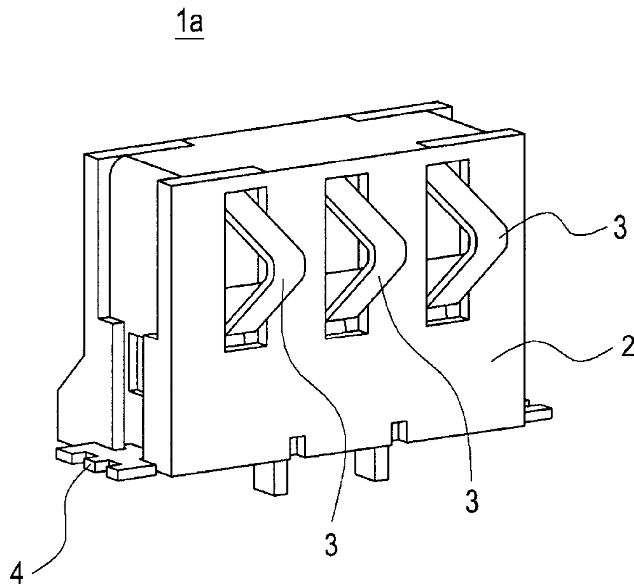
FIG. 1 (PRIOR ART)
