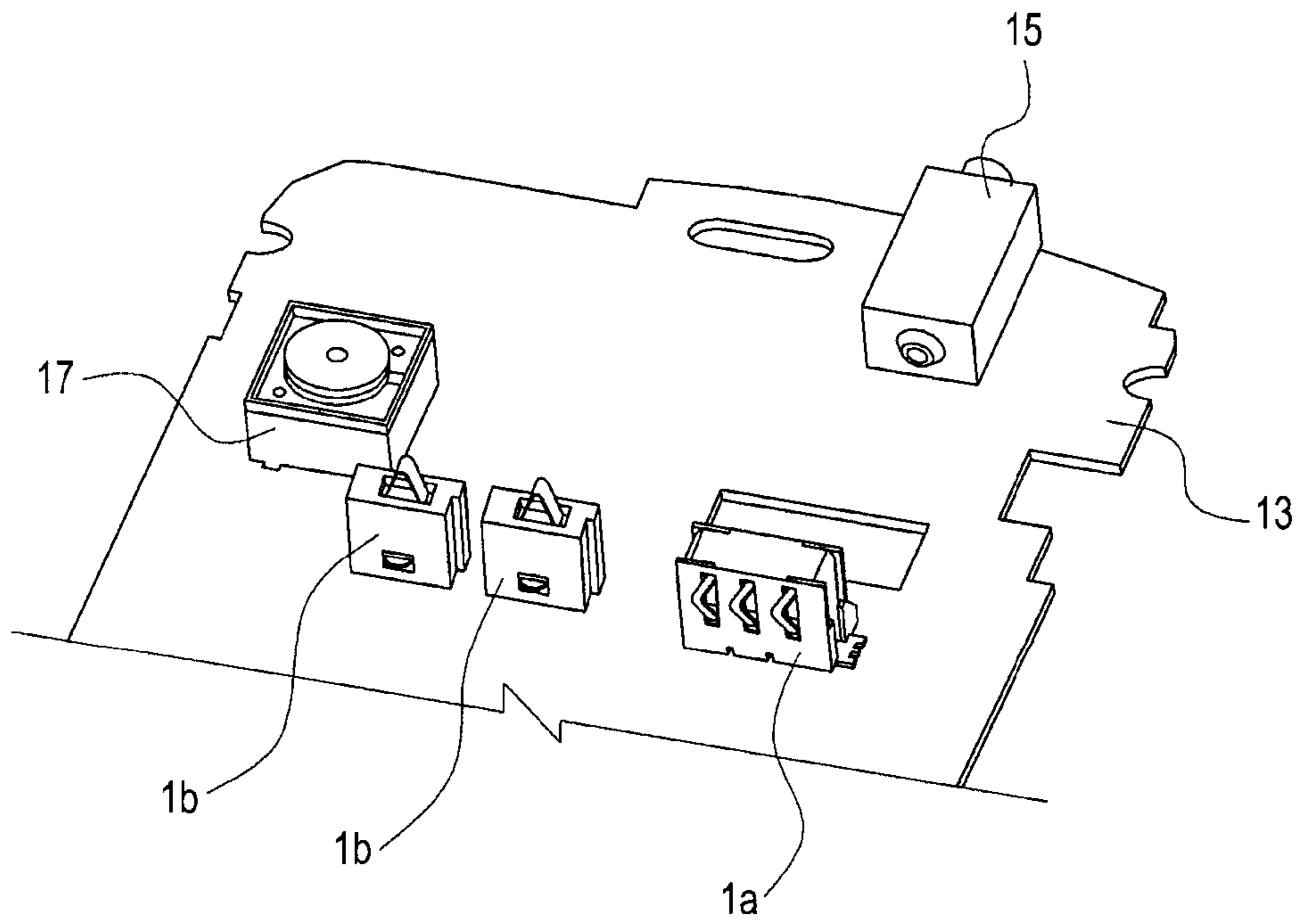
FIG. 3 (PRIOR ART)
