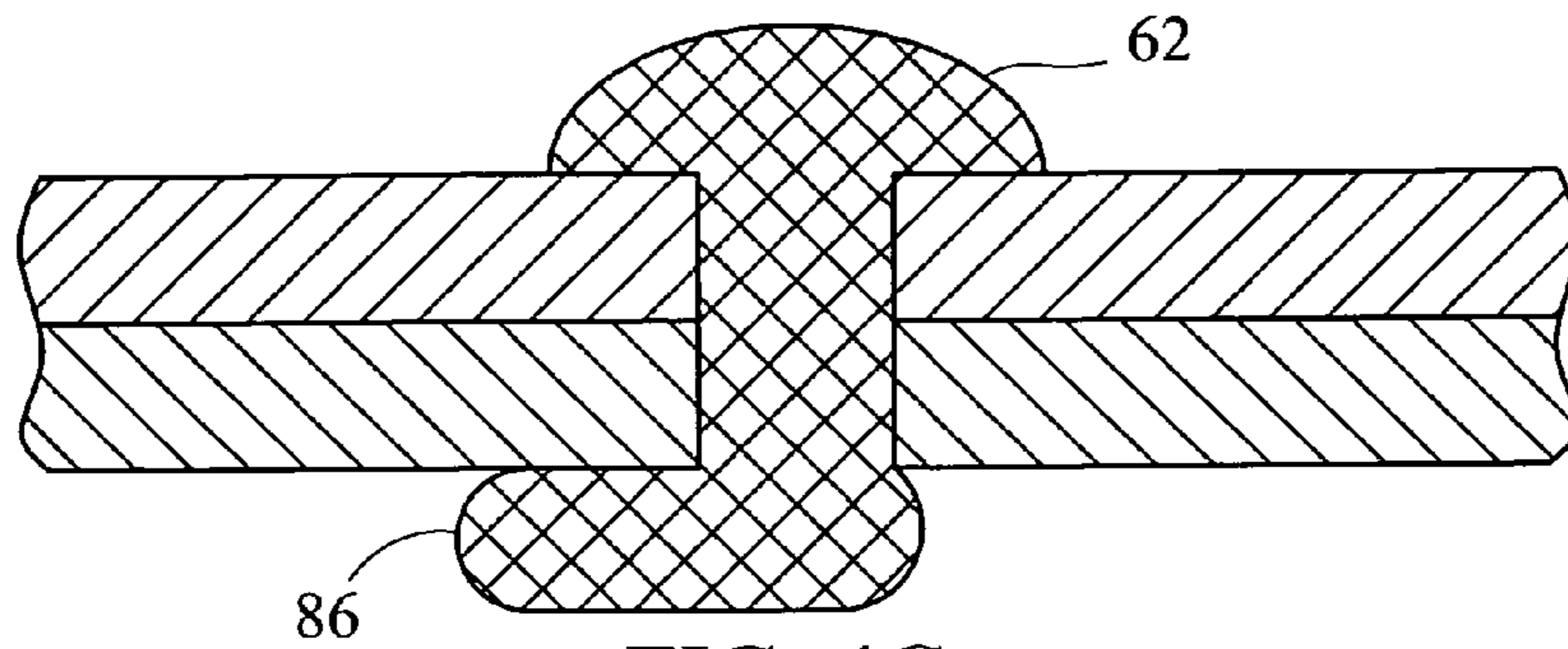
FIG. 4C PRIOR ART
