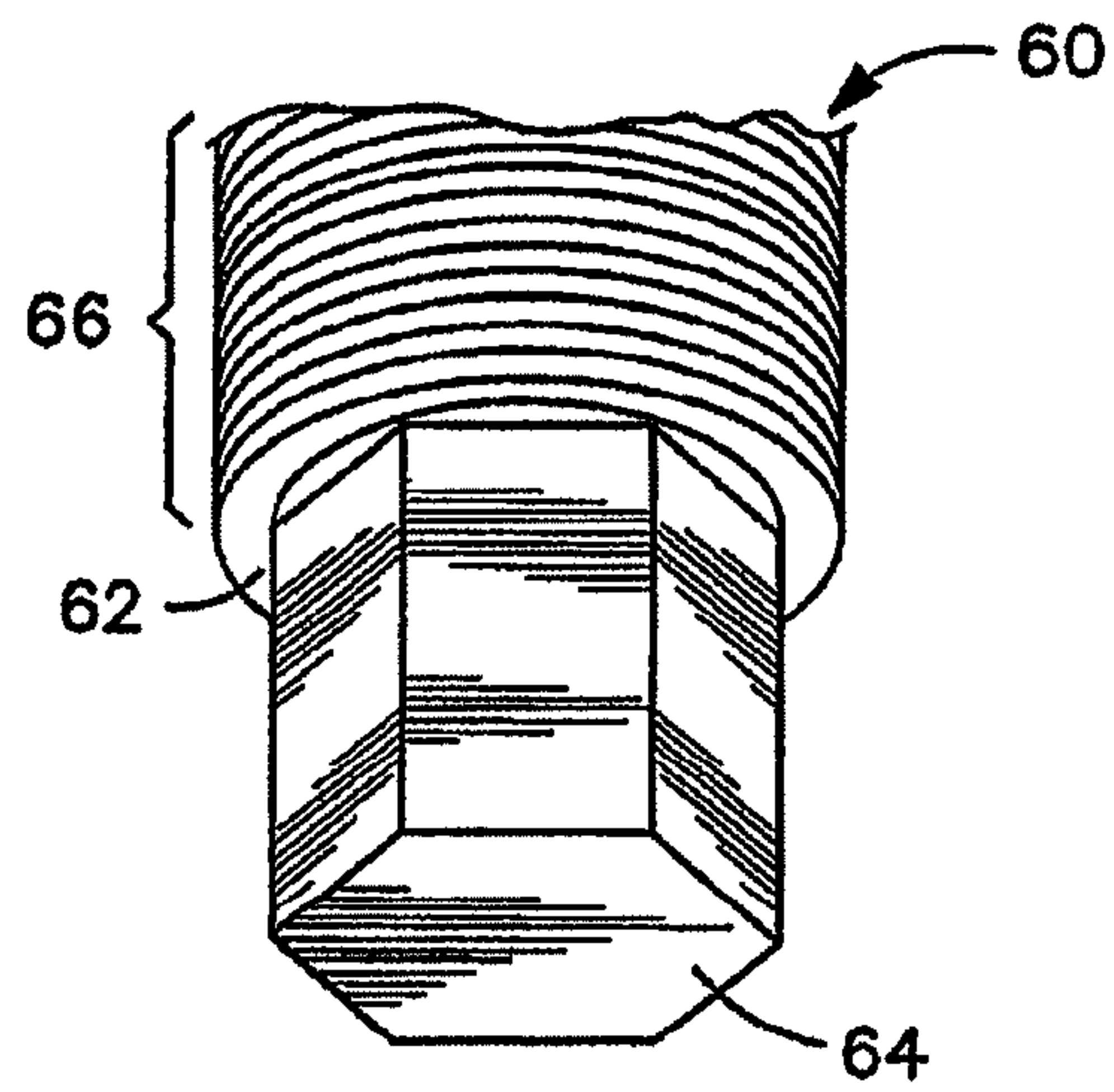
FIG. 4 PRIOR ART
