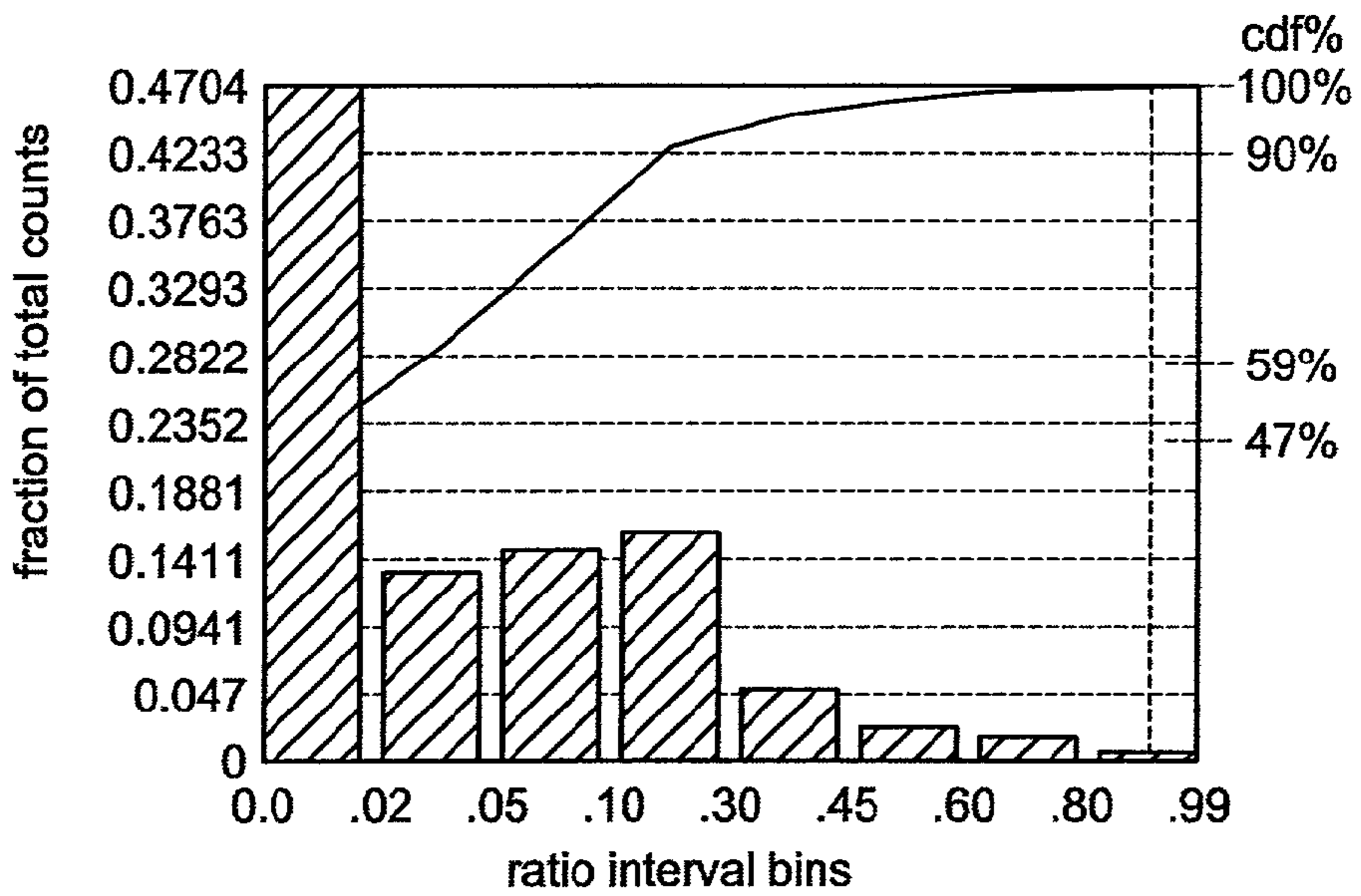
1657 user, time hopped away before returning to program ratio:HopdT/time-avilable
