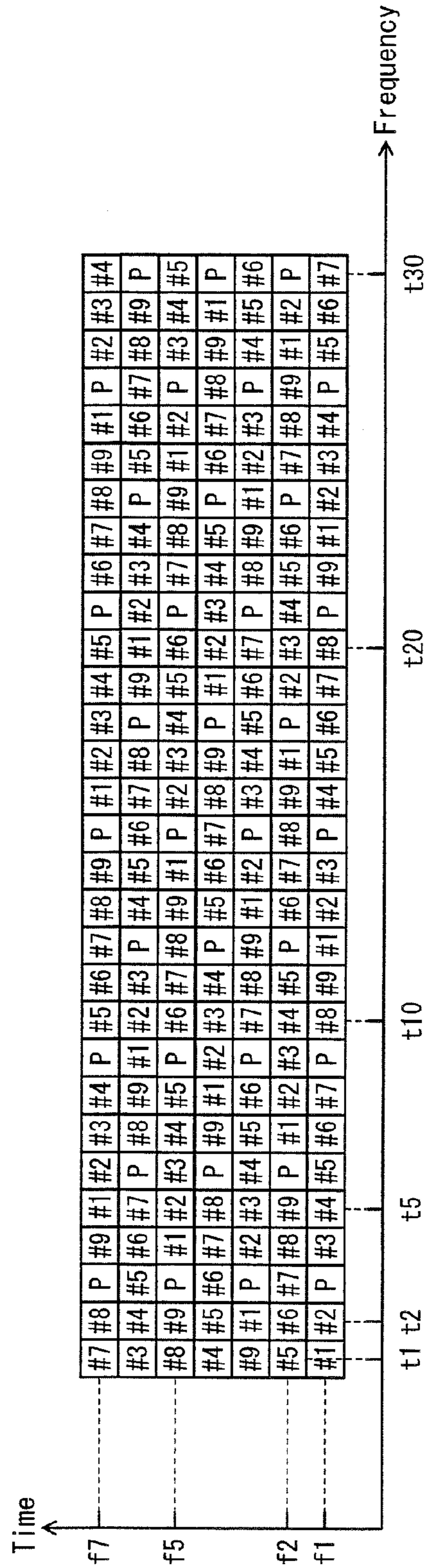
FIG. 80B Modulated signal z2
