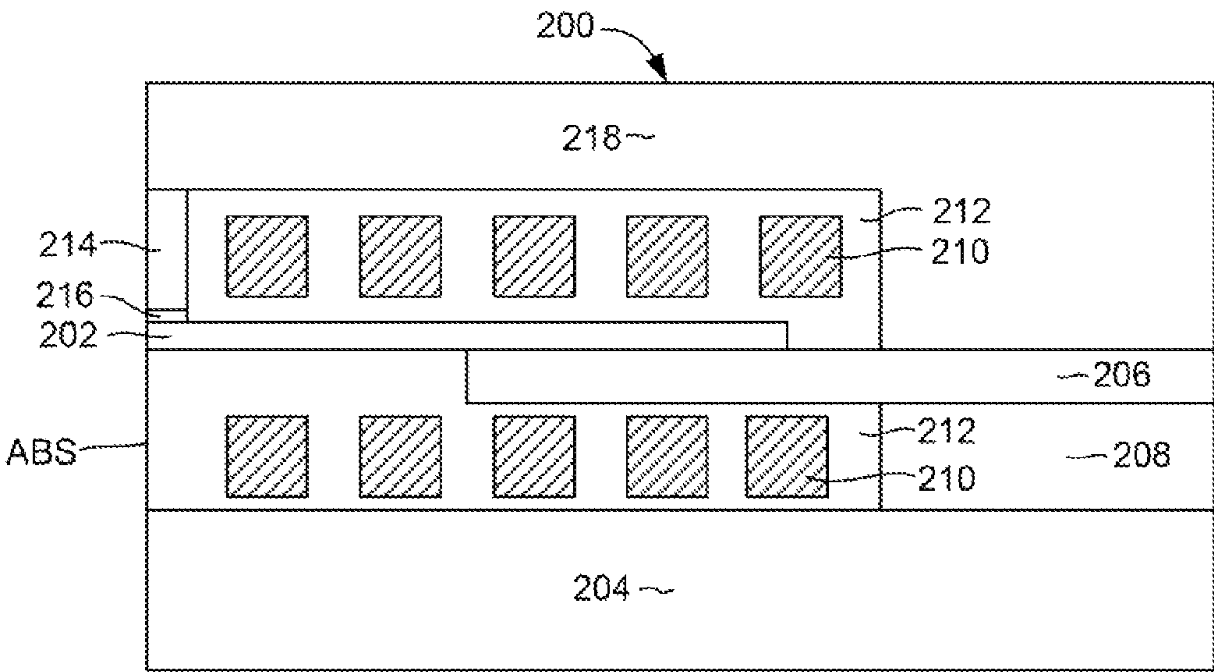
FIG. 2 (prior art)
