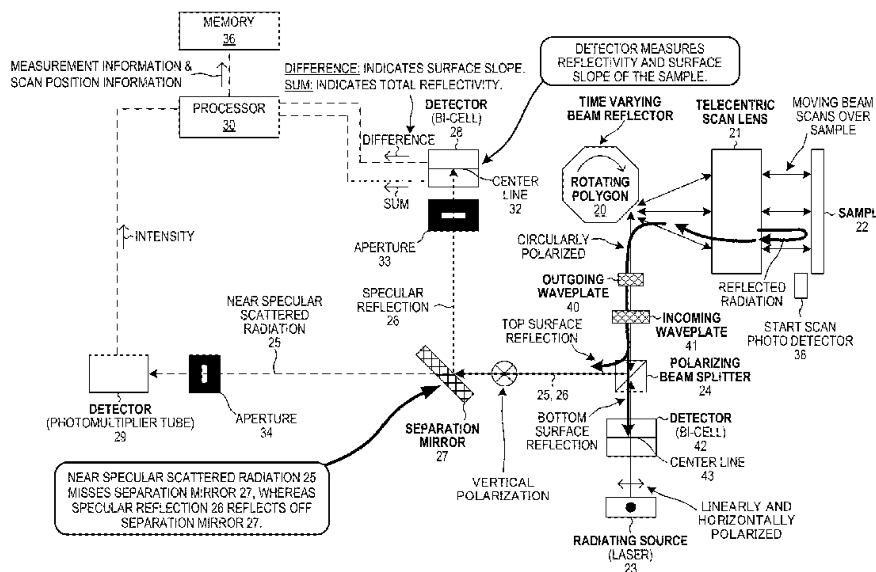
TOP VIEW OPTICAL INSPECTOR
