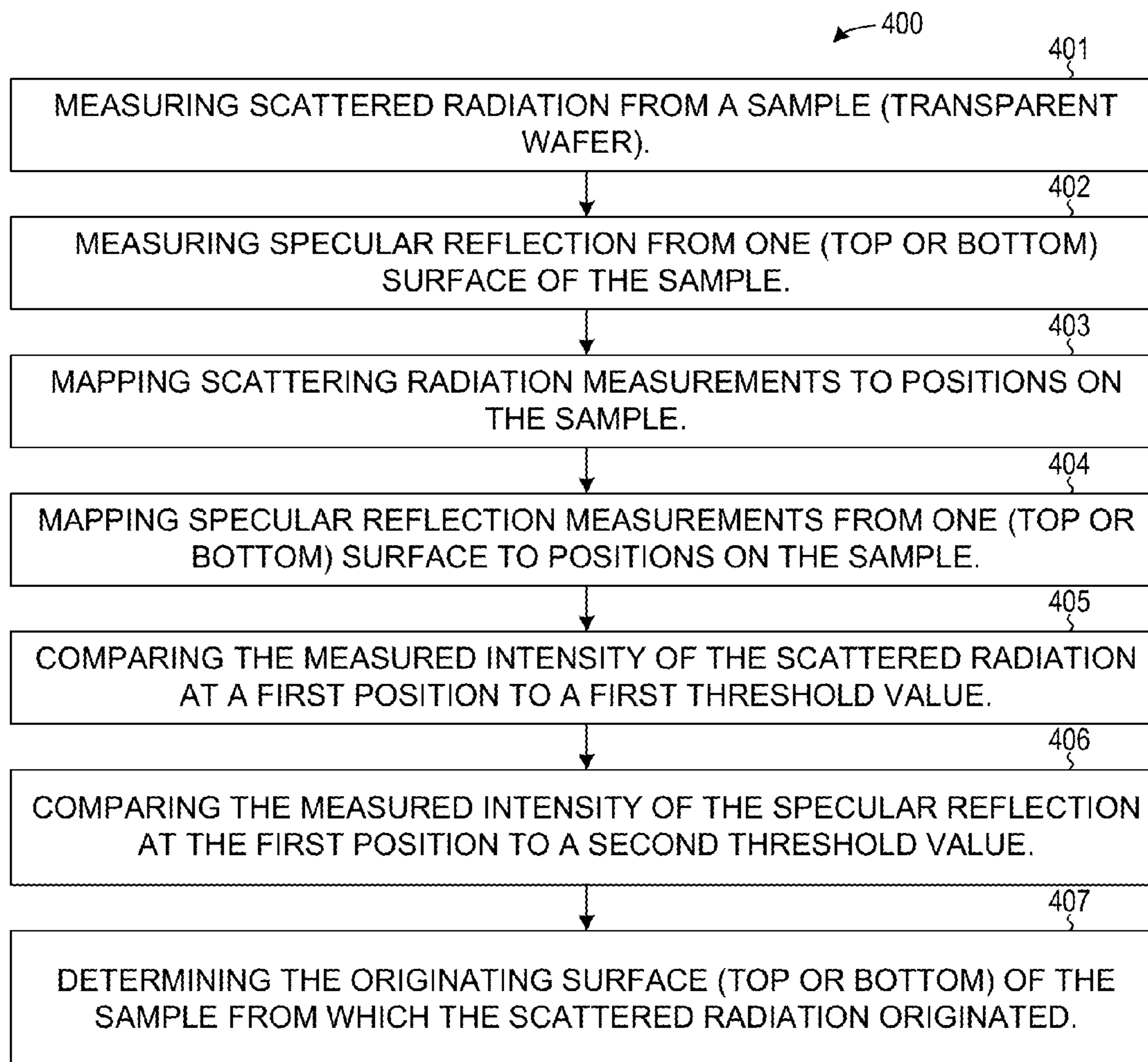
OPTICAL INSPECTION FLOWCHART FIG. 22
