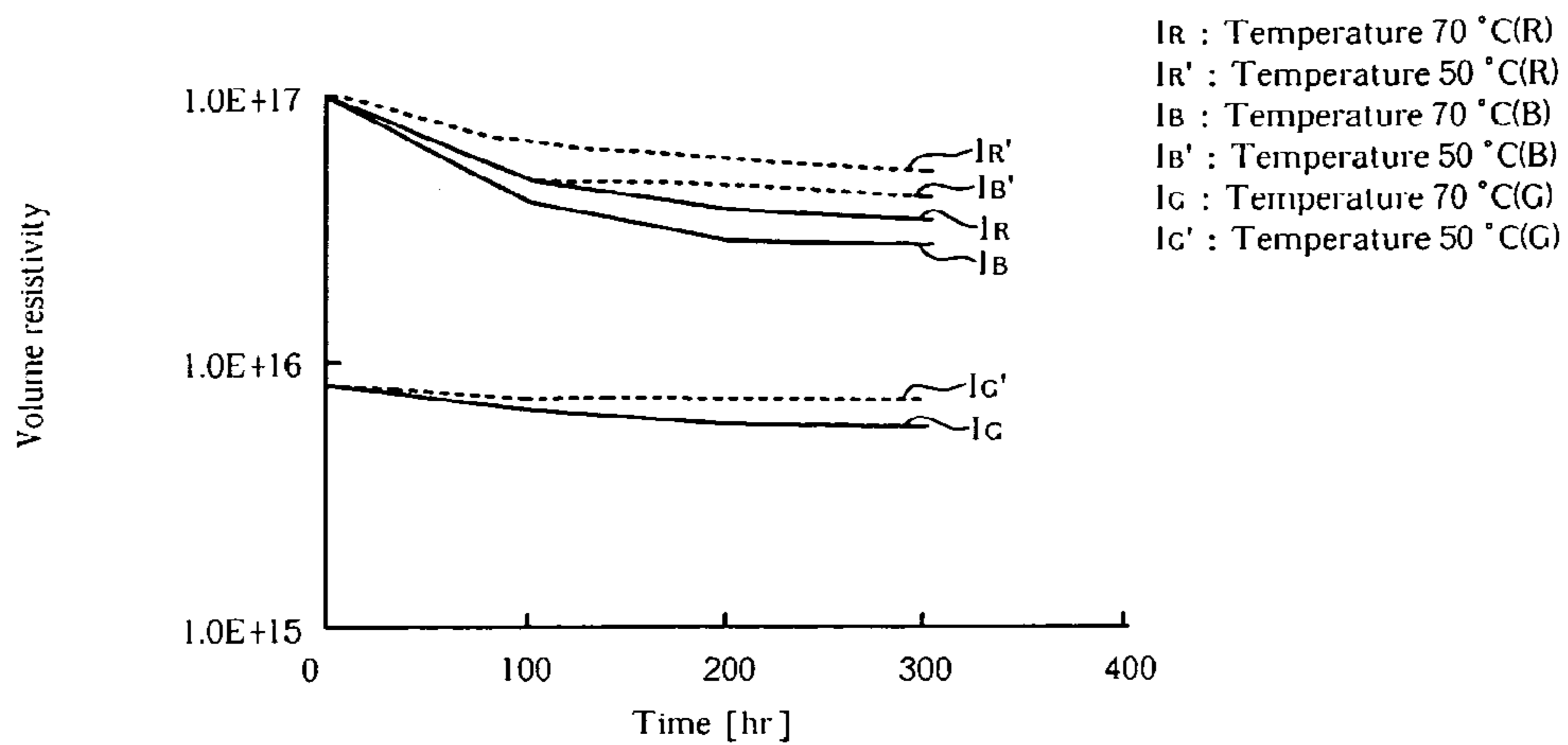
Fig. 9 Prior art
