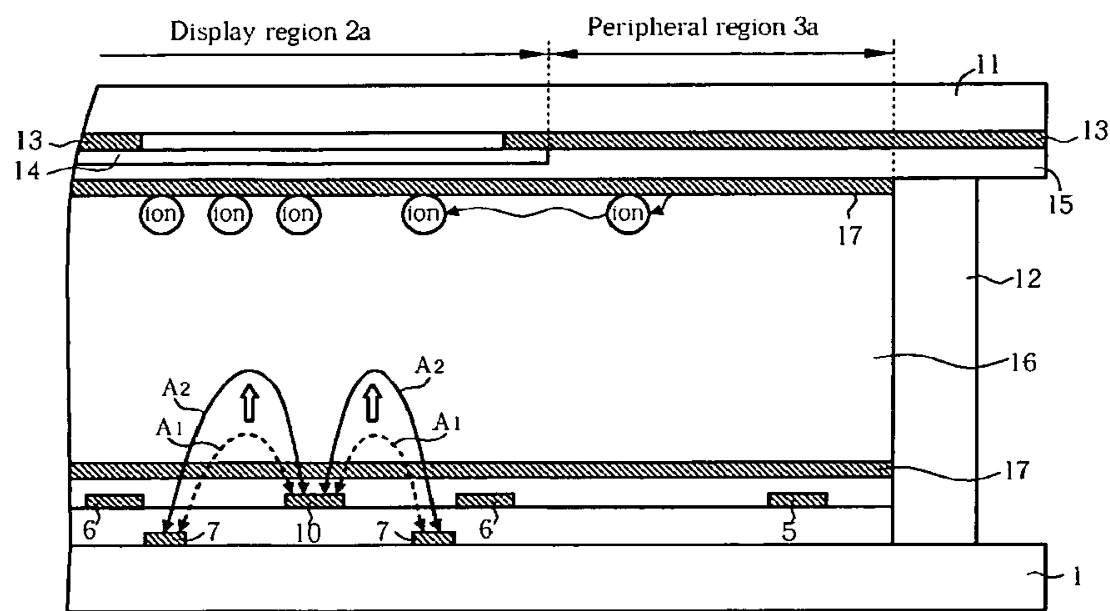
Fig. 4 Prior art
