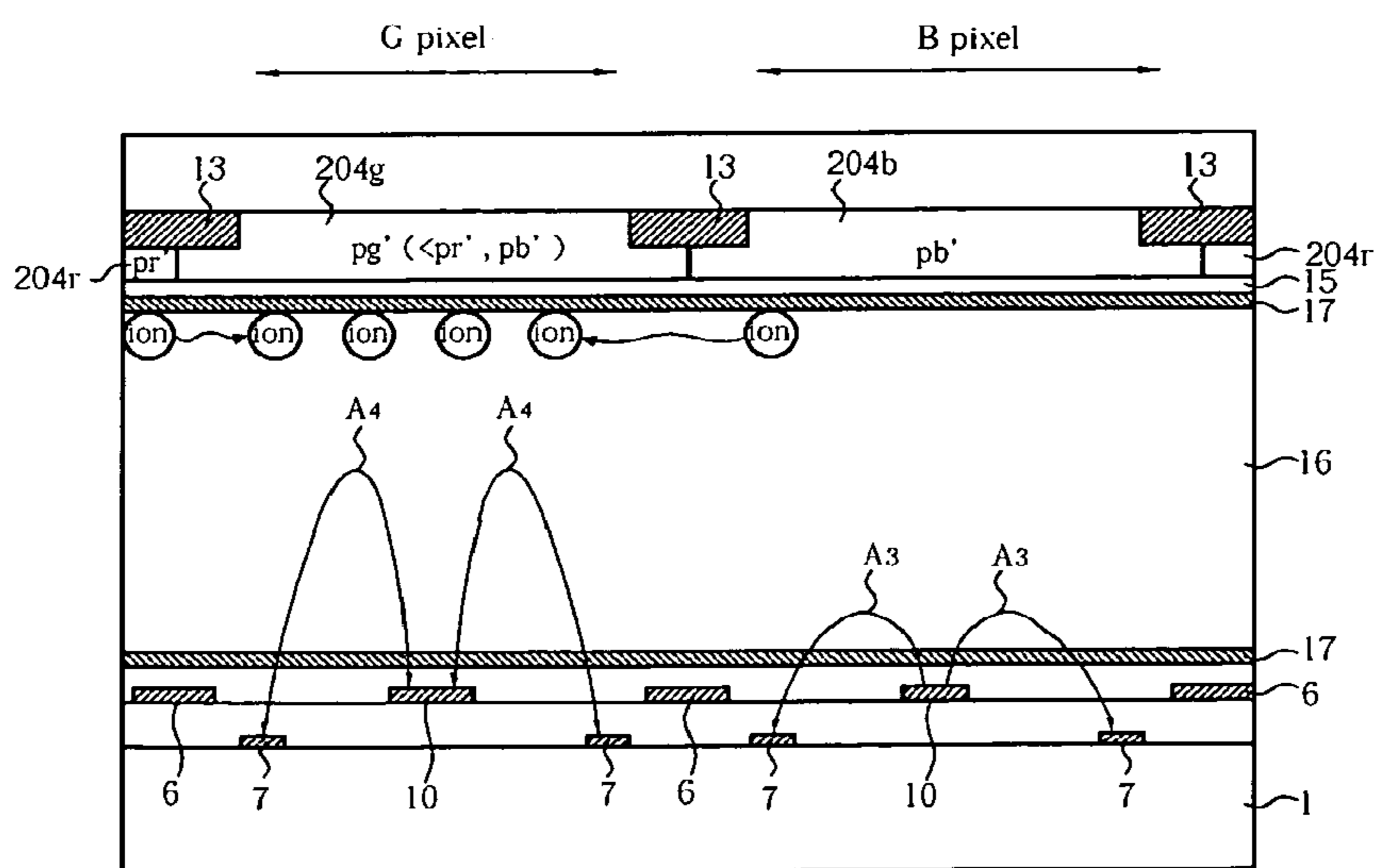
Fig. 10 Prior art
