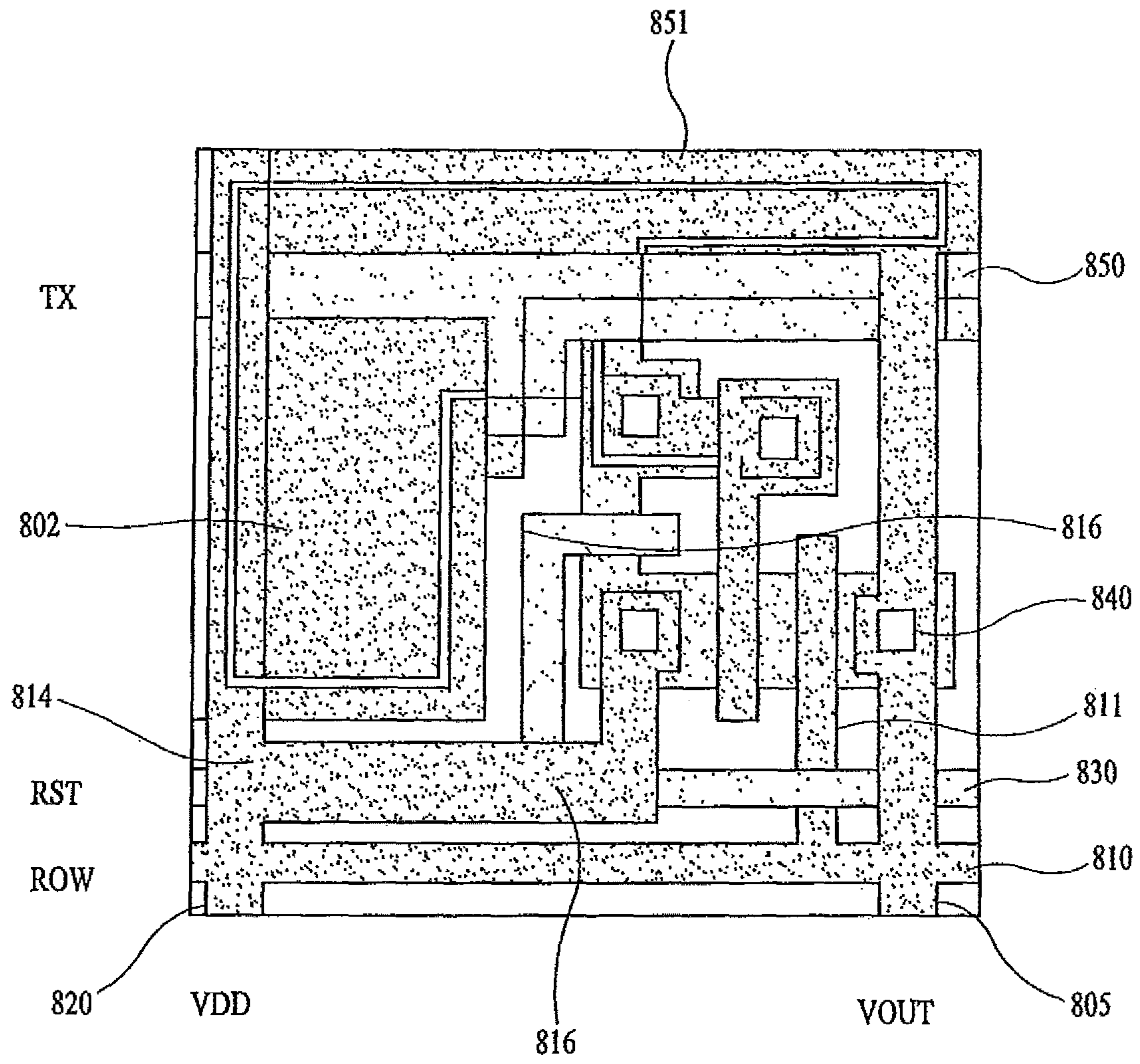
FIG. 7 (PRIOR ART)
