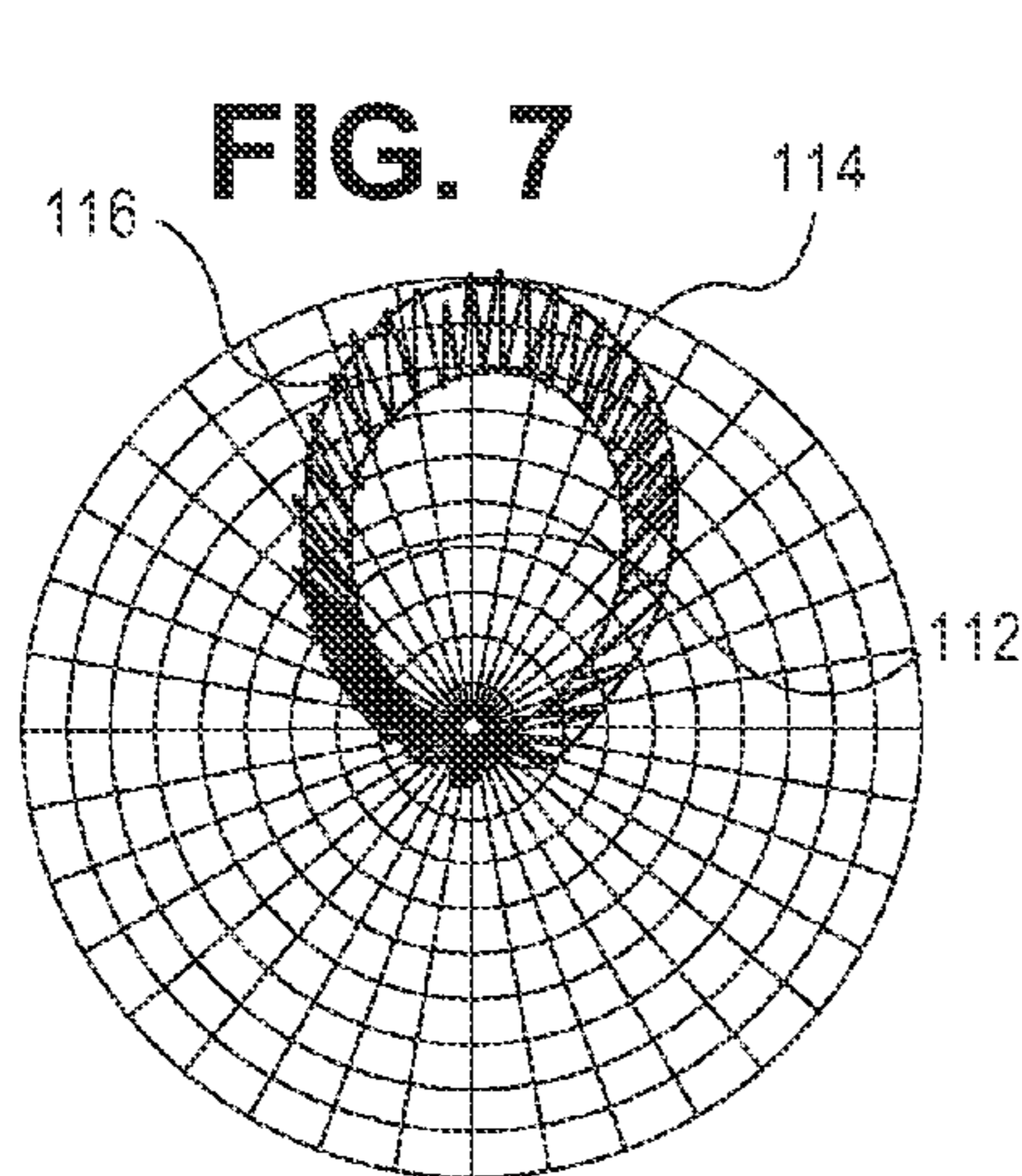
AZIMUTH PATTERN F = 713 MHz HPOL = 81%
