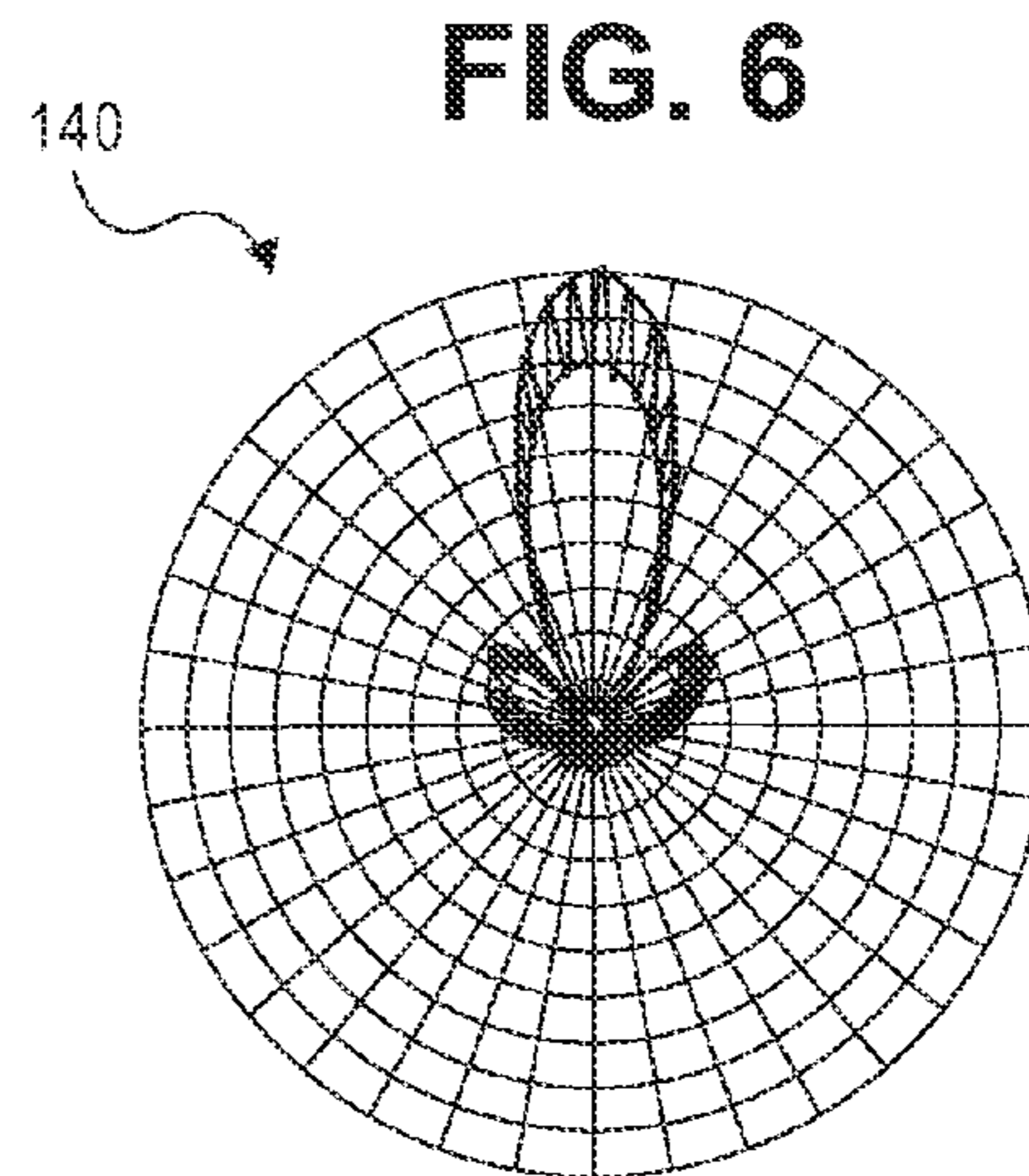
ELEVATION PATTERN F = 698 MHz VPOL = 80%
