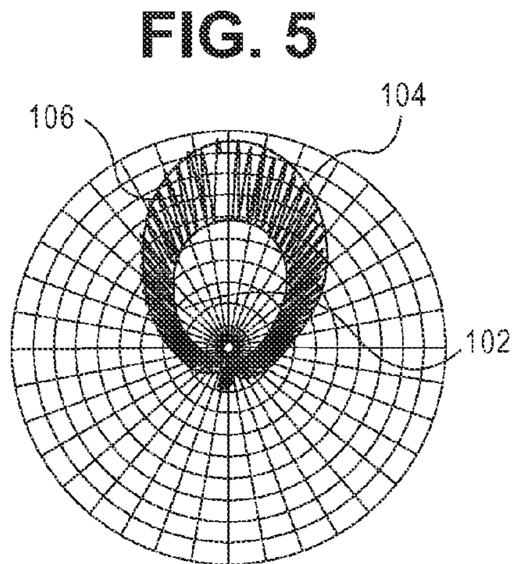
AZIMUTH PATTERN F = 698 MHz HPOL = 64%
