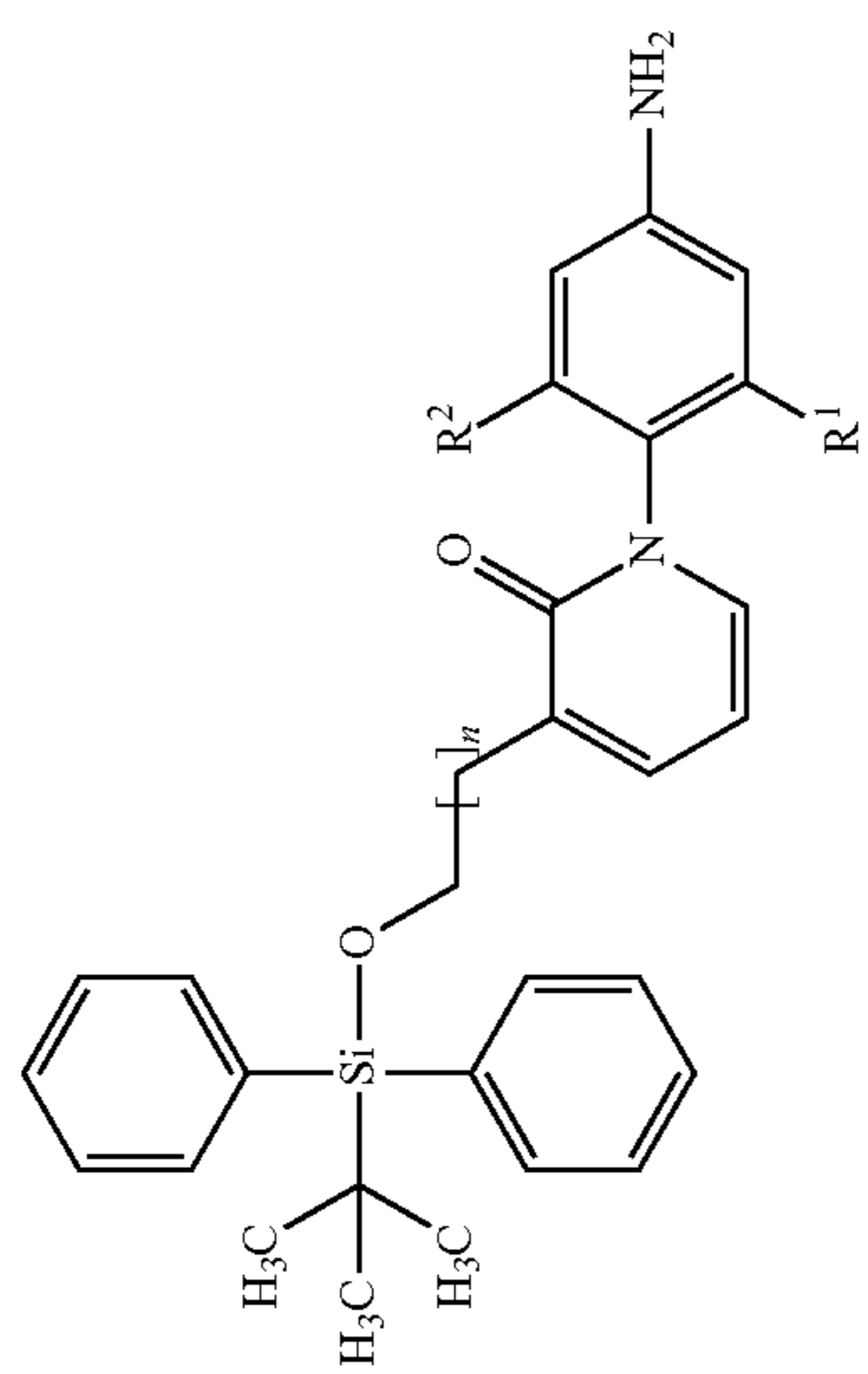
Scheme 1:
