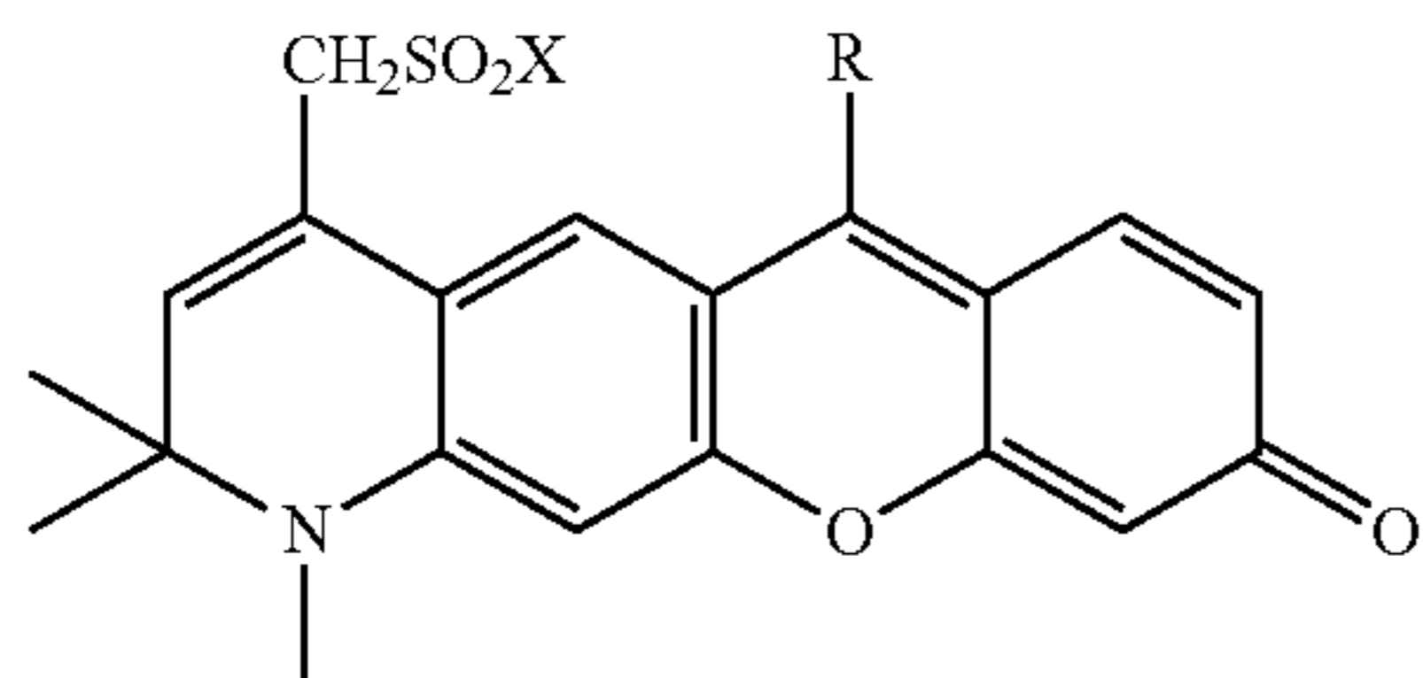
rhodol dyes
