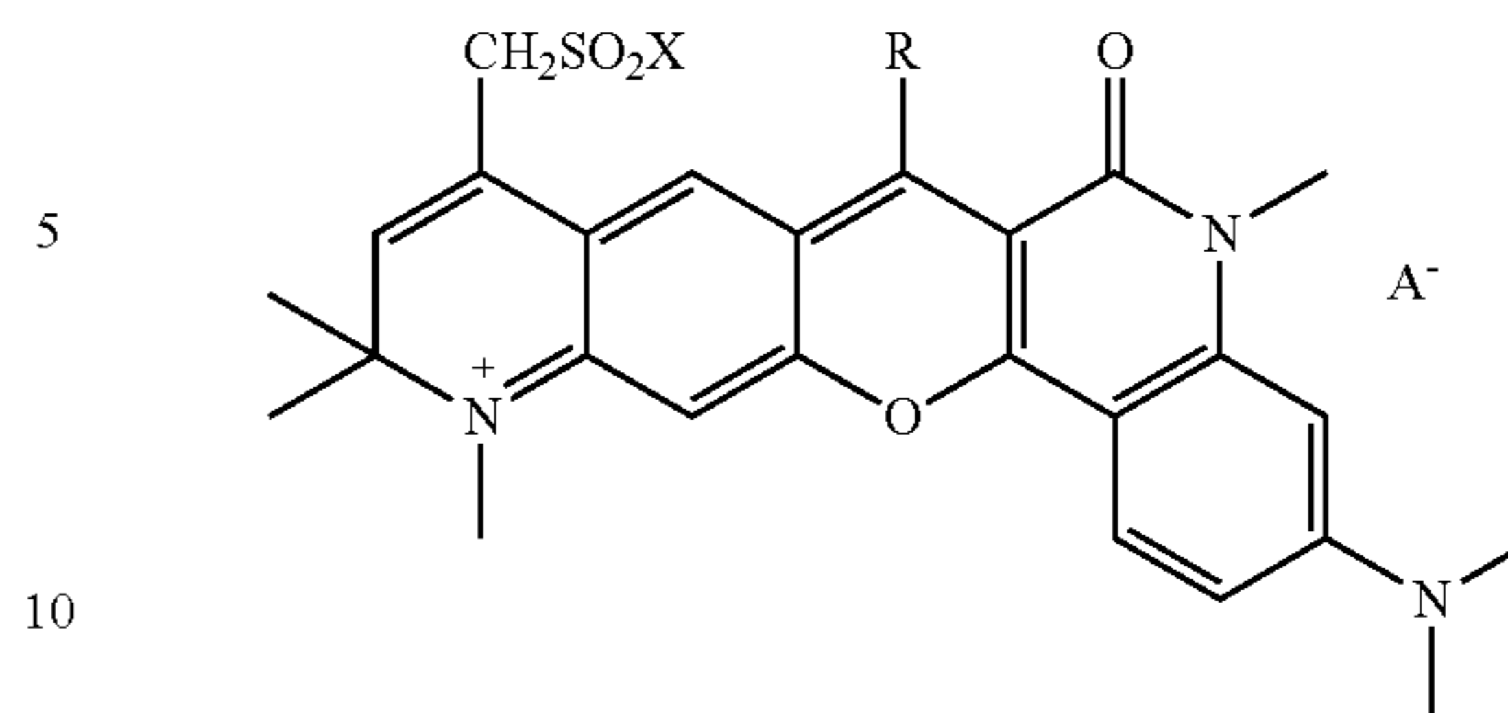
amidopyrylium dyes
