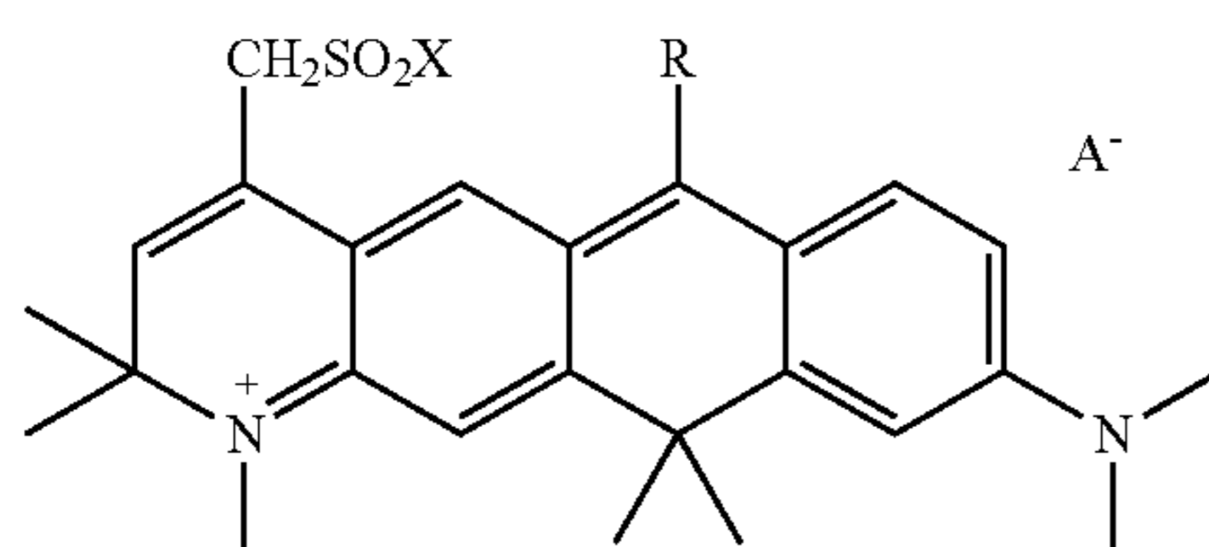
carbopyronines
