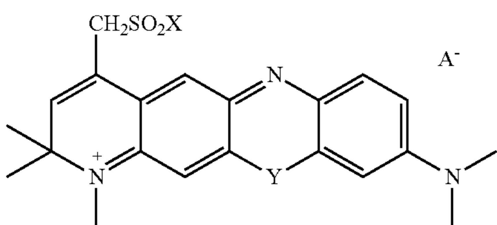
azine dyes Y = O (oxazines), S (thiazines), CR 2 (carbazines)
