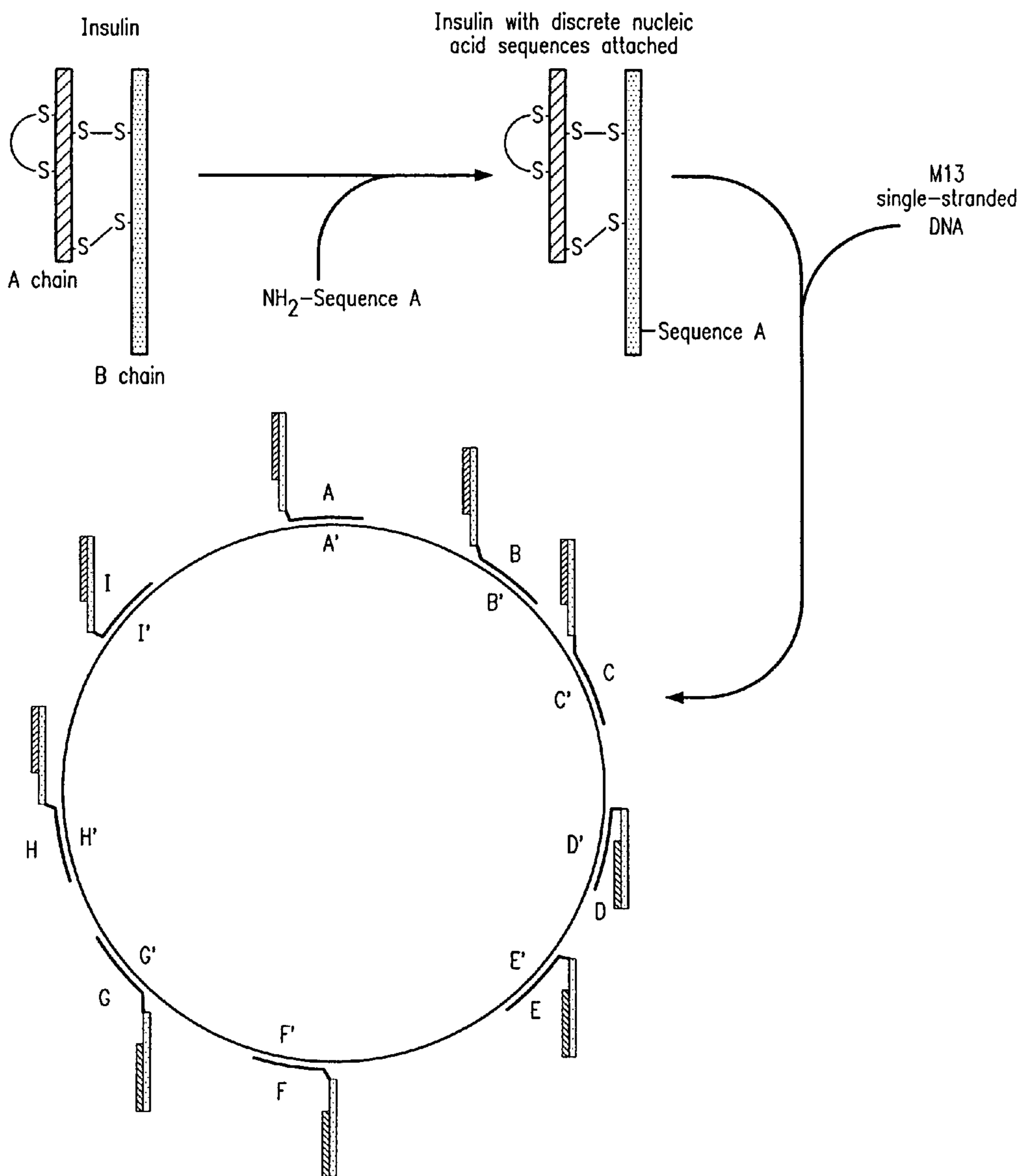
FIG. 23 Multimerization of Insulin molecules by hybridization to discrete Sequences
