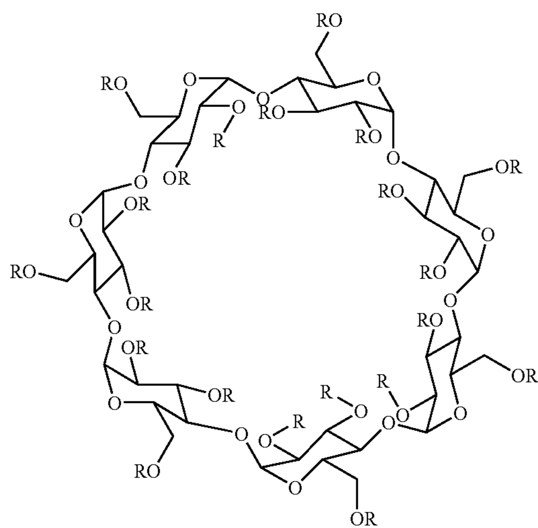
R = H \beta -cyclodextrin R = \text{CH}_2\text{CH}(\text{OH})\text{CH}_3 hydroxypropyl \beta -cyclodextrin
