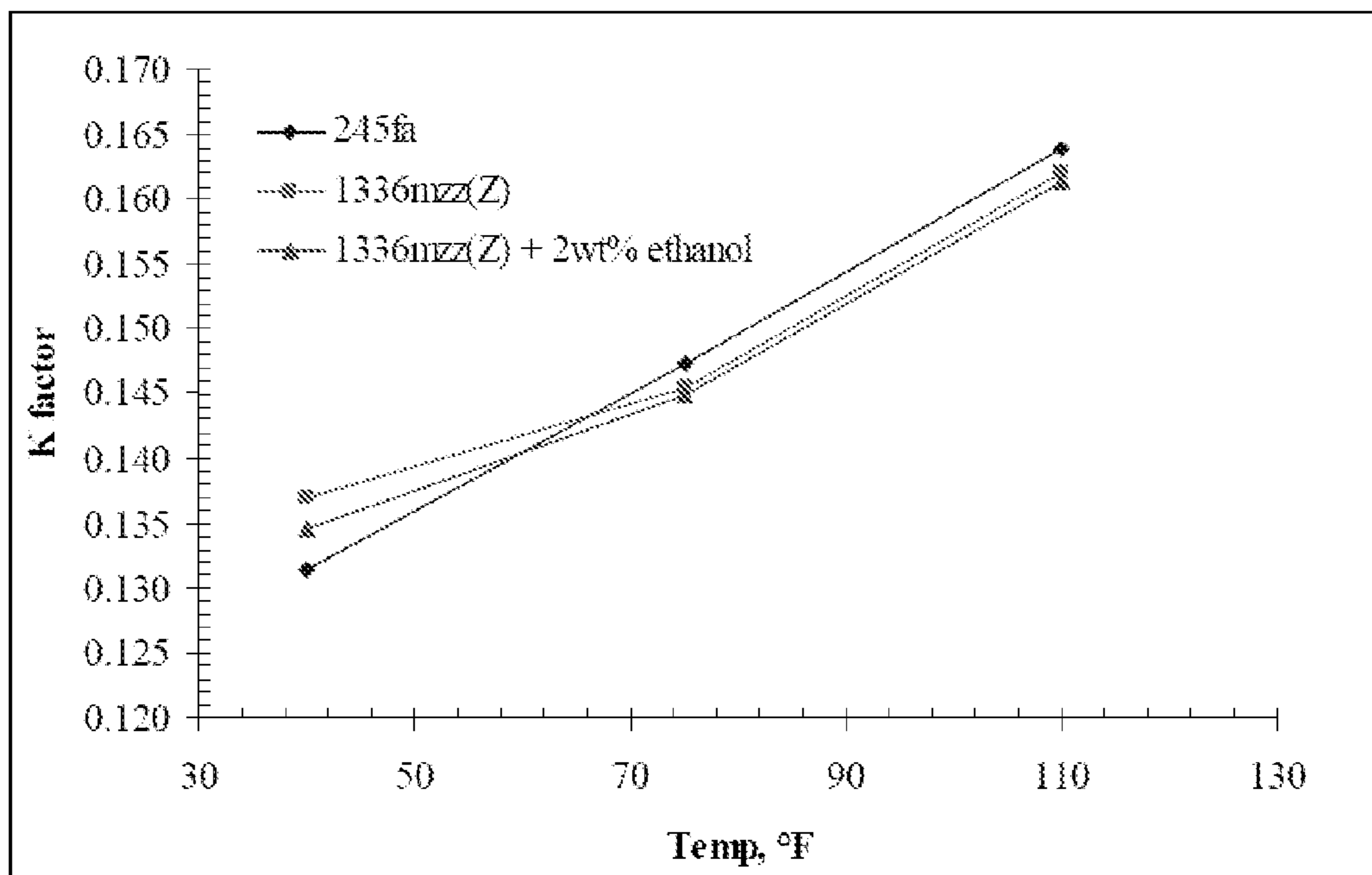
k factors of polyurethane foams
