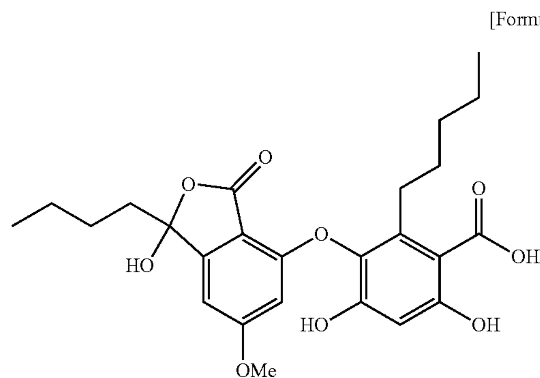
Chemical Formula: C 25 H 30 O 9 Molecular Weight: 474.5
