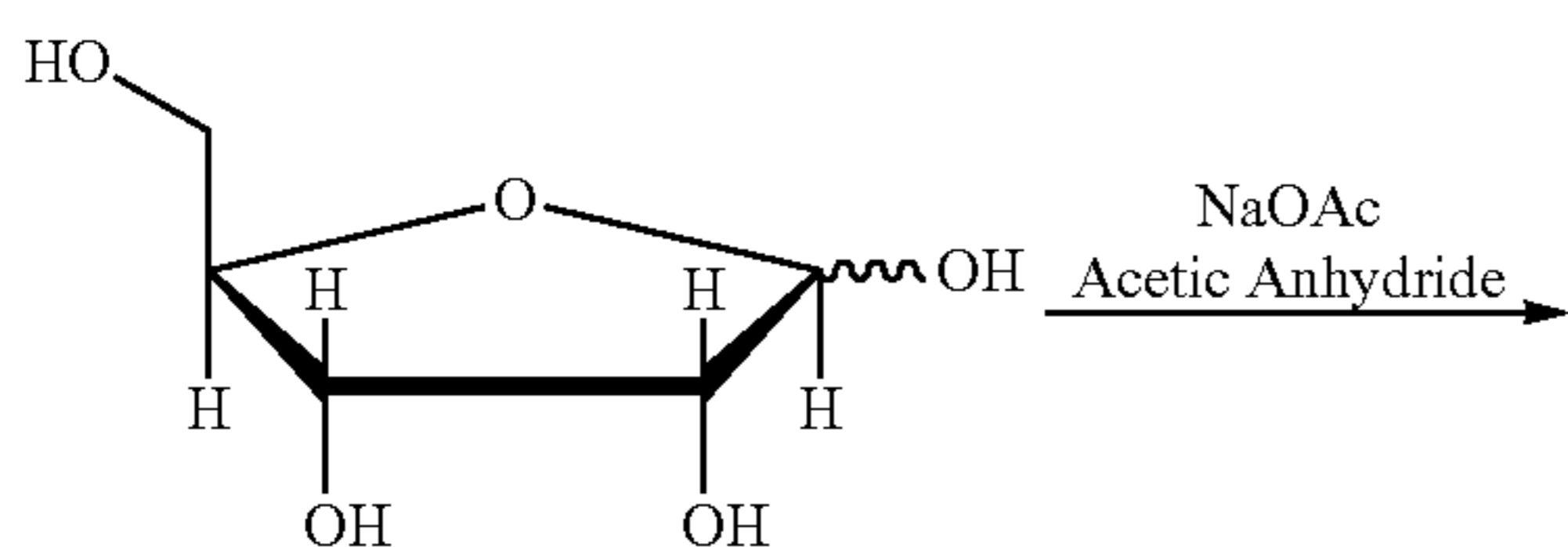
Scheme 1
