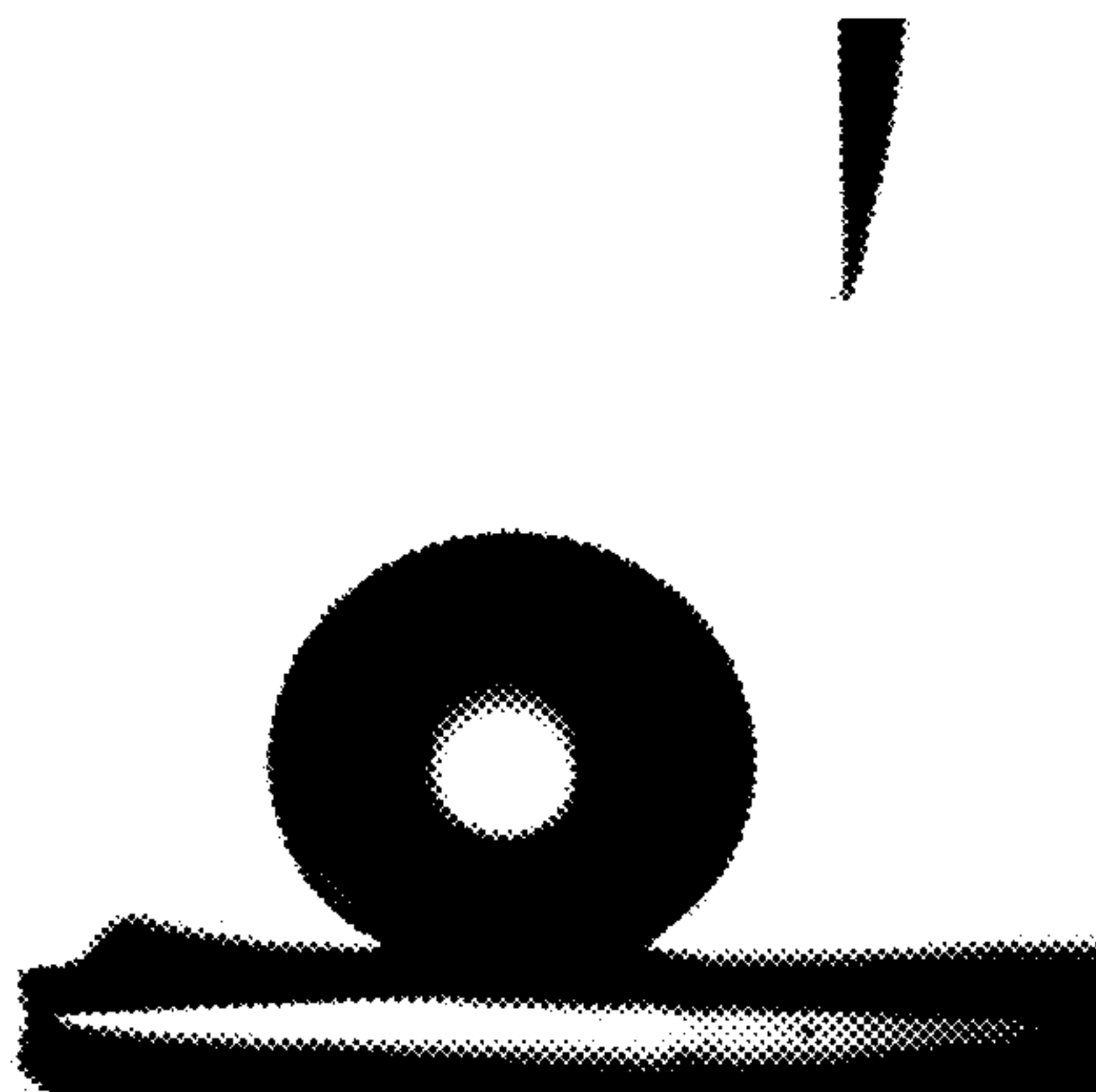
FIG. 36C Ti Textured & Autoclaved ( \theta = 152^\circ )
