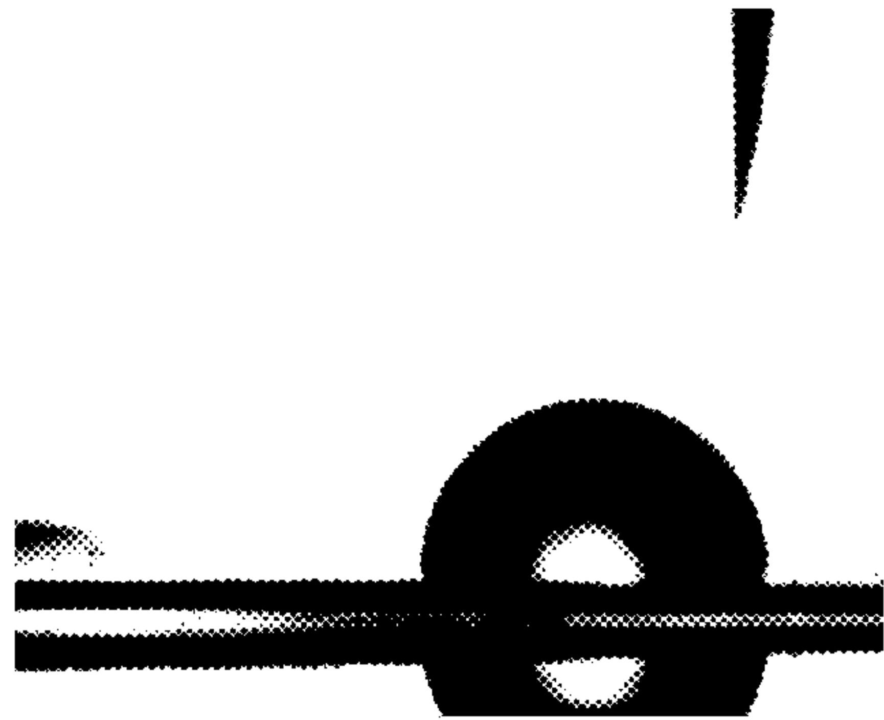
FIG. 36A Ti Control ( \theta = 93^\circ )
