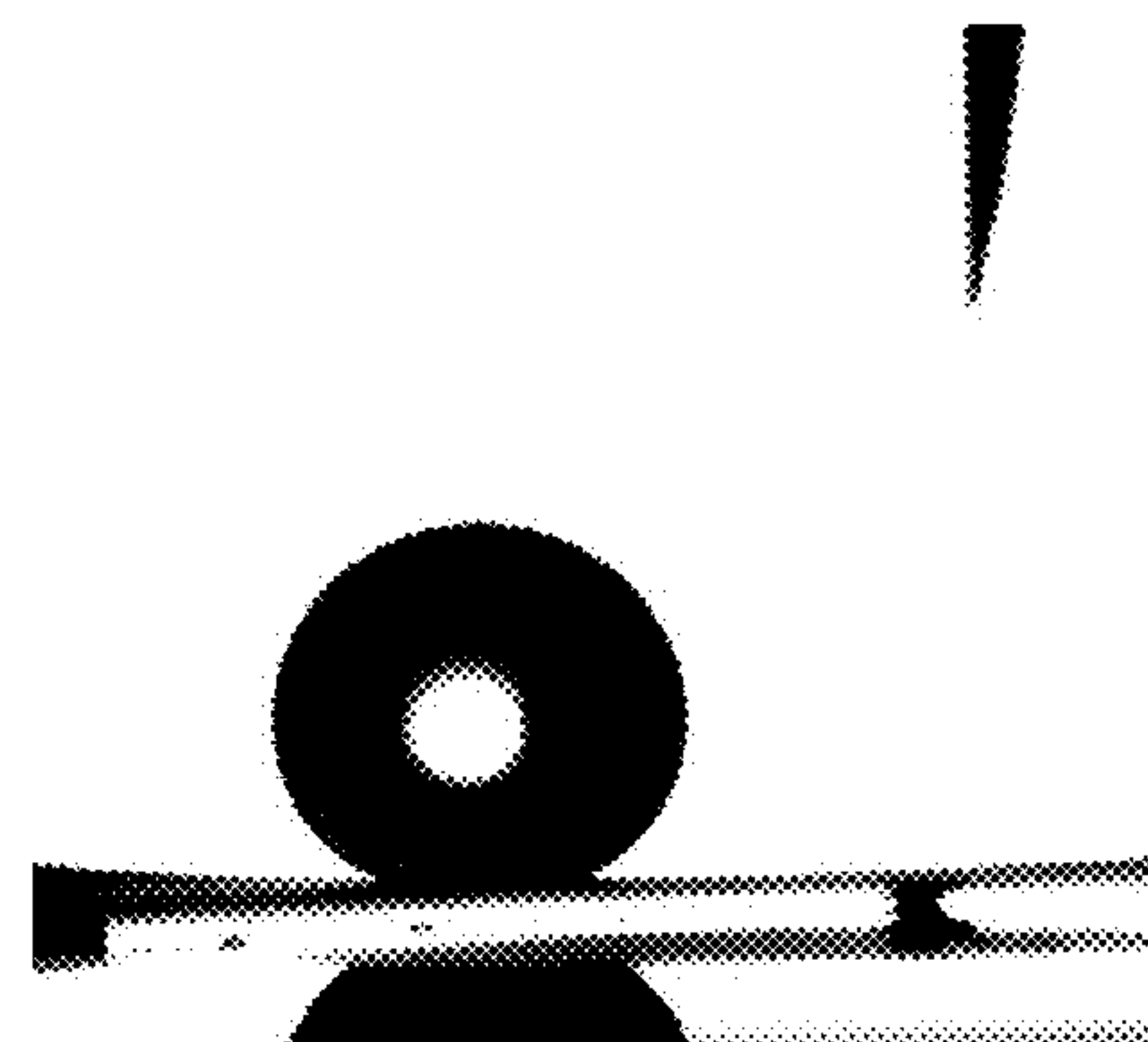
FIG. 36F SS Textured & Autoclaved ( \theta = 152.6^\circ )
