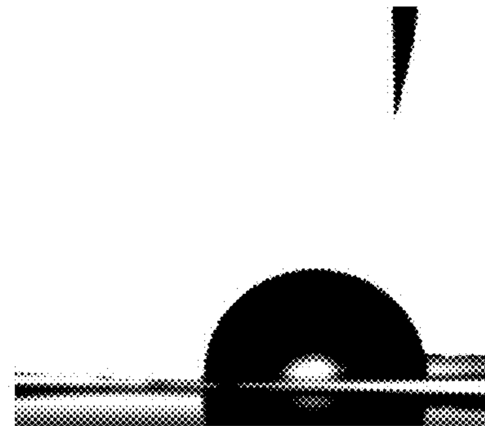
FIG. 36D SS Control ( \theta = 72.5^\circ )
