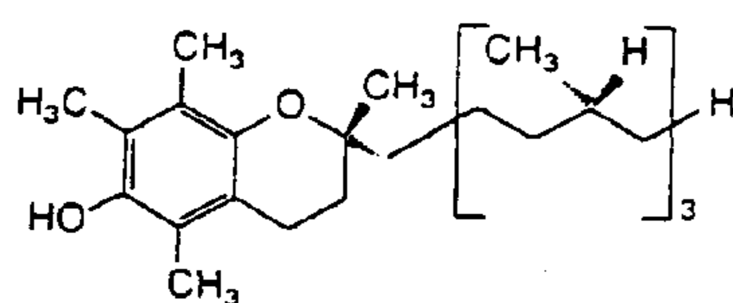
\alpha -Tocopherol (vitamin E)
