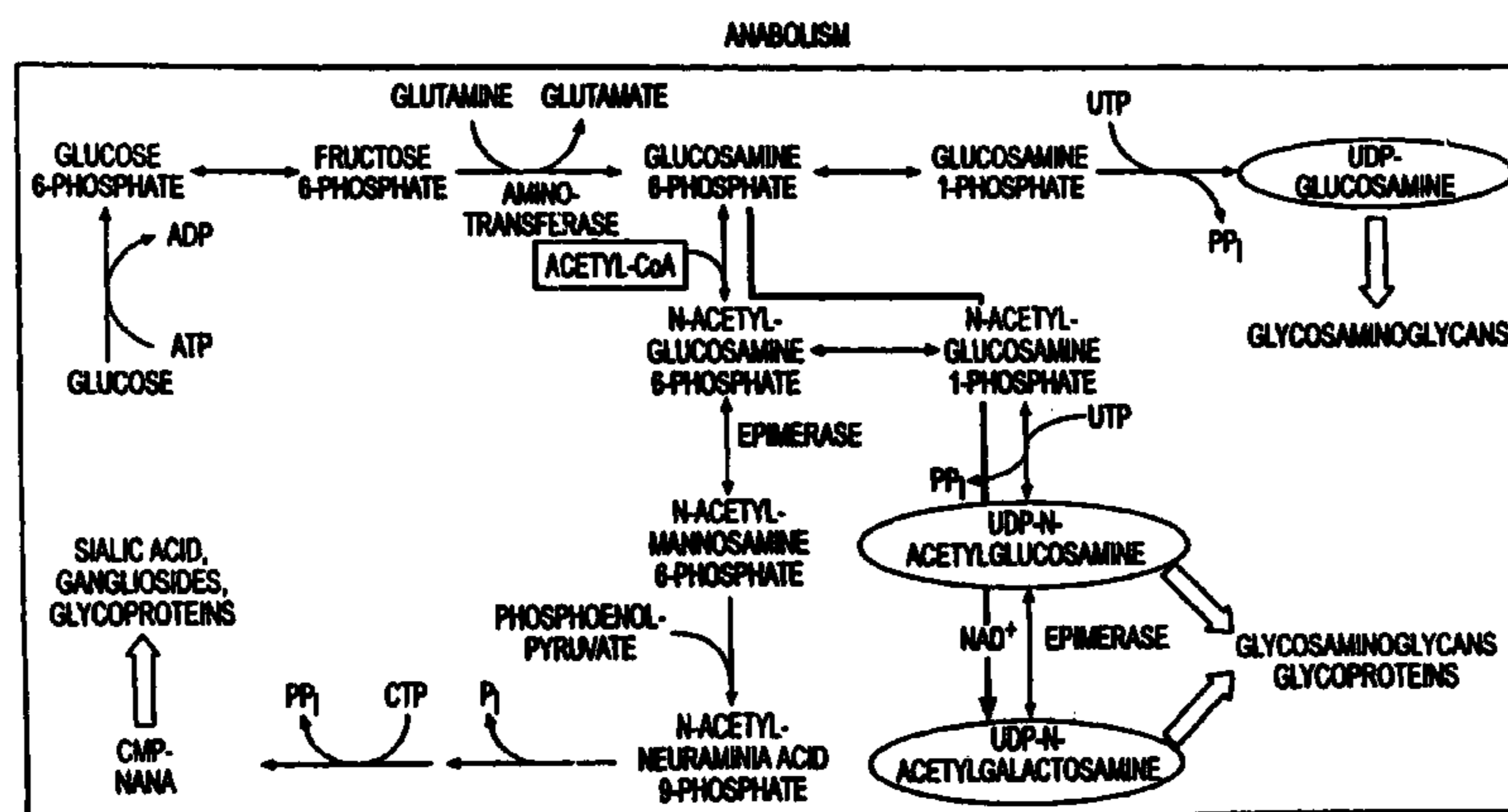
THE SYNTHESIS OF GLYCOSAMINOGLYCANS FROM GLUCOSAMINE
