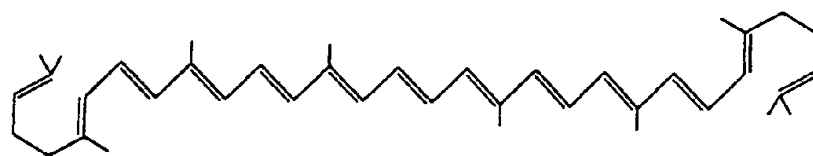
Lycopene
