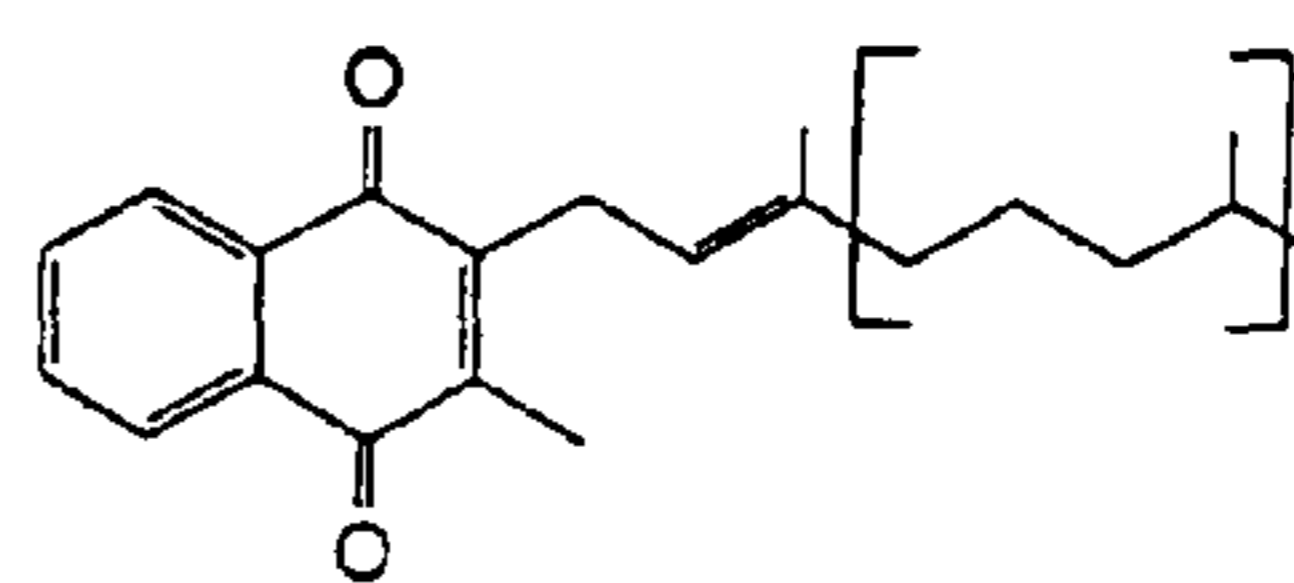
Phylloquinone
