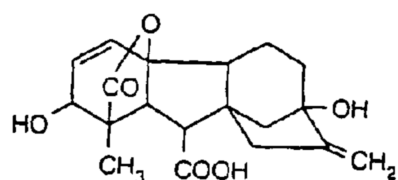
Gibberellic acid
