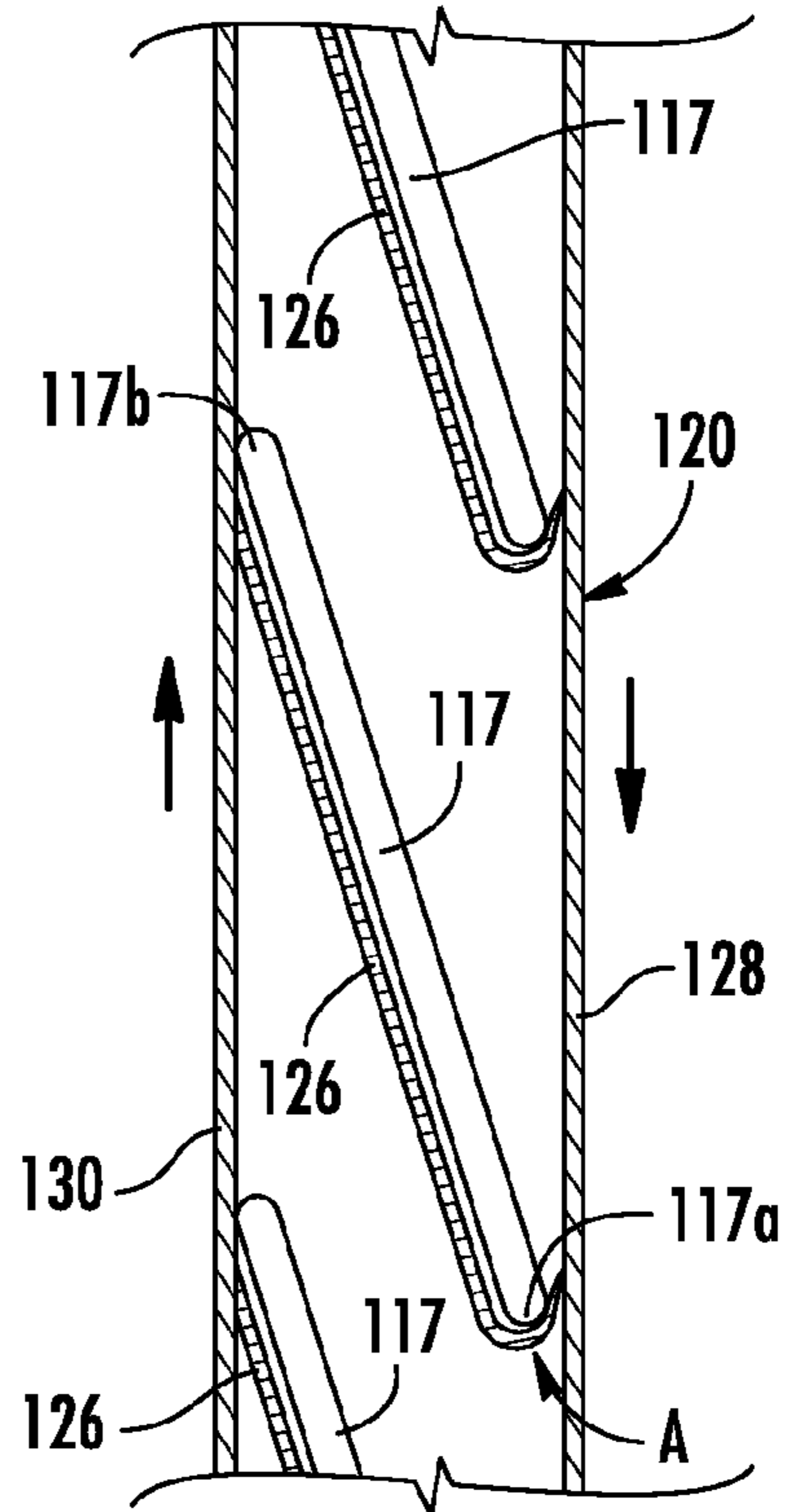
FIG. 3 PRIOR ART
