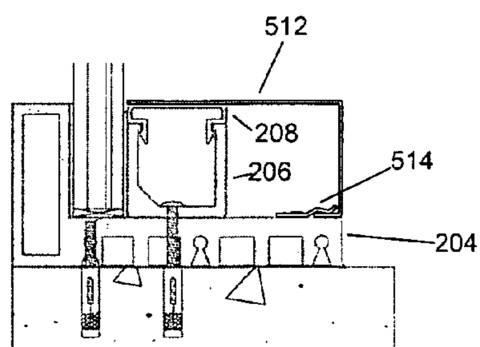
HEAD/SILL/JAMB WITH AESTHETIC COVER CAP
