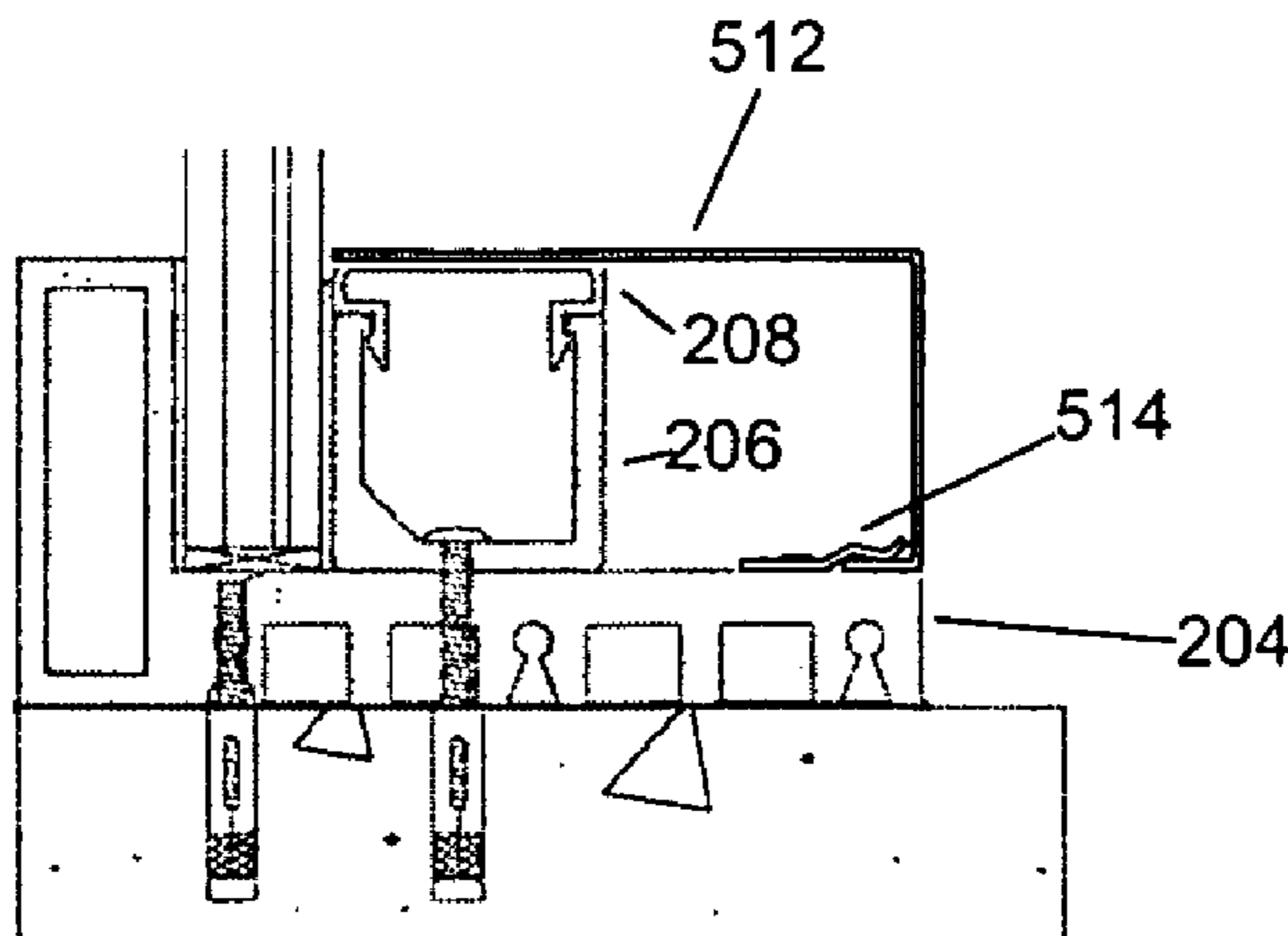
HEAD/SILL/JAMB WITH AESTHETIC COVER CAP
