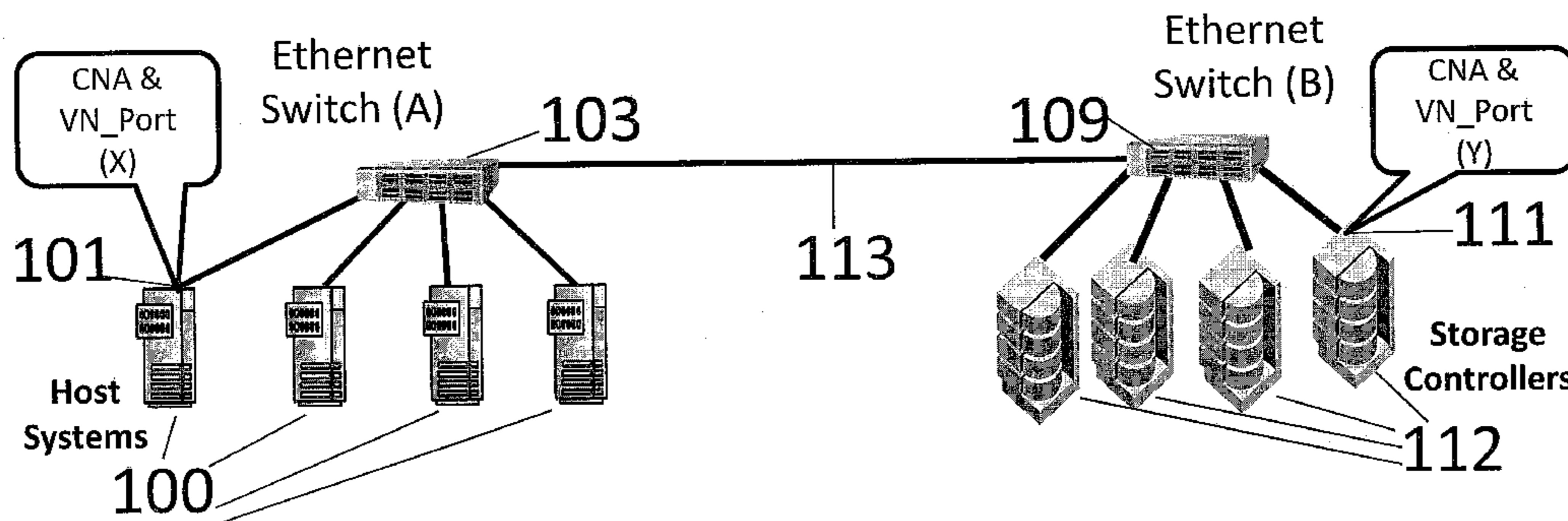
A Direct Mode FCoE Network Configuration Example
