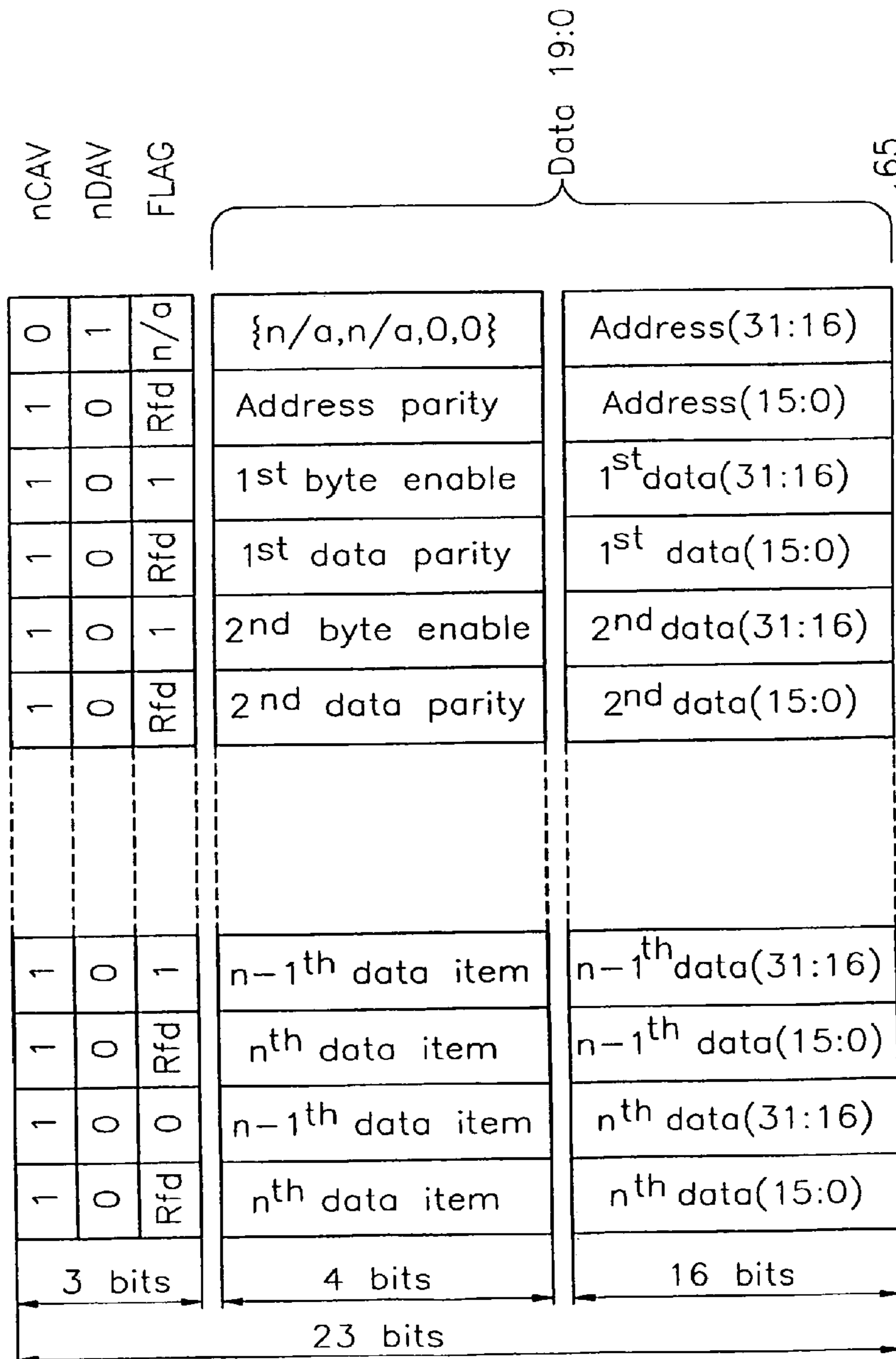
Example implementation showing 1960-style burst local bus protocol carried on HP-GLINK physical layer
