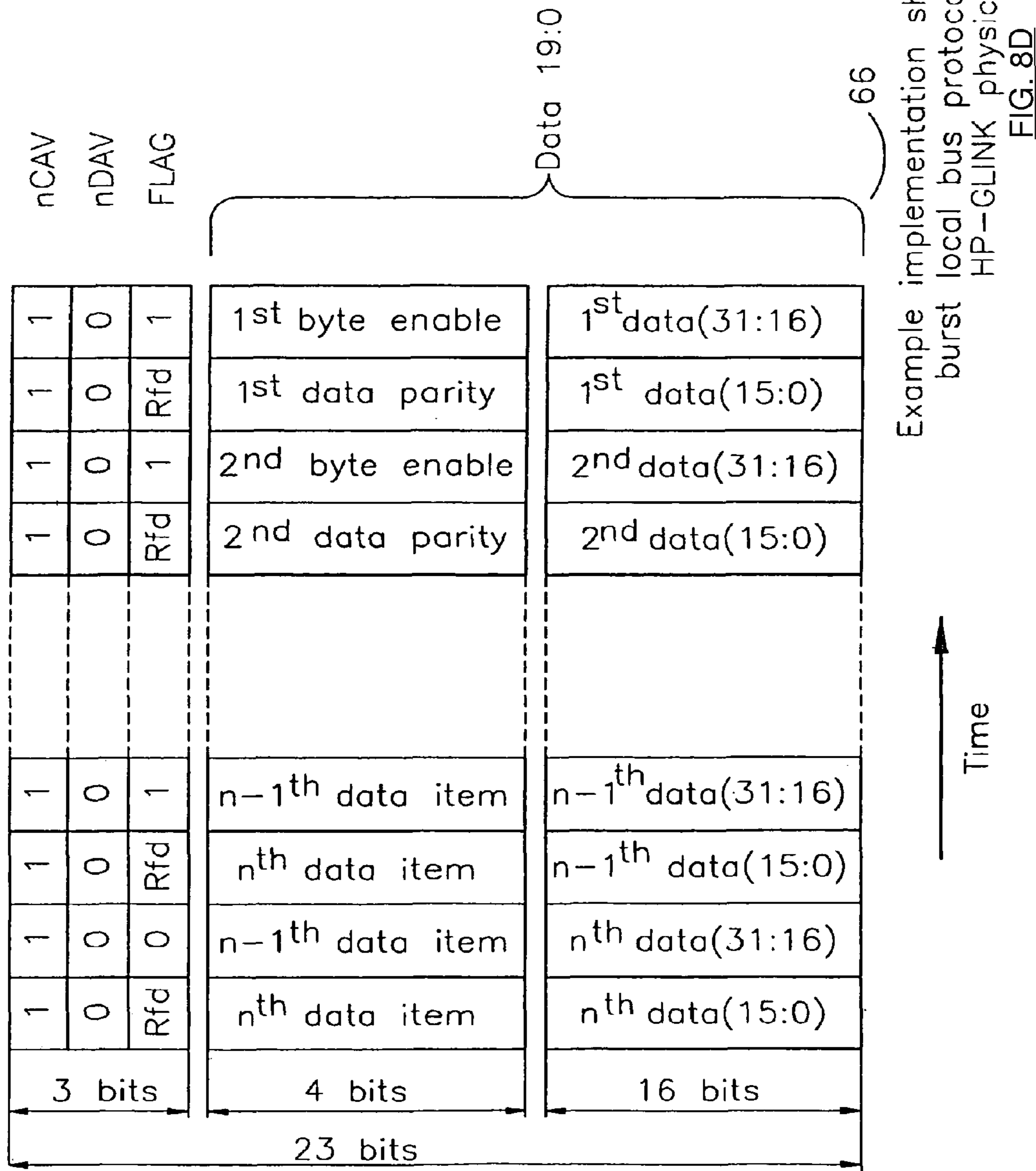
Current protocol embodiment(Read data burst returning)
