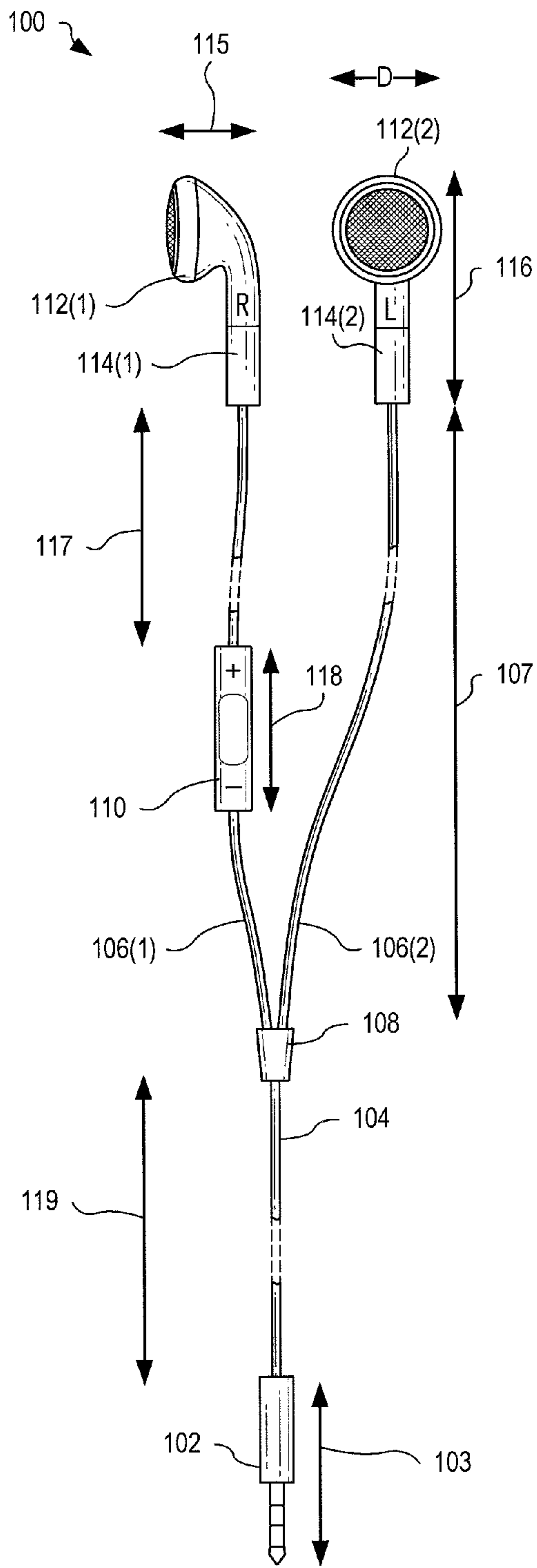
FIG. 1 PRIOR ART
