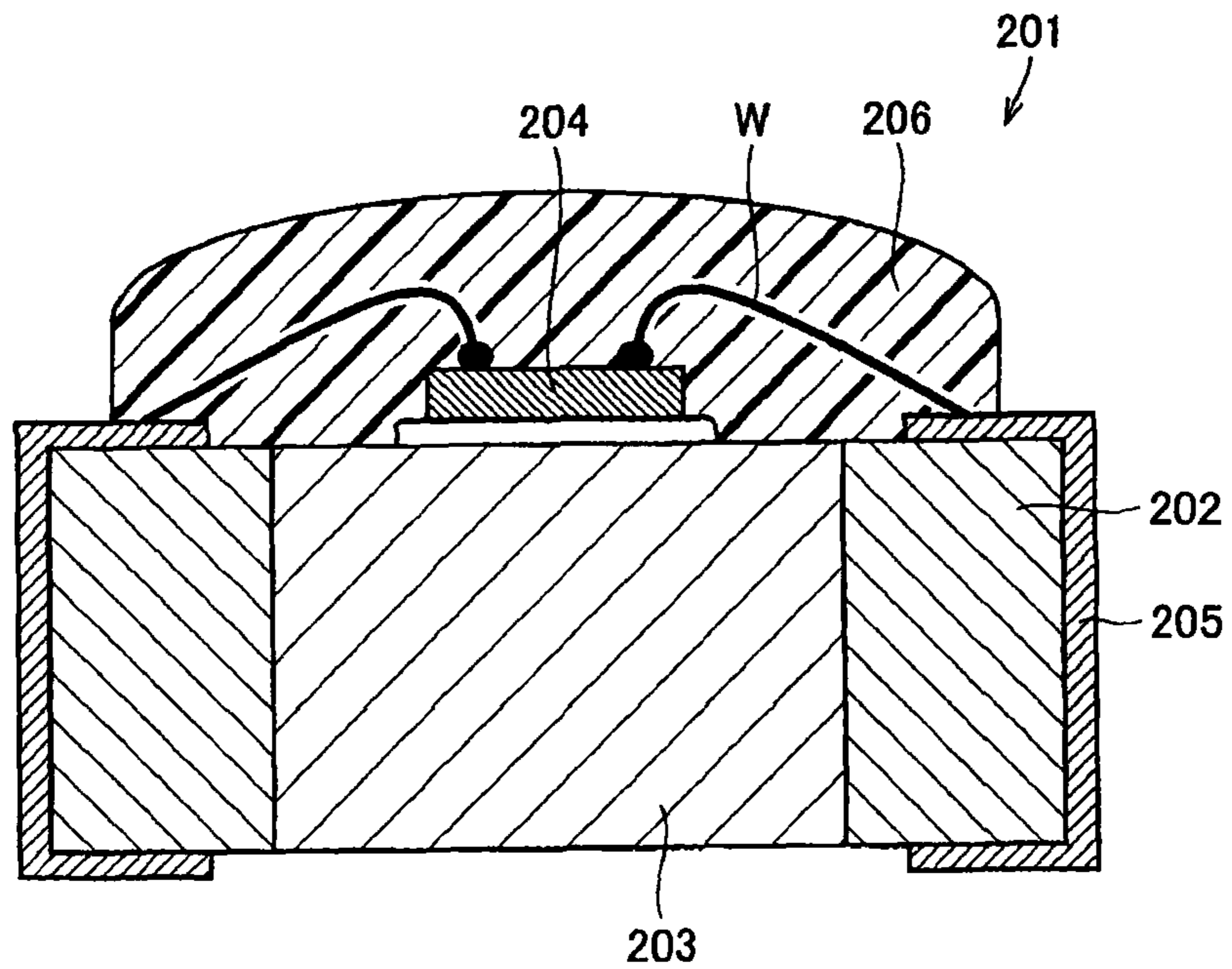
FIG.15 PRIOR ART
