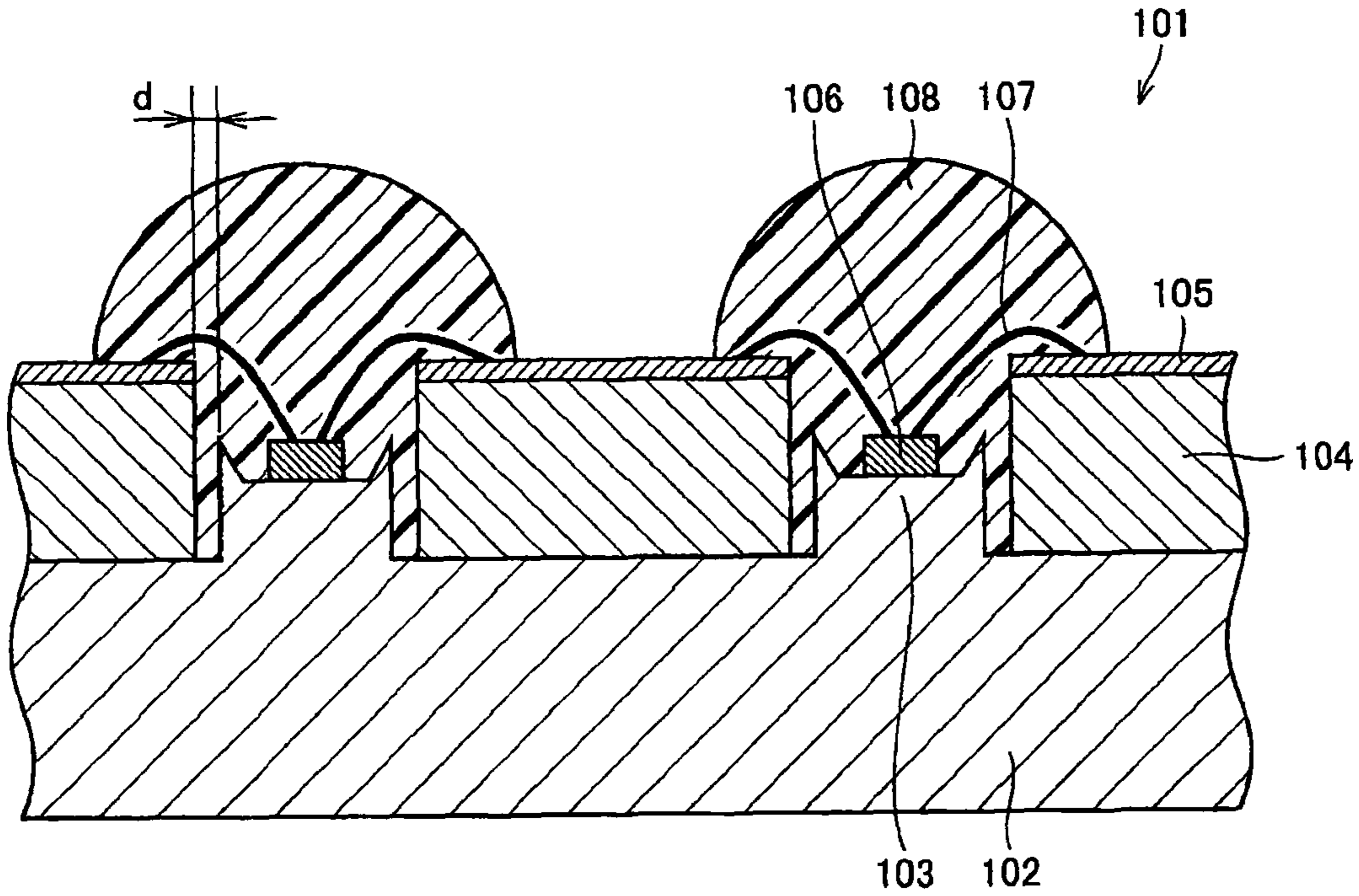
FIG.14 PRIOR ART
