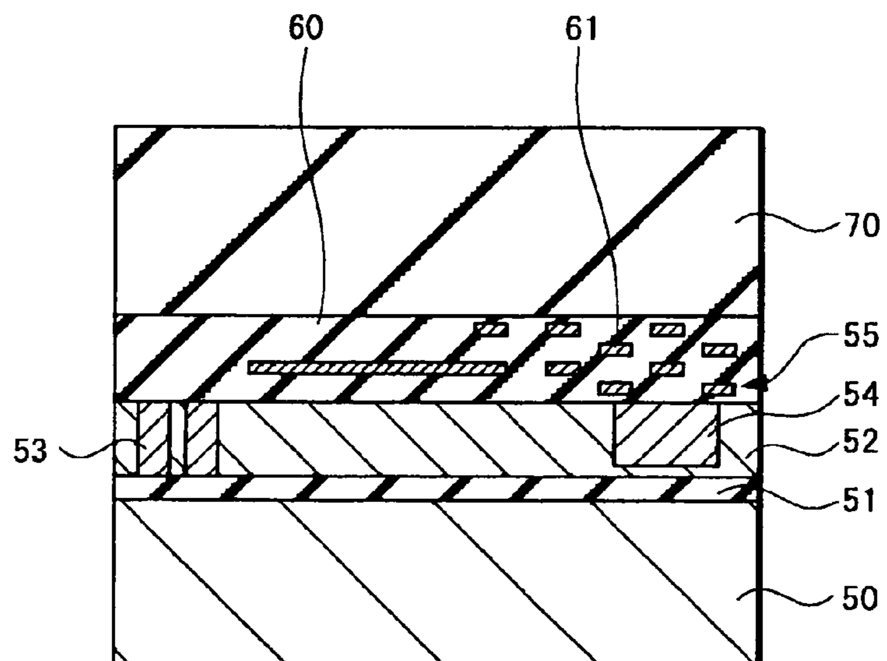
FIG. 4C (RELATED ART)
