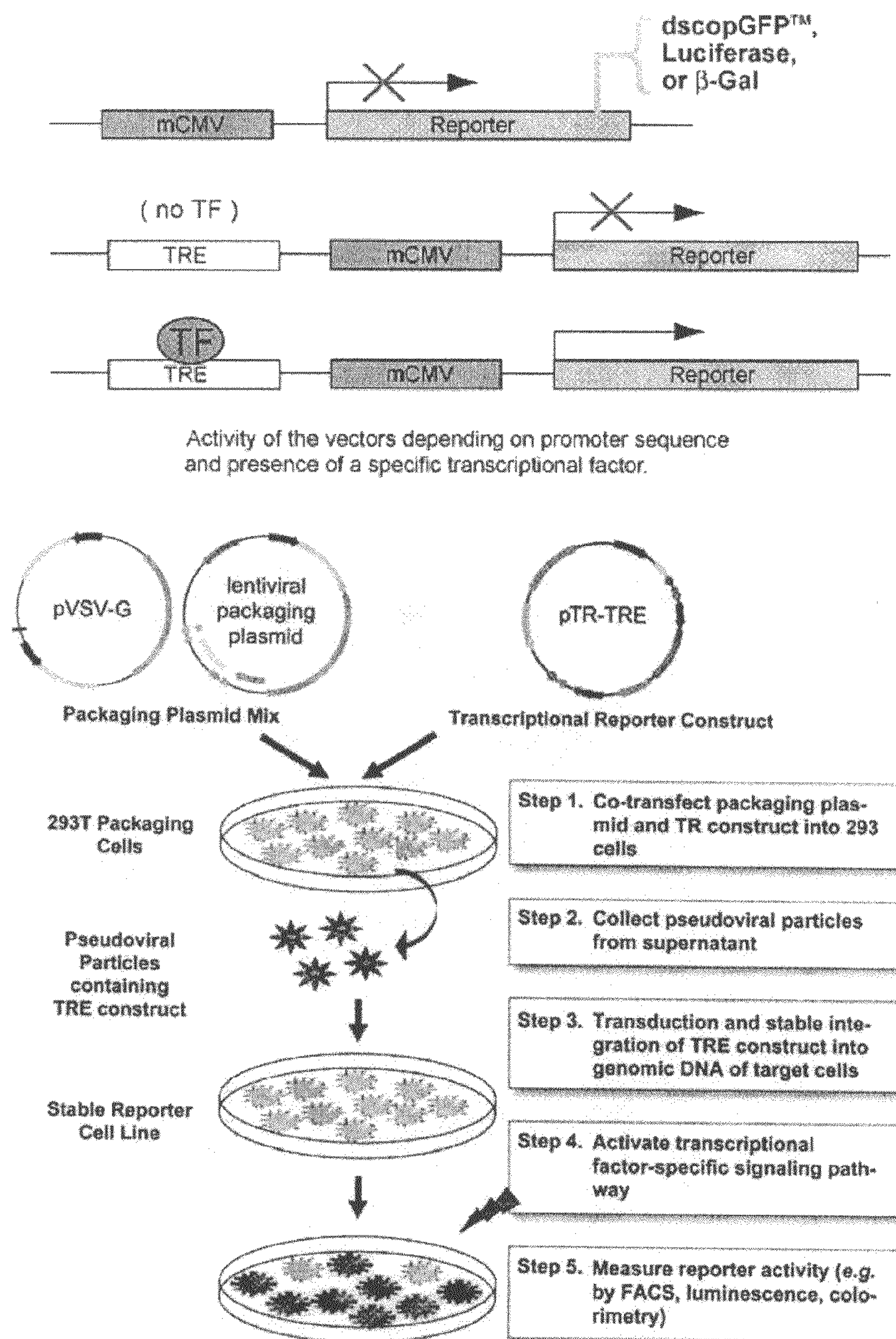
Schematic presentation of the packaging procedure for pTR constructs and making of stable cell lines.
