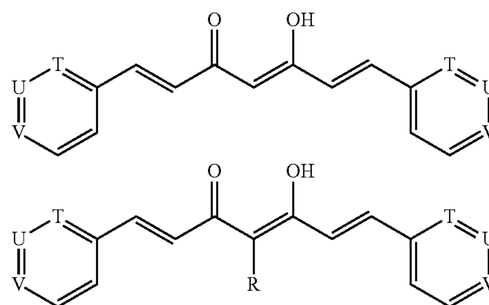
Pyridine aryl ring analogs.
