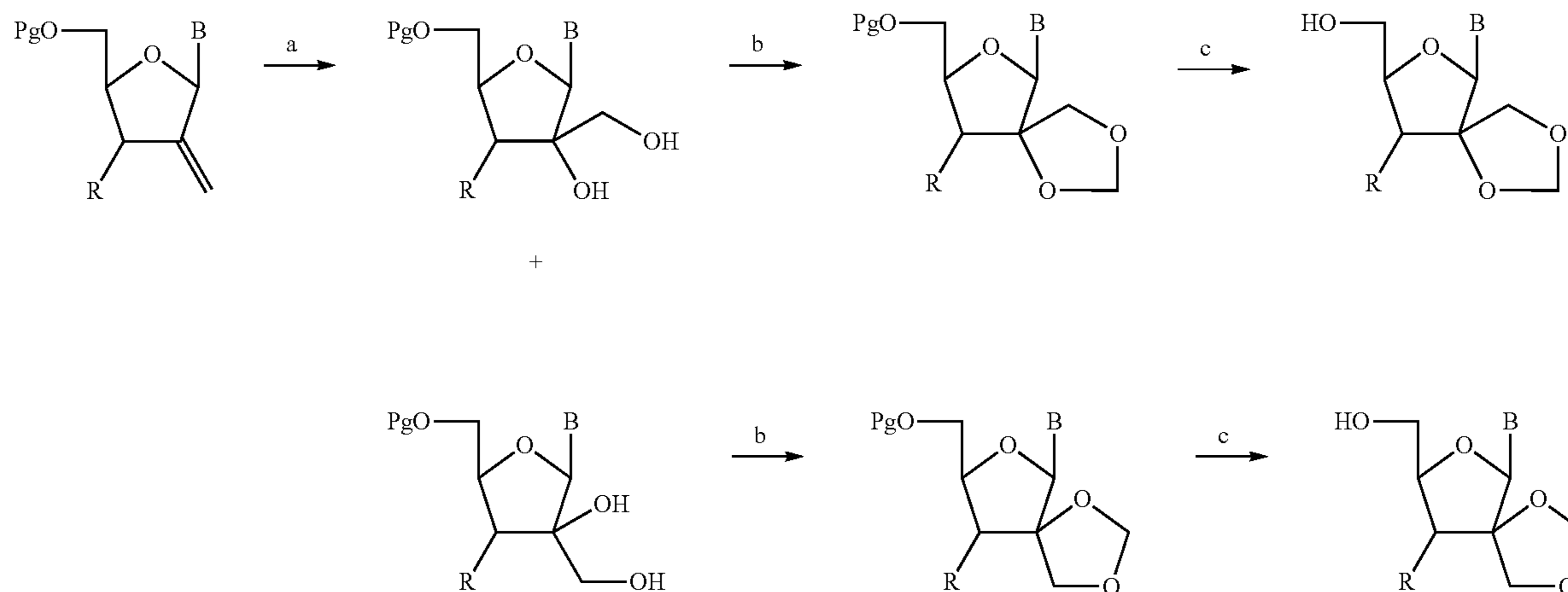
Scheme 3. General Procedure for preparing 2'-spiro-(1,3-dioxolan-5-yl) Nucleosides
