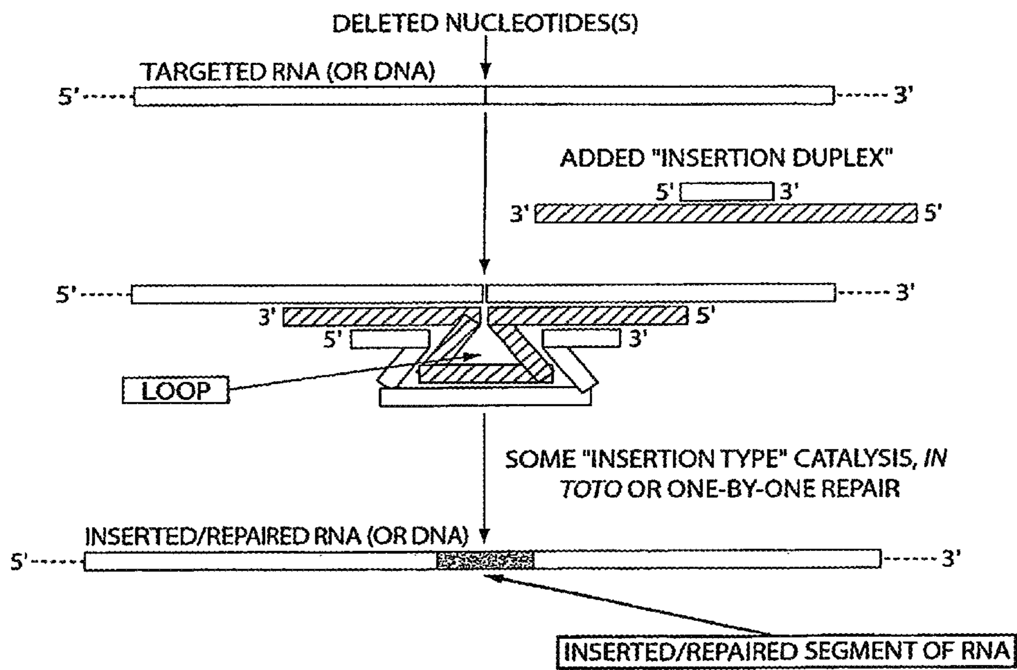
SCHEME 5
