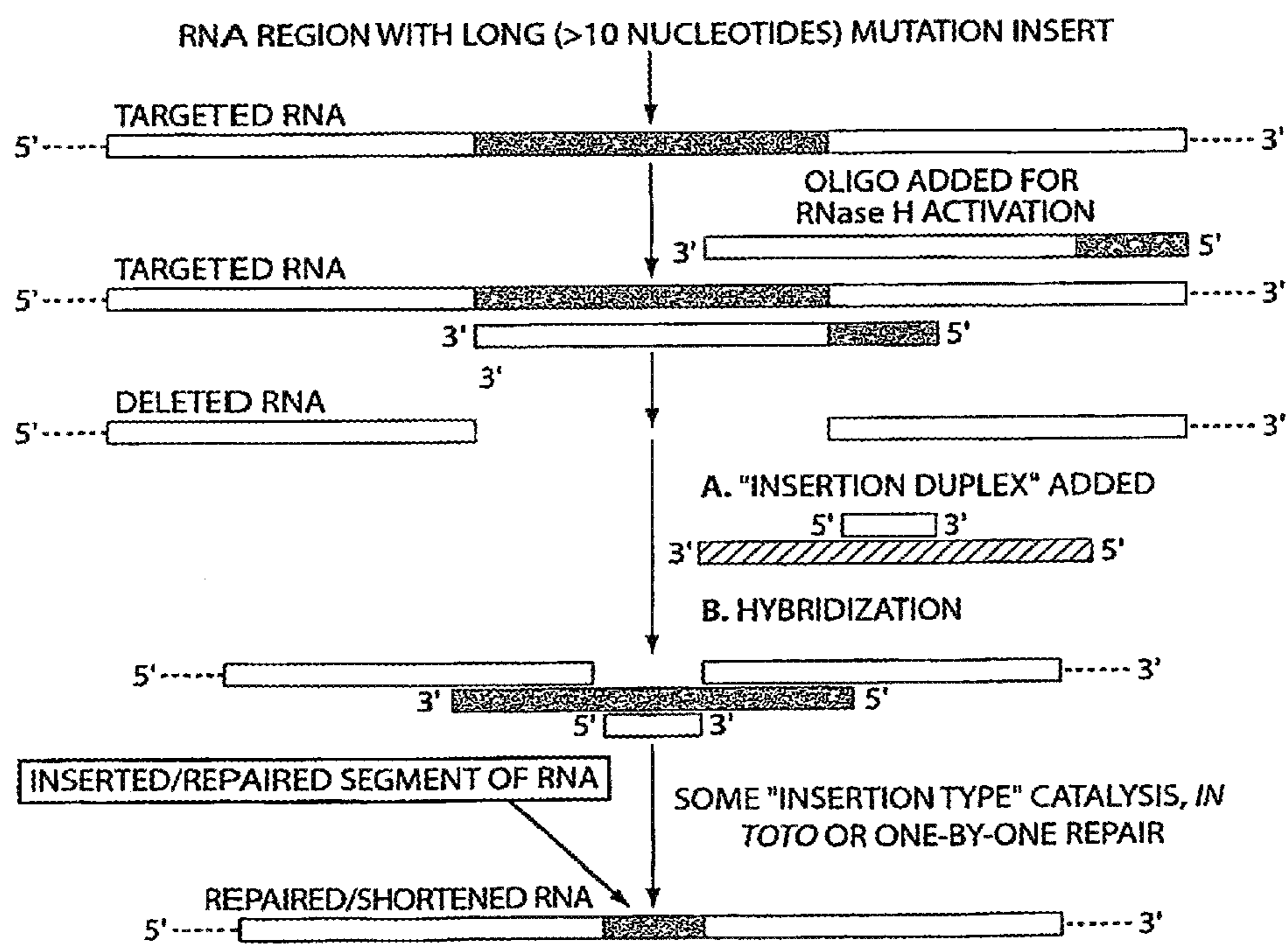
SCHEME 6
