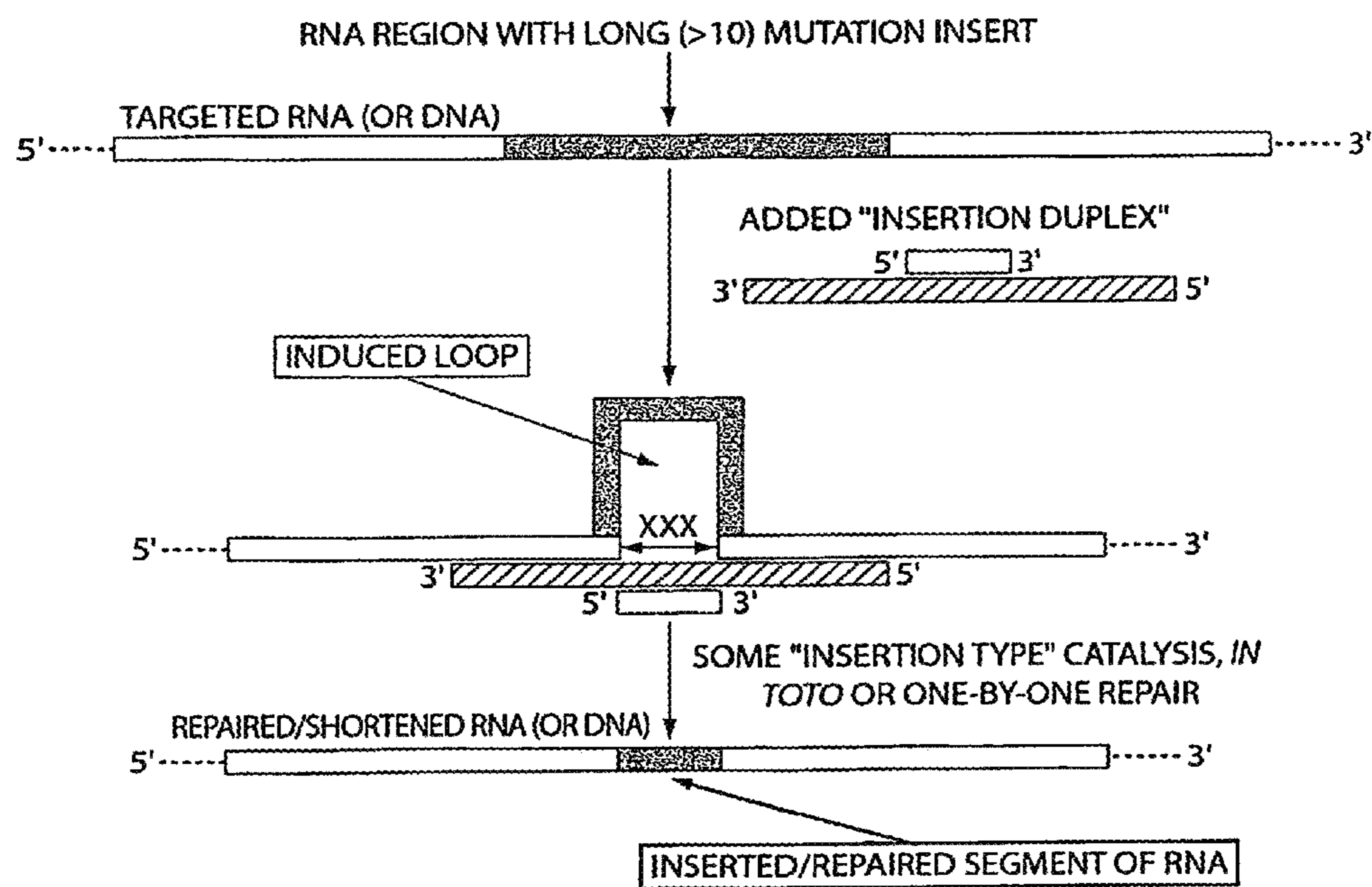
SCHEME 7
