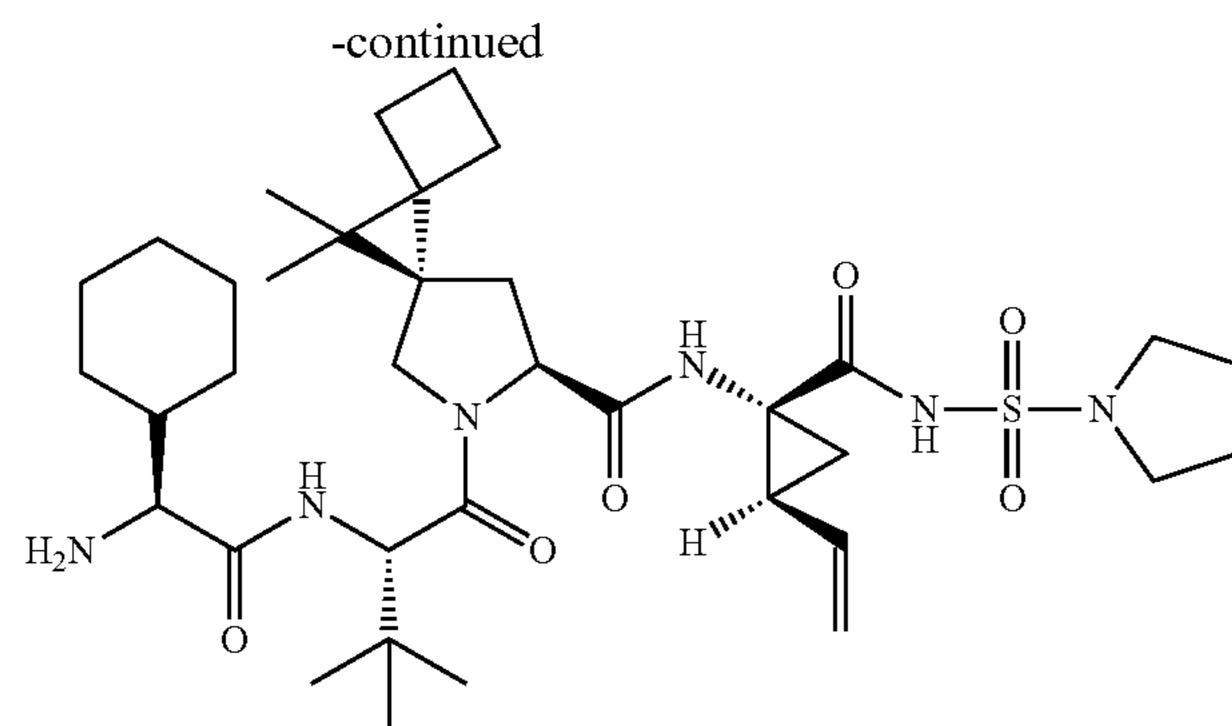
Intermediate I
