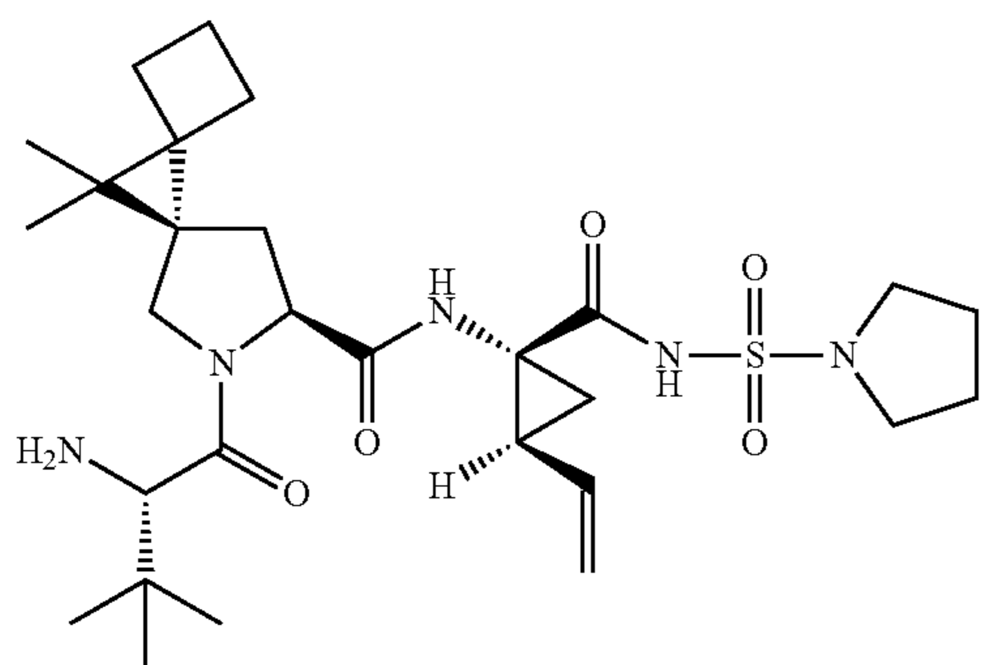
Compound 1g
