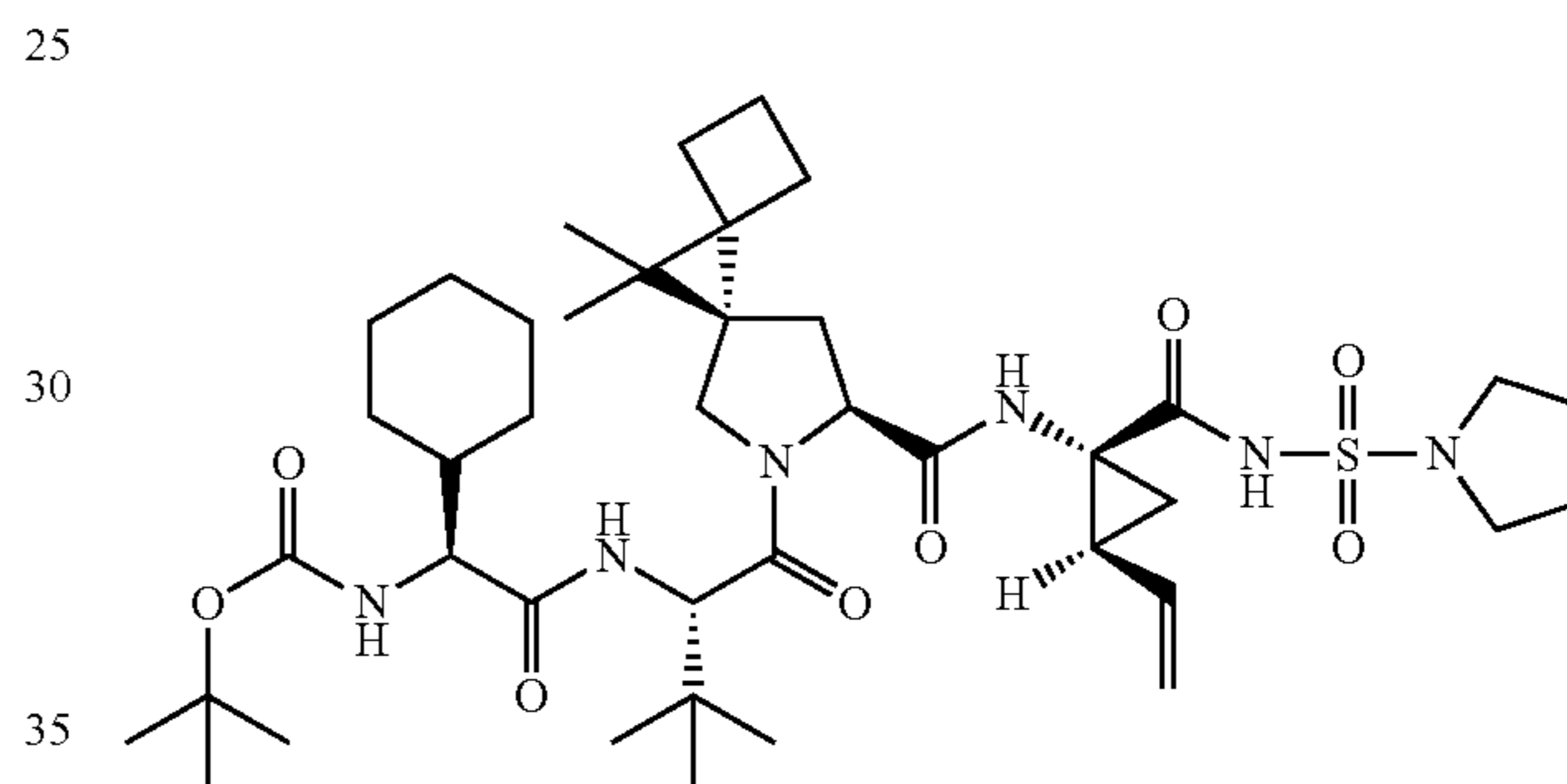
Compound 1h
