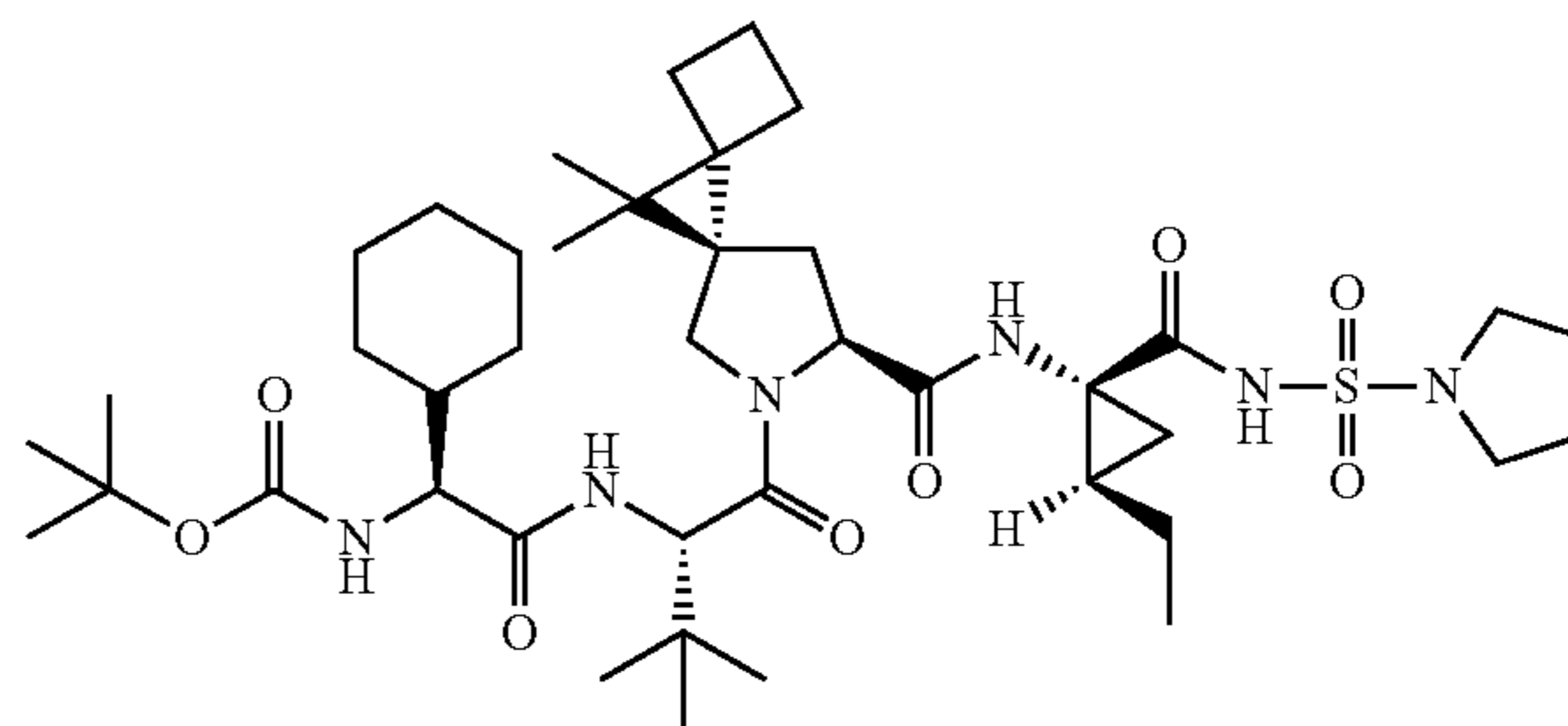
Compound 2g
