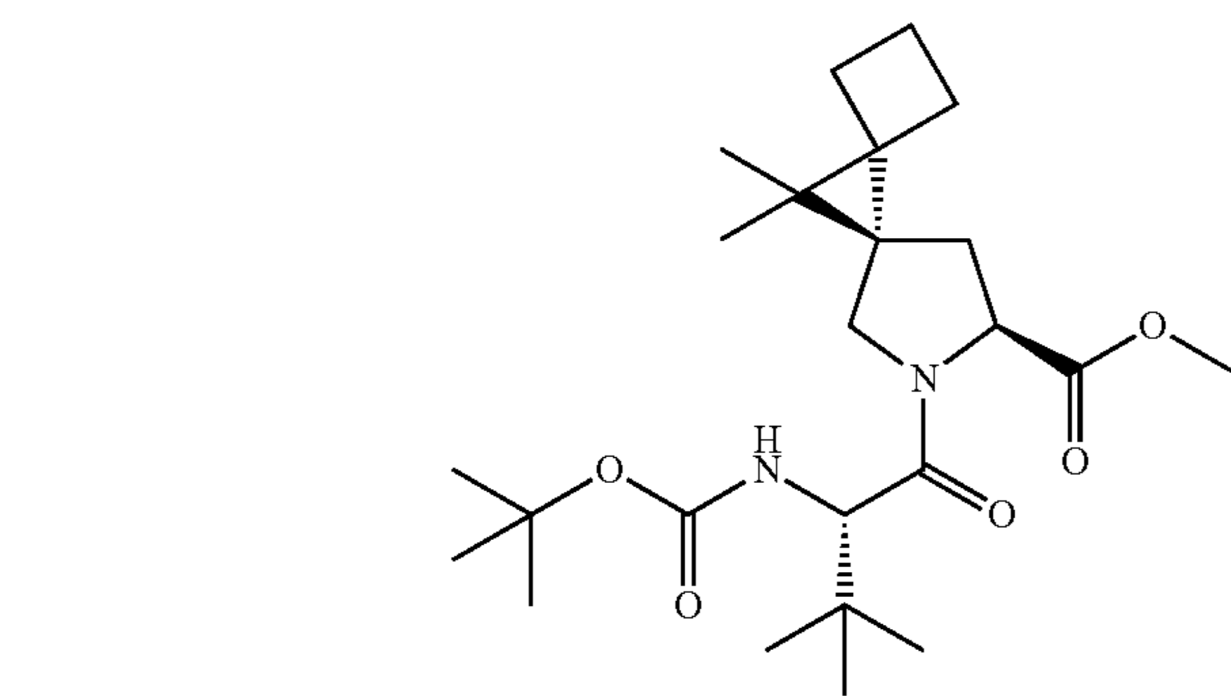
Compound 2c
