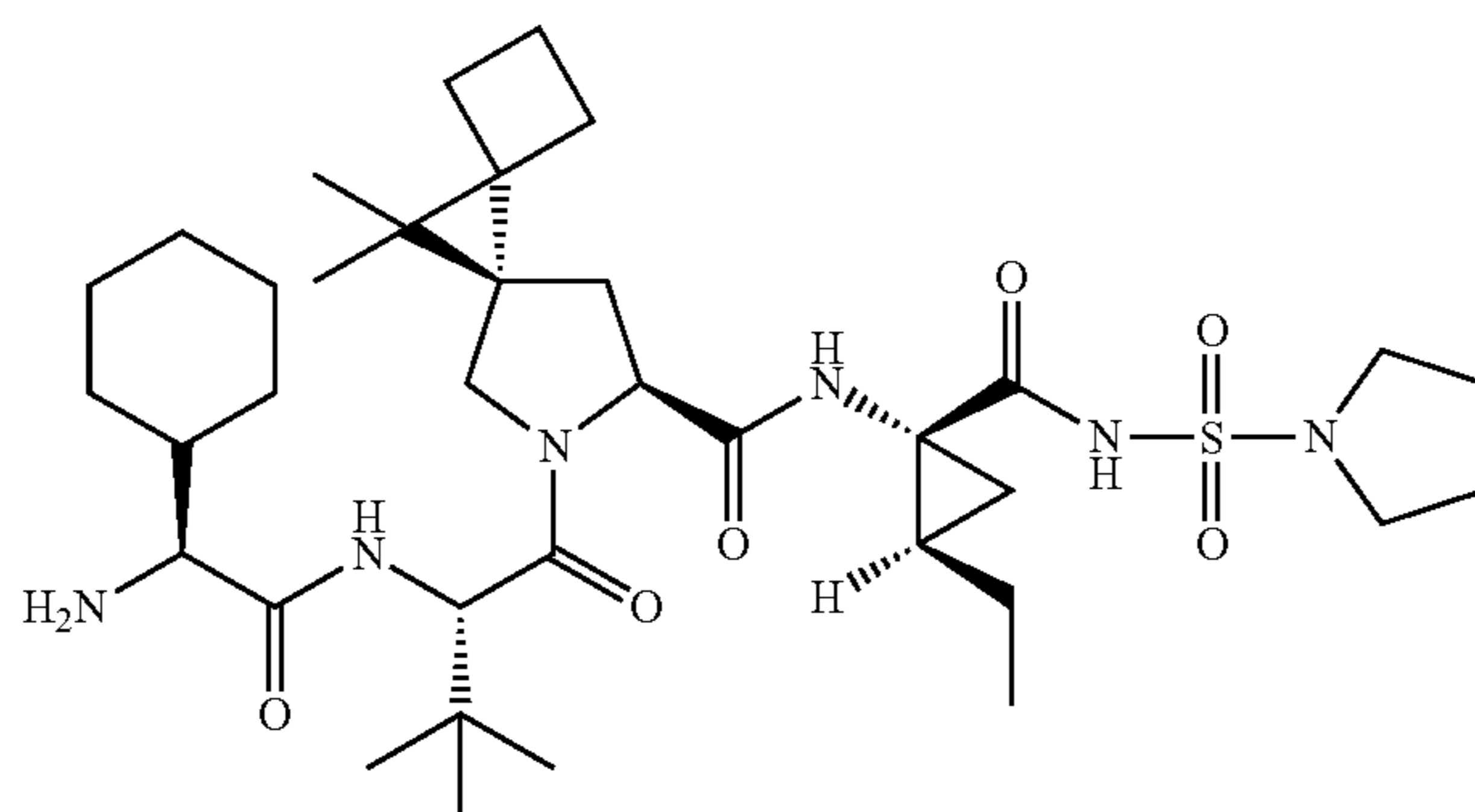
Intermediate II
