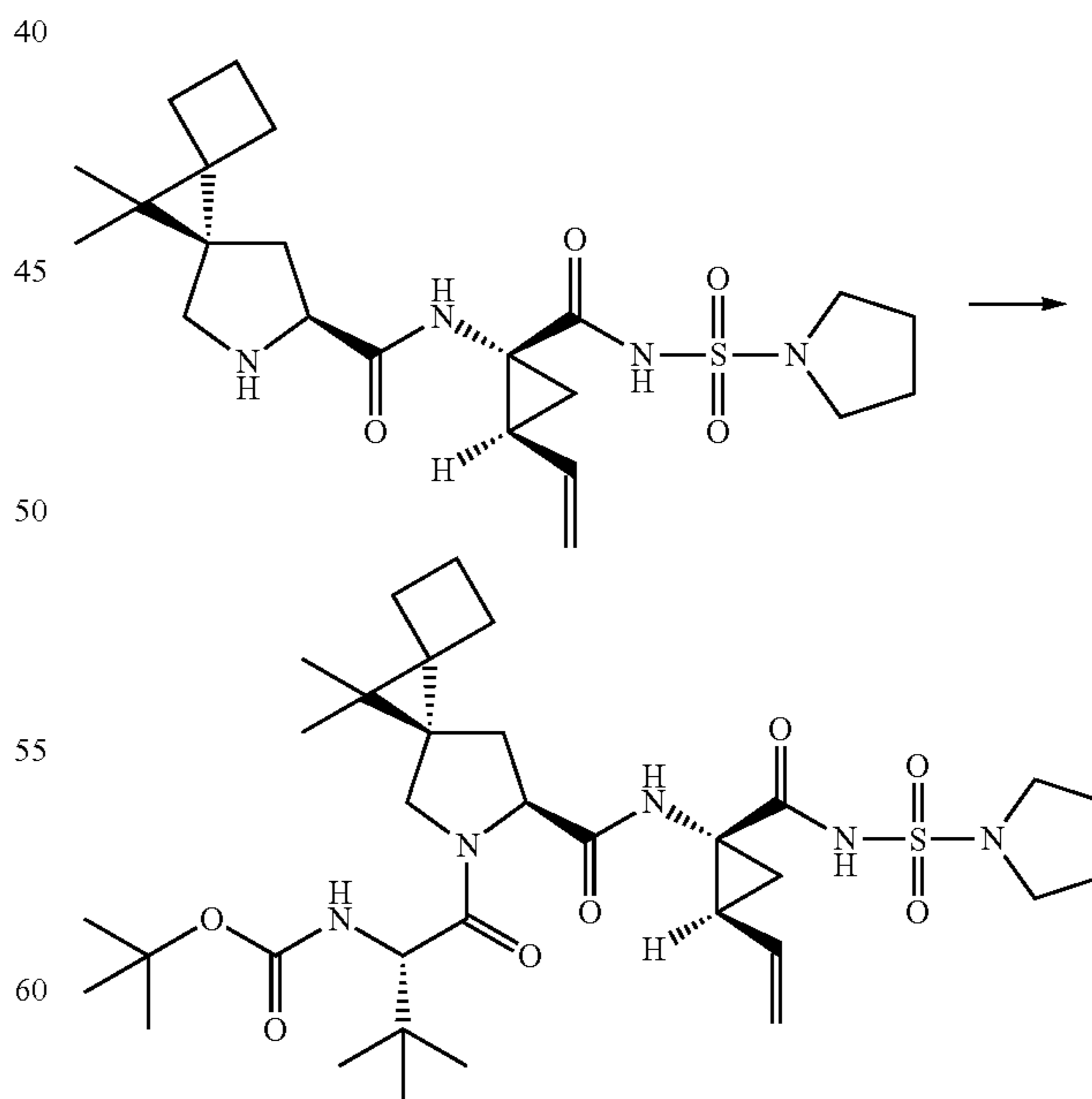
Compound 1f
