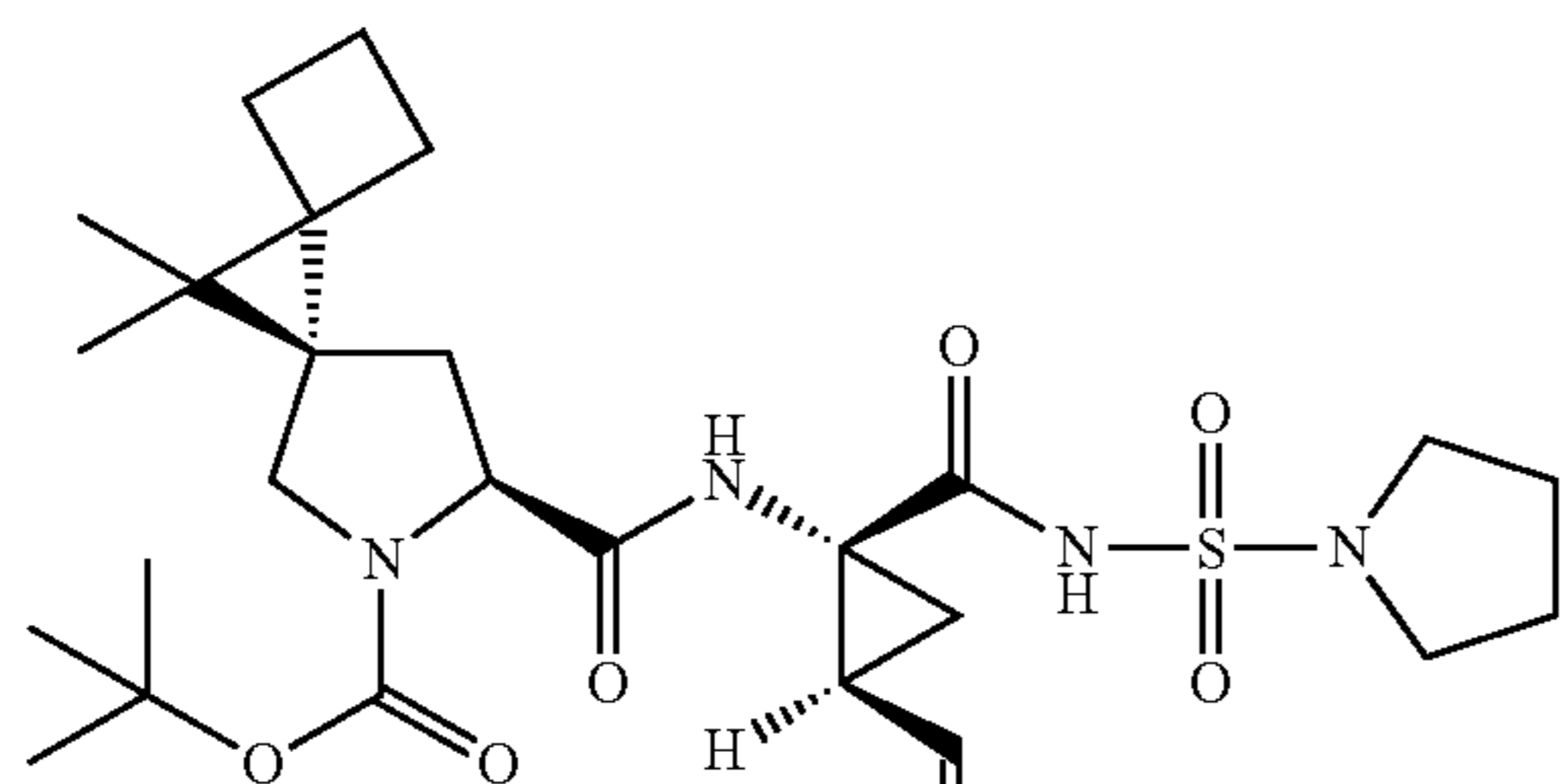
Compound 1d
