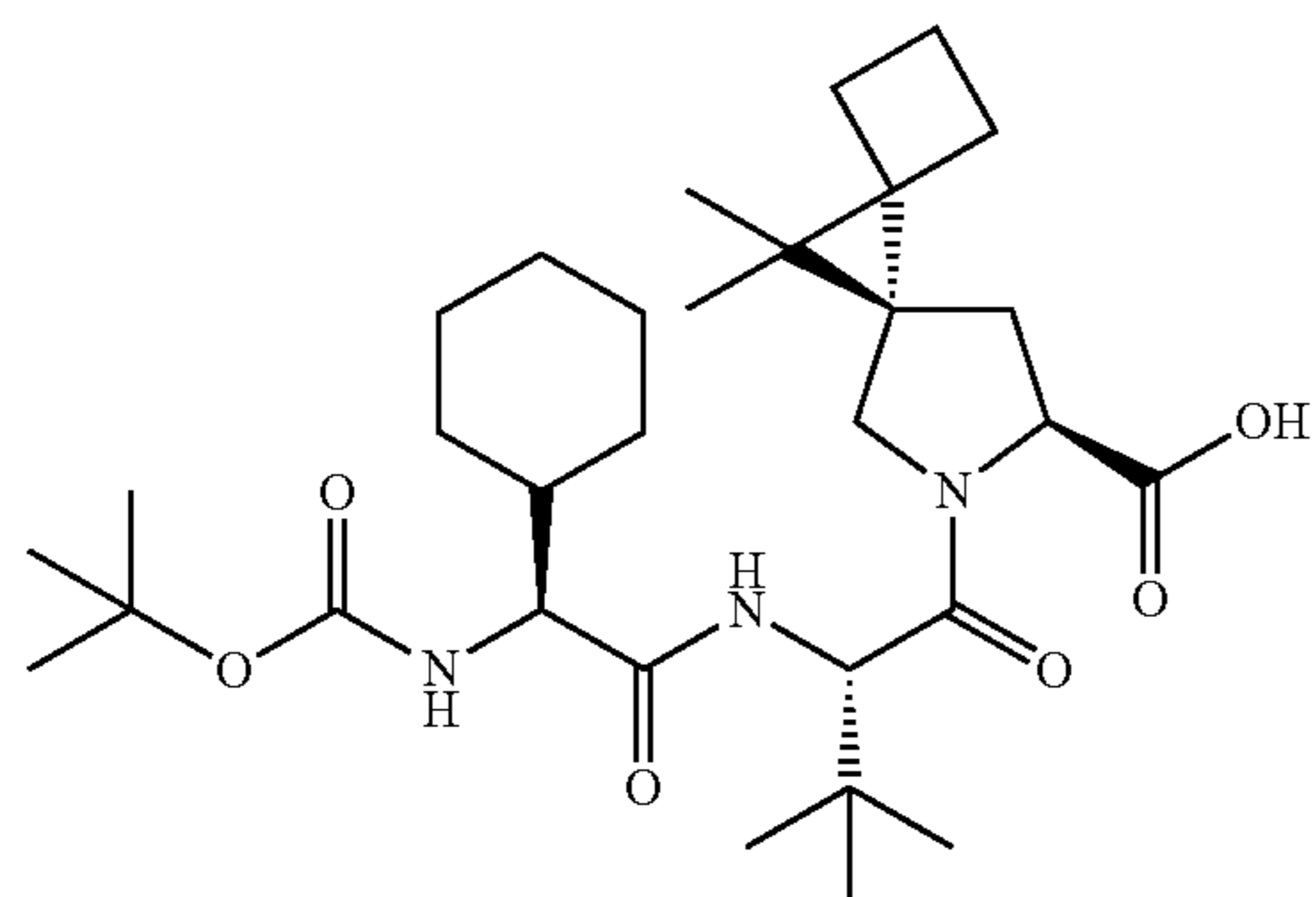
Compound 2f
