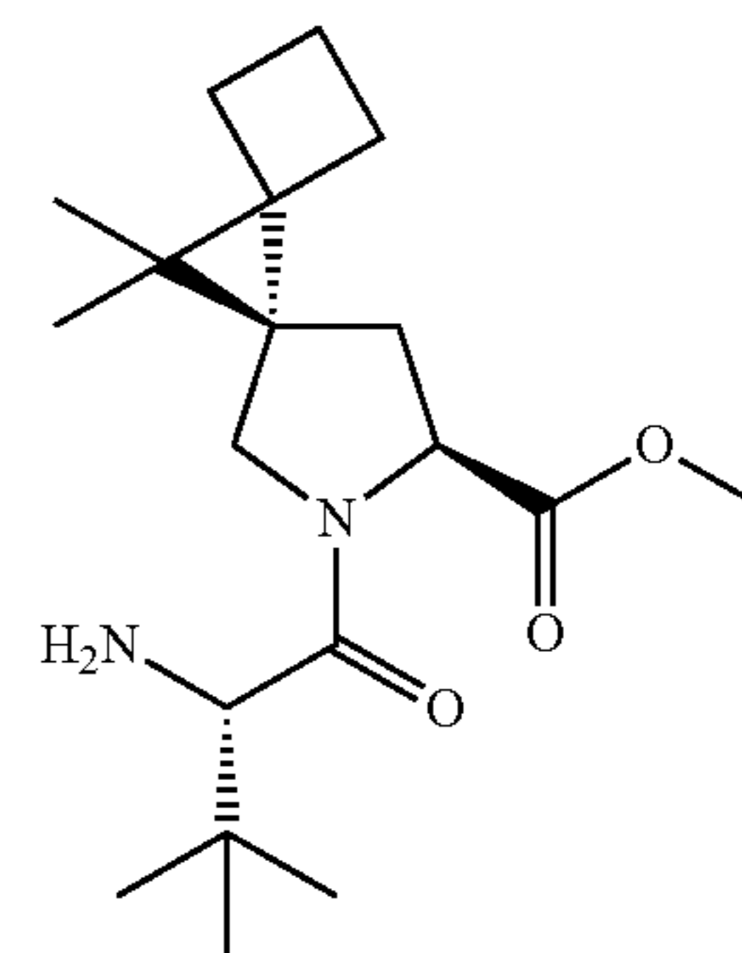
Compound 2d
