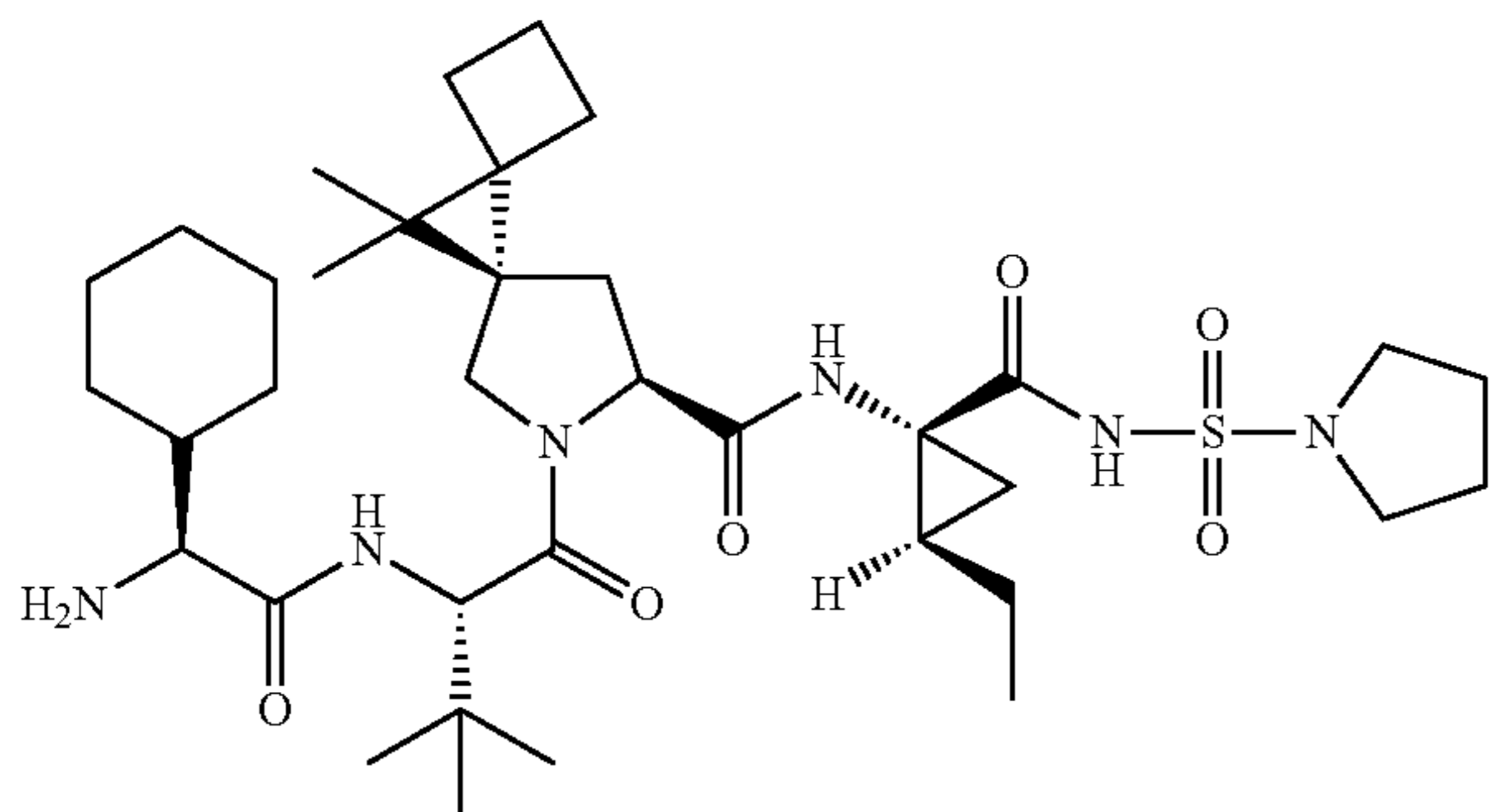
Intermediate II
