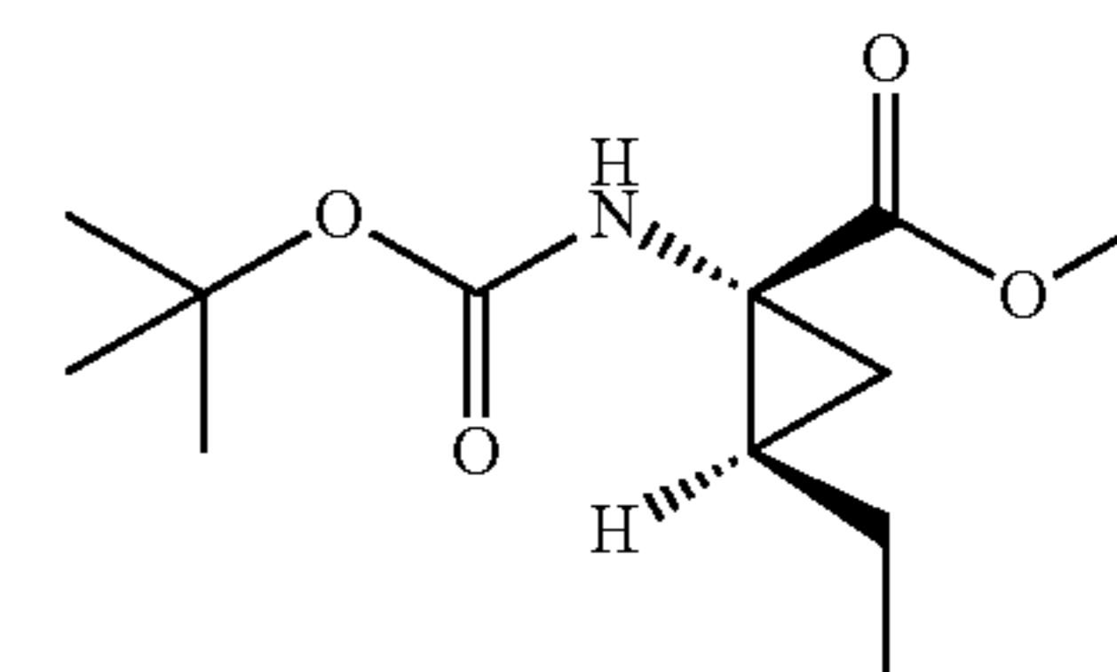
Compound 3a
