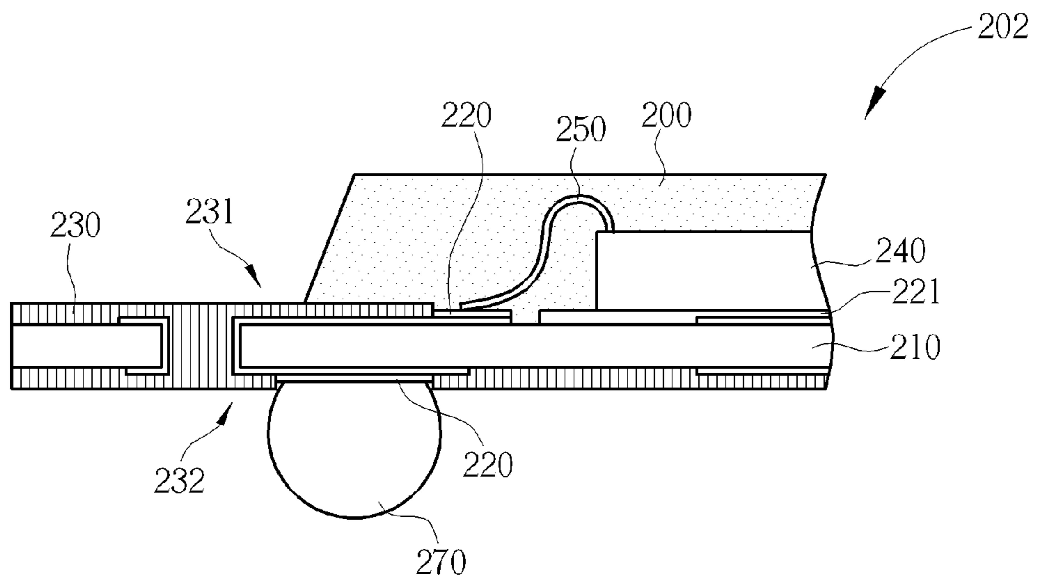
FIG. 6 PRIOR ART
