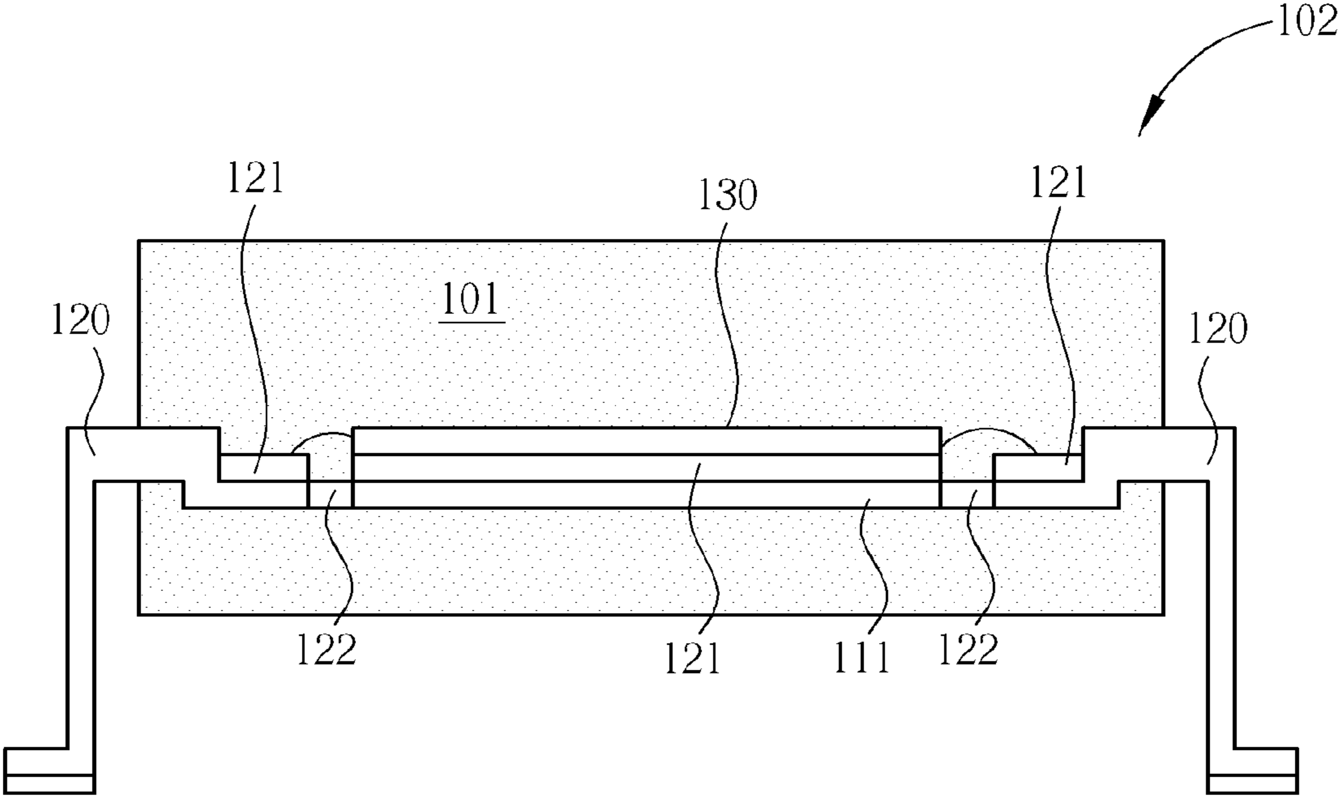
FIG. 4 PRIOR ART
