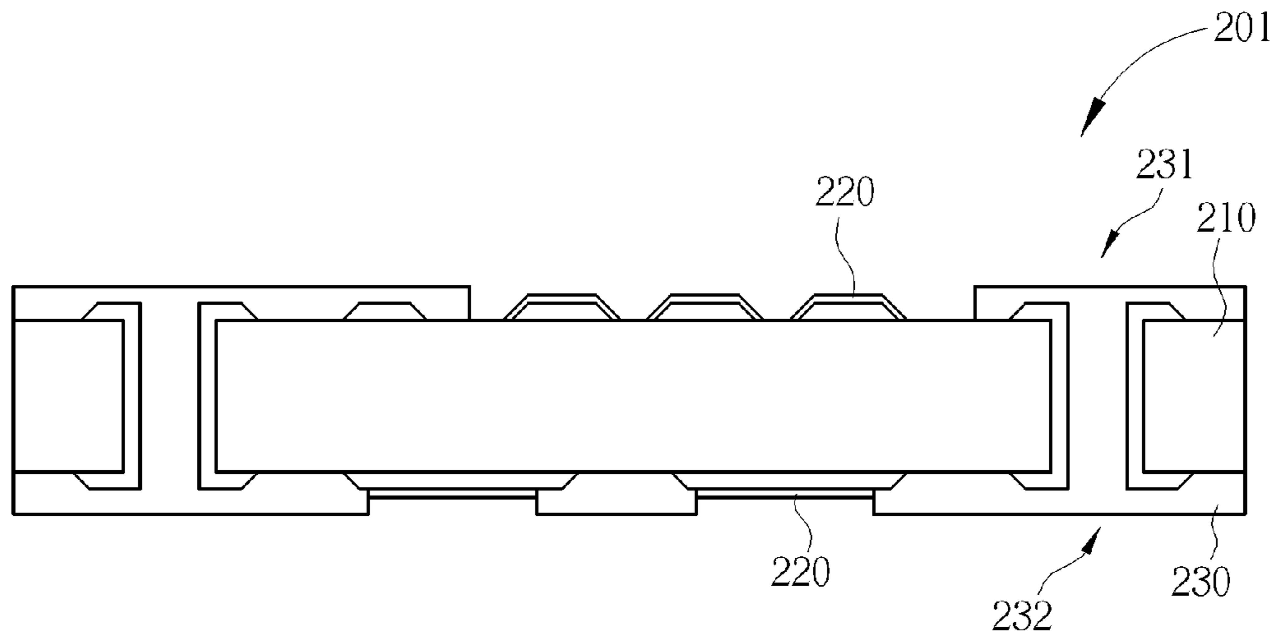
FIG. 5 PRIOR ART
