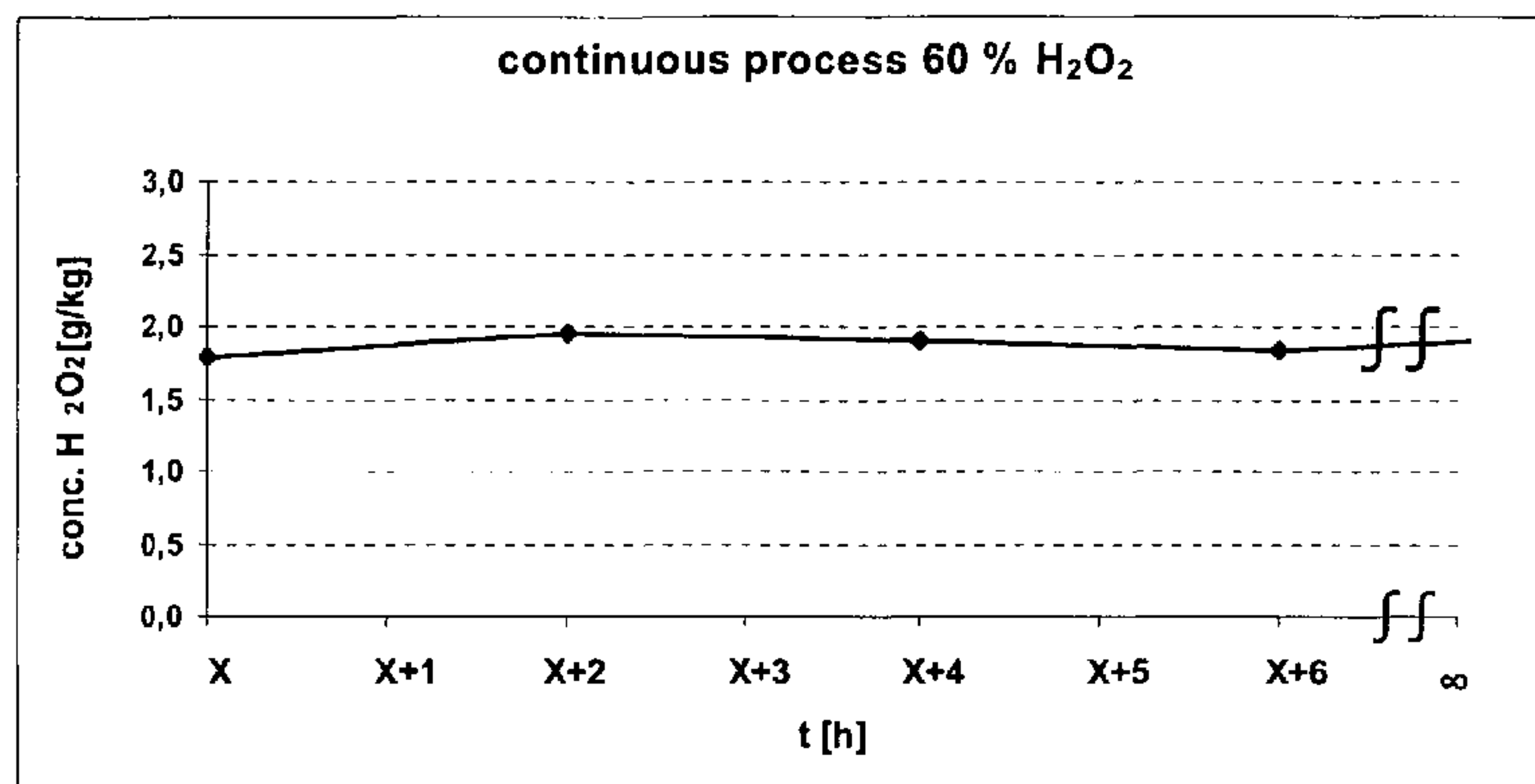
Hydrogen peroxide concentration in the reaction mixture during step a) of the Example 1 (continuous process according to the invention with a H 2 O 2 starting concentration of 60%);
