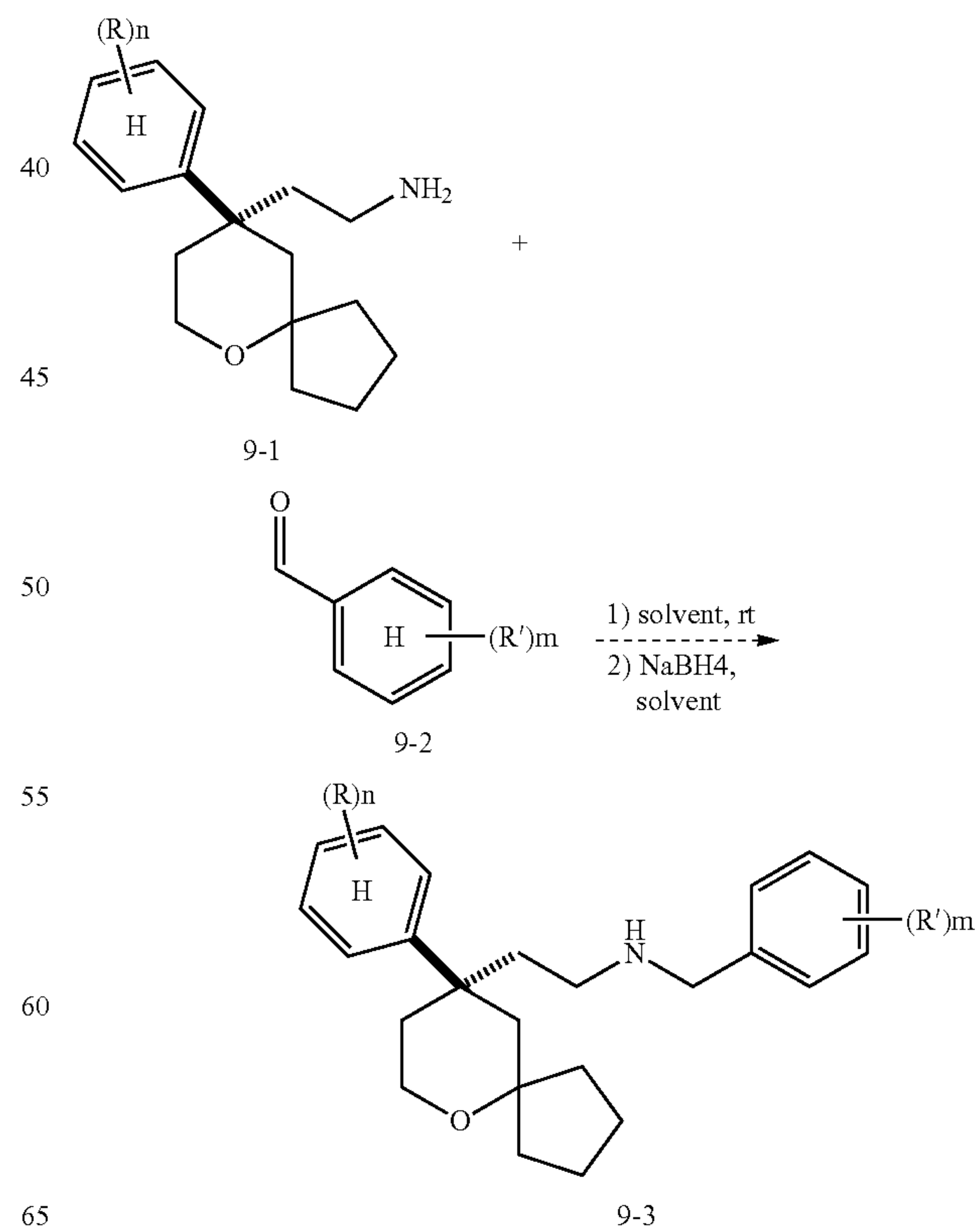
Scheme 9
