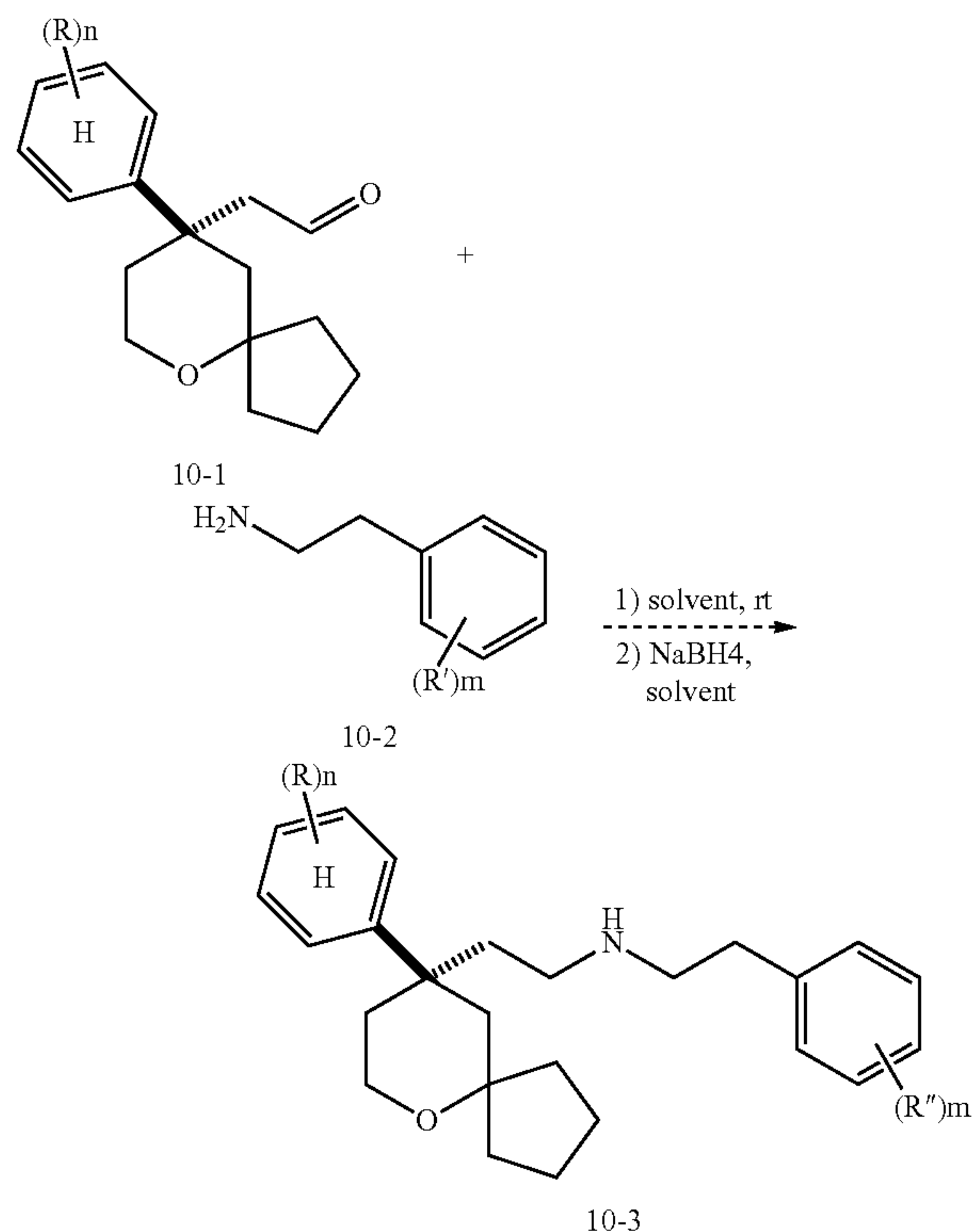
Scheme 10
