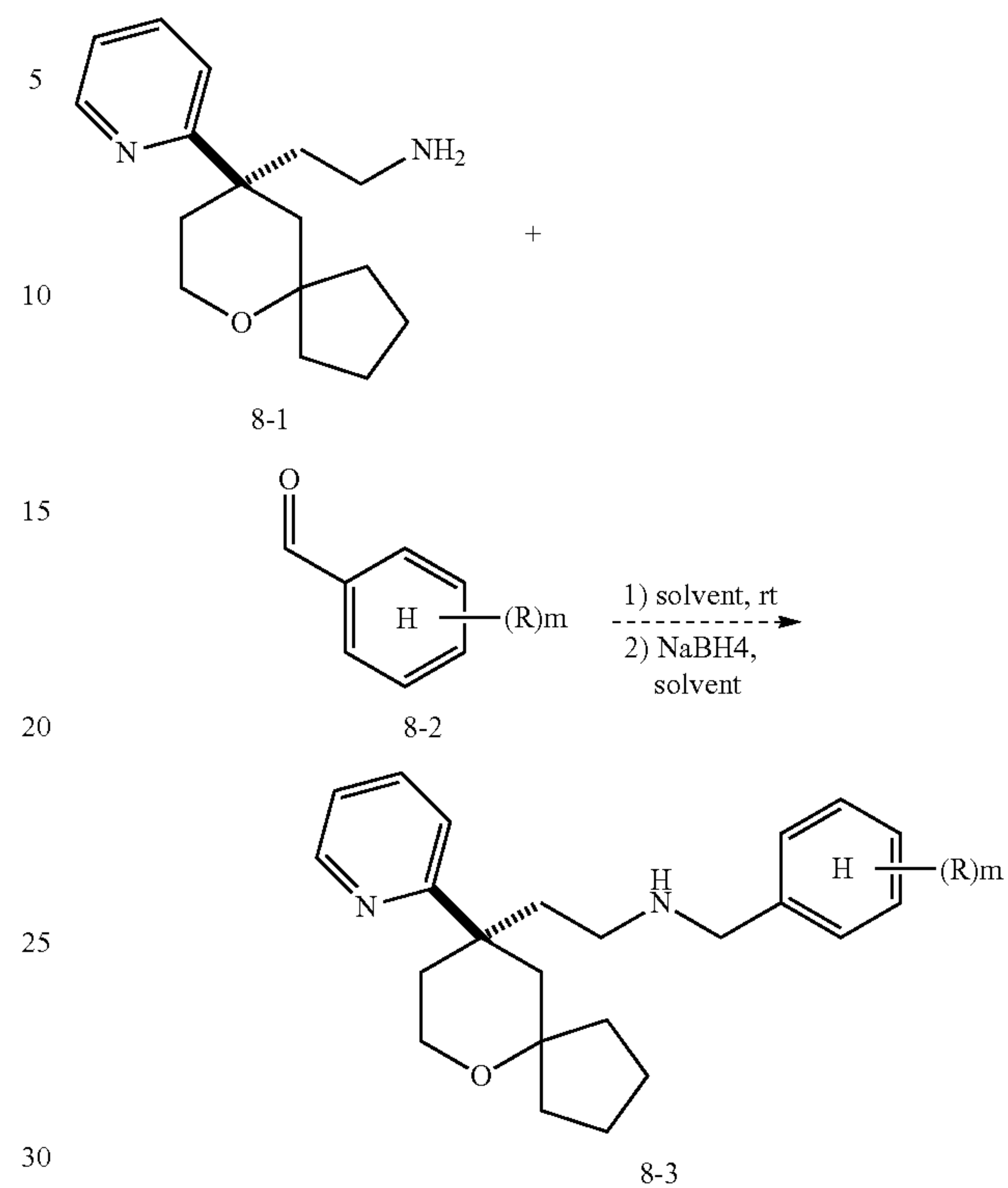
Scheme 8
