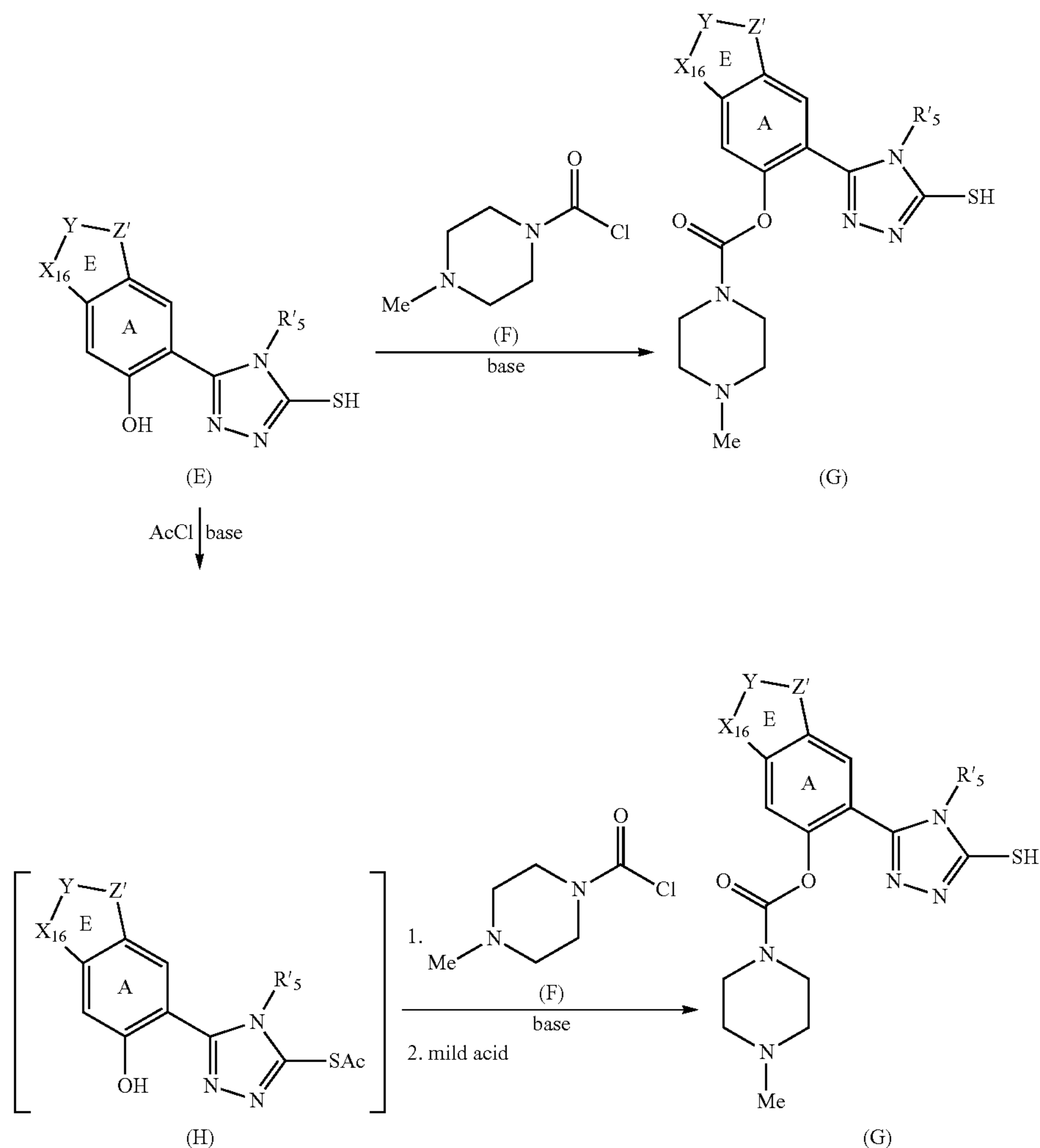
Scheme IX: Preparation of prodrugs in which the 4-hydroxy group of compounds of the invention is protected with 4-methyl-piperazine-1-carbamoyl.
