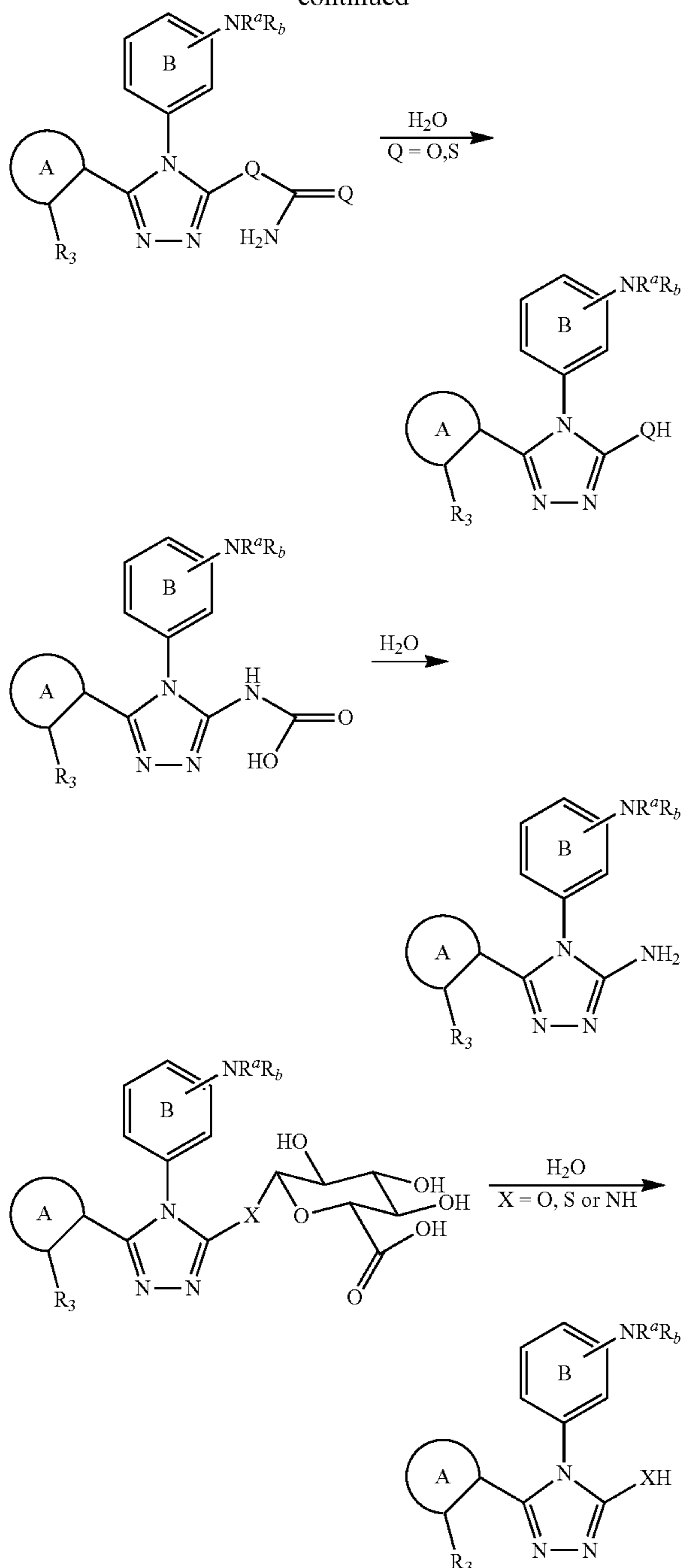
Scheme I: Synthesis of triazole compounds of the invention
