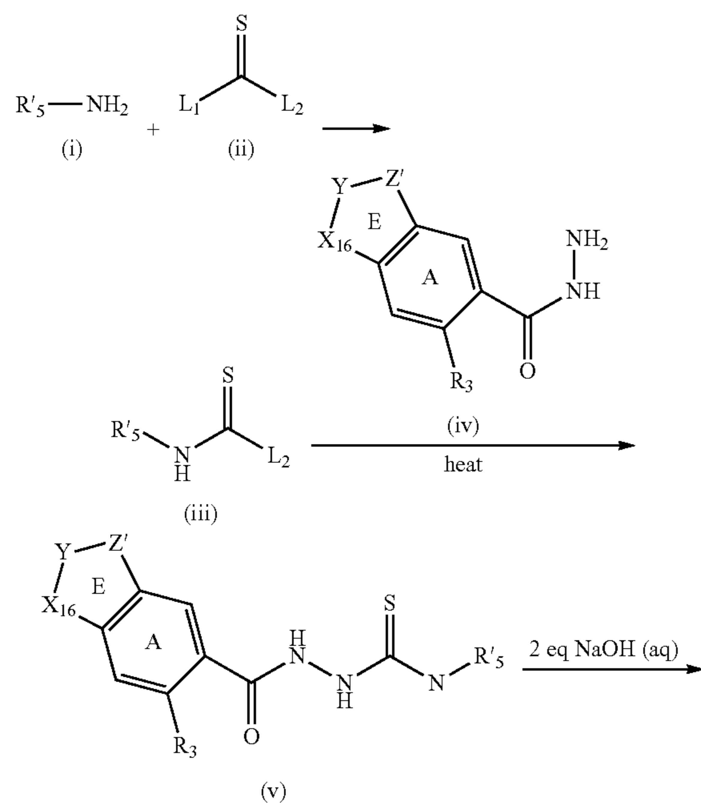
Scheme VI: Alternative synthesis of triazole compounds of the invention
