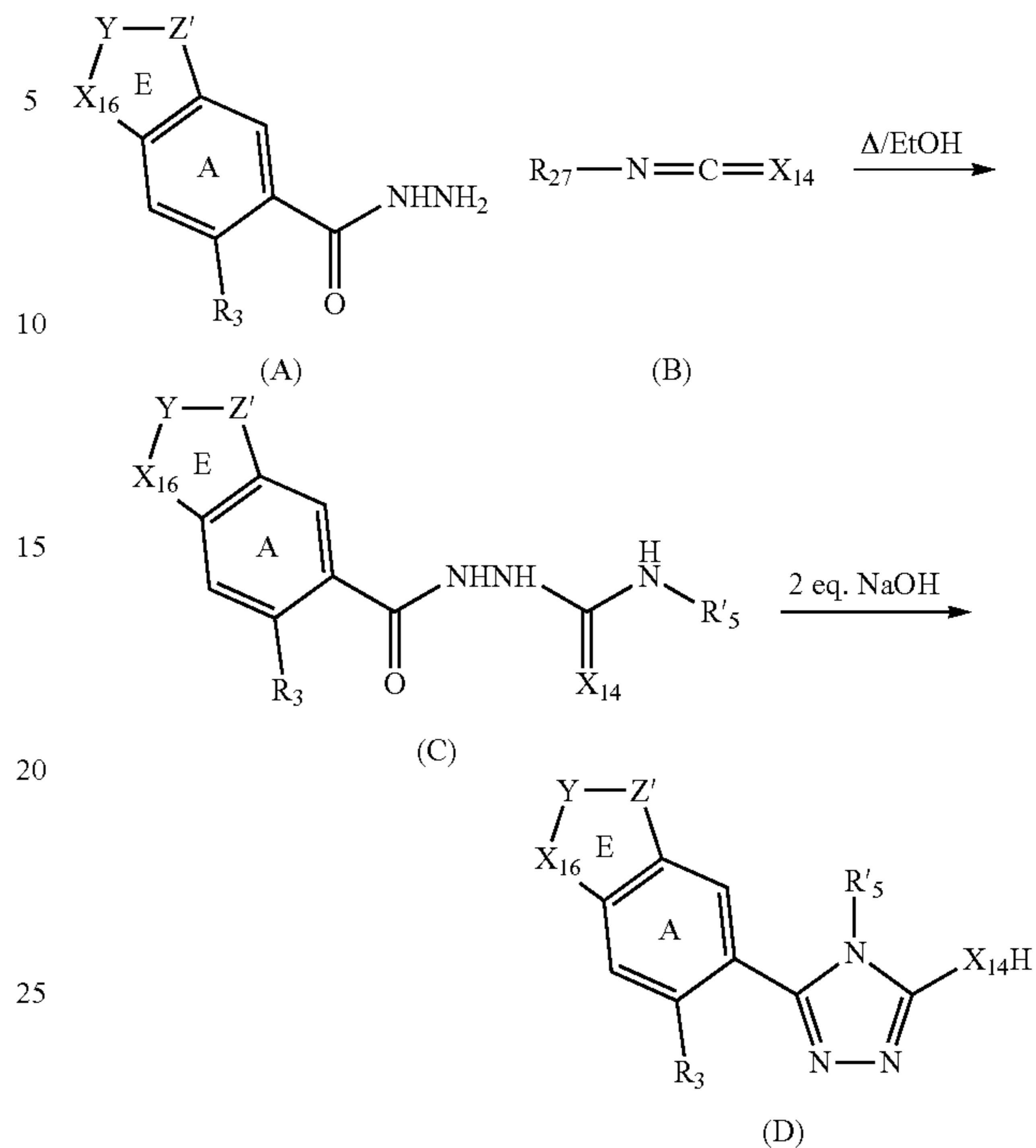
Scheme V: Synthesis of triazole compounds of the invention
