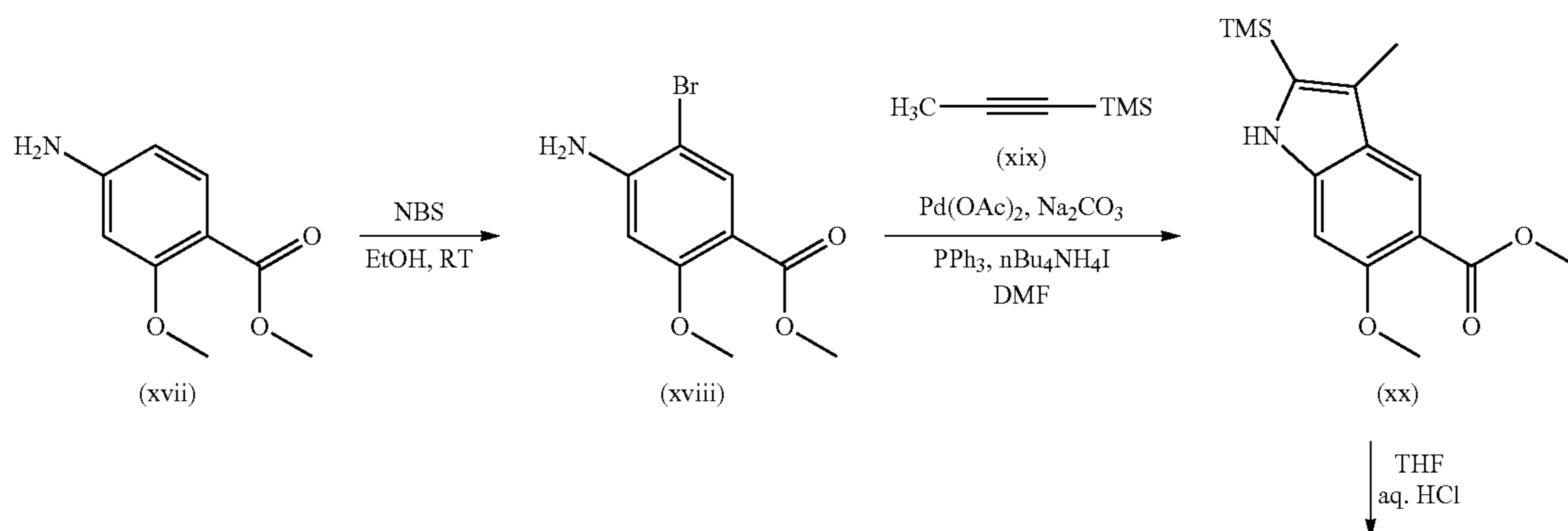
Scheme VIII: Method of preparing a 1H-indole-hydrazide
