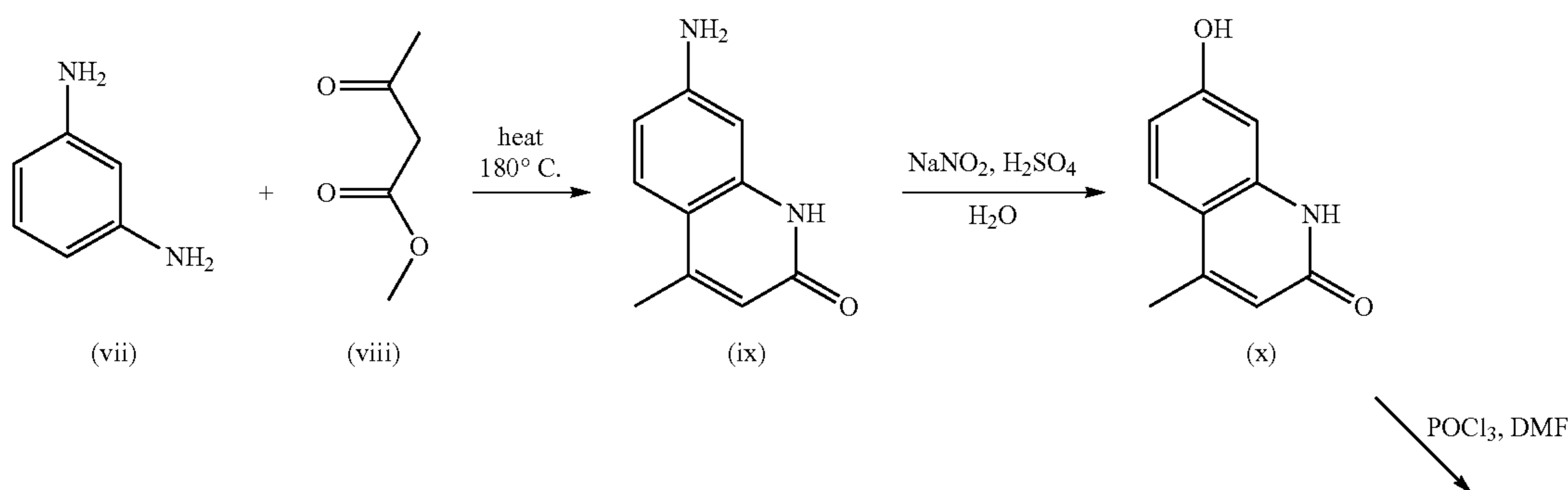
Scheme VII: Alternative synthesis of triazole compounds of the invention
