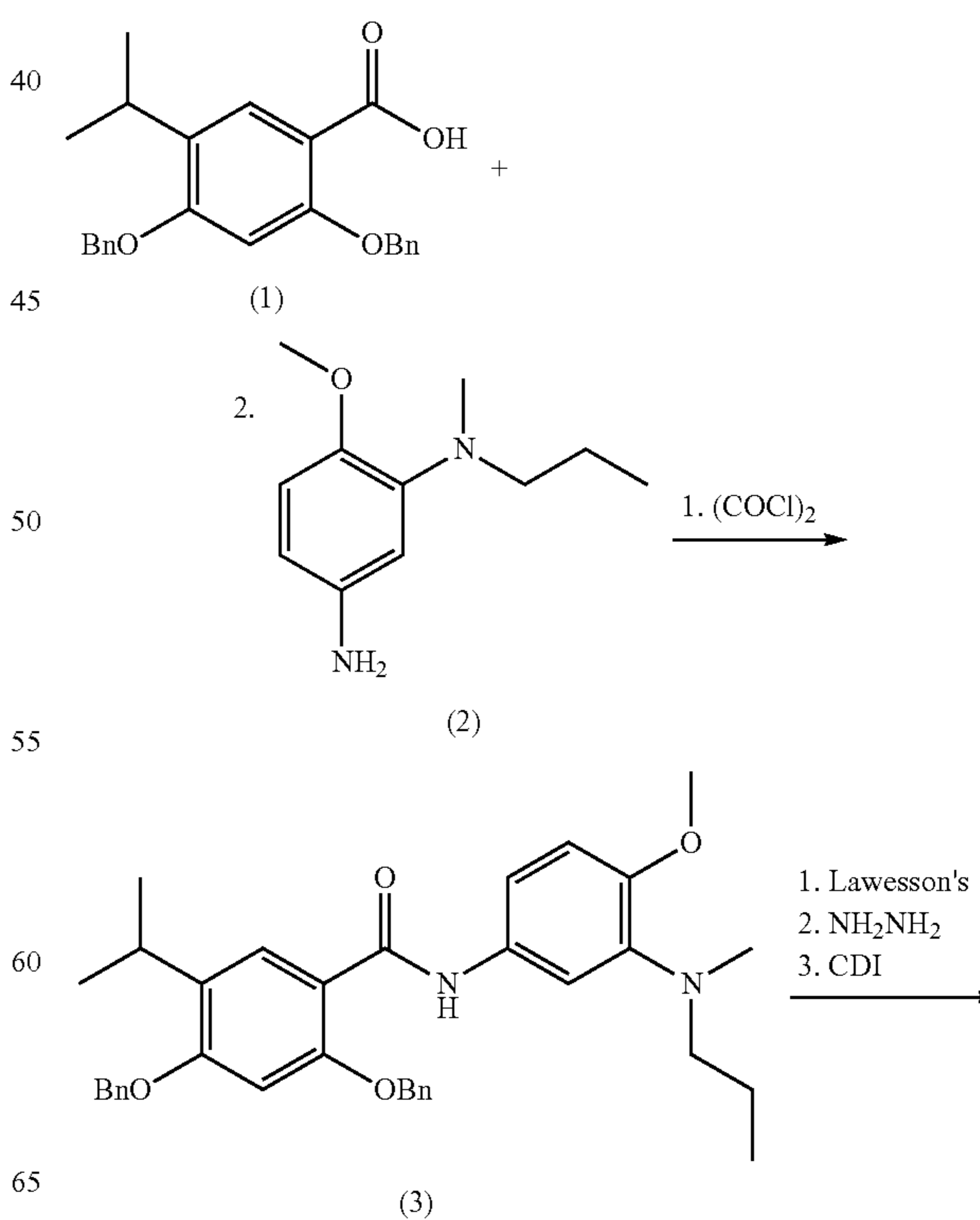
Scheme I: Synthesis of triazole compounds of the invention
