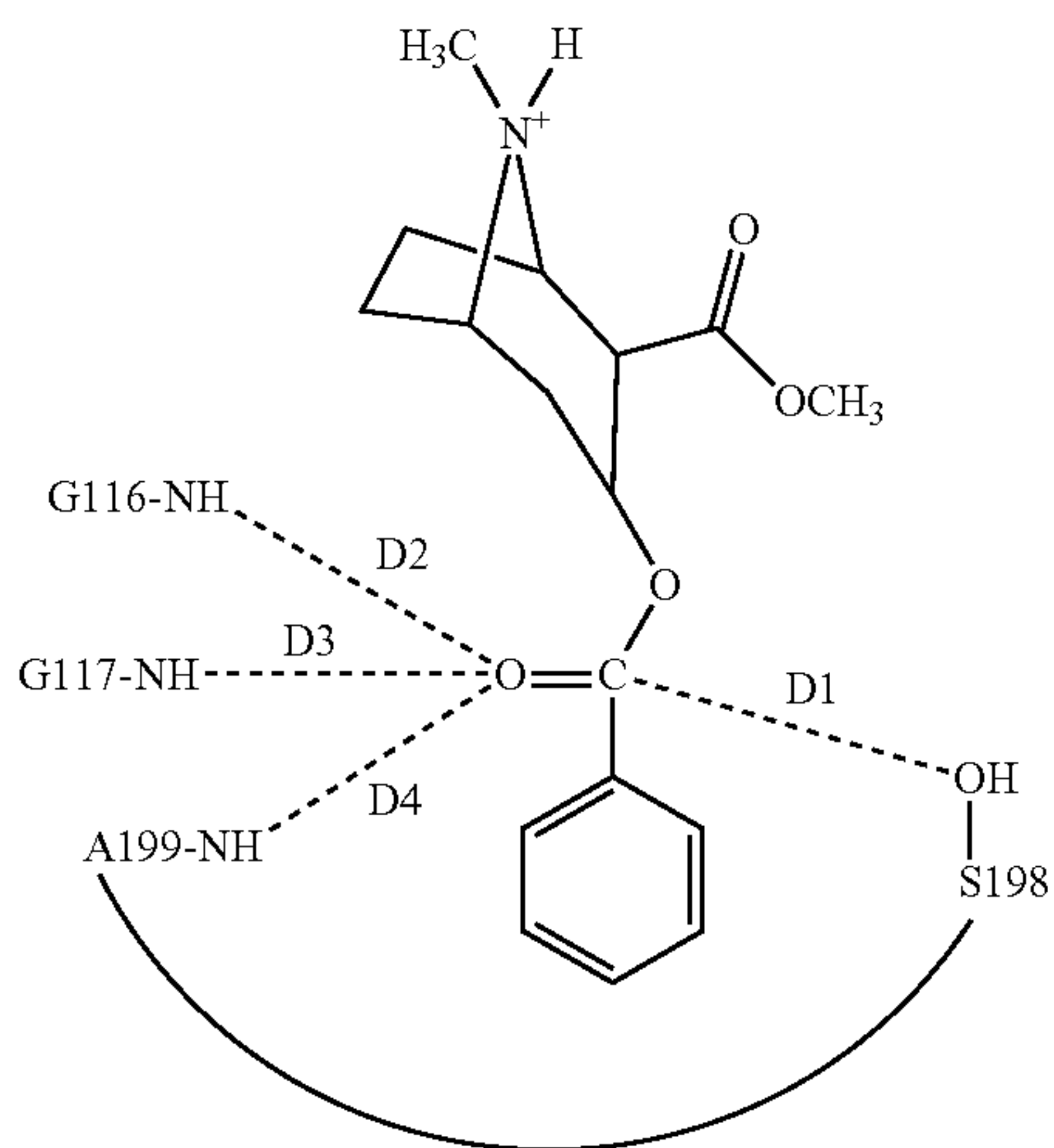
Scheme 2. Hydrolysis of (-)-cocaine and (+)-cocaine.
