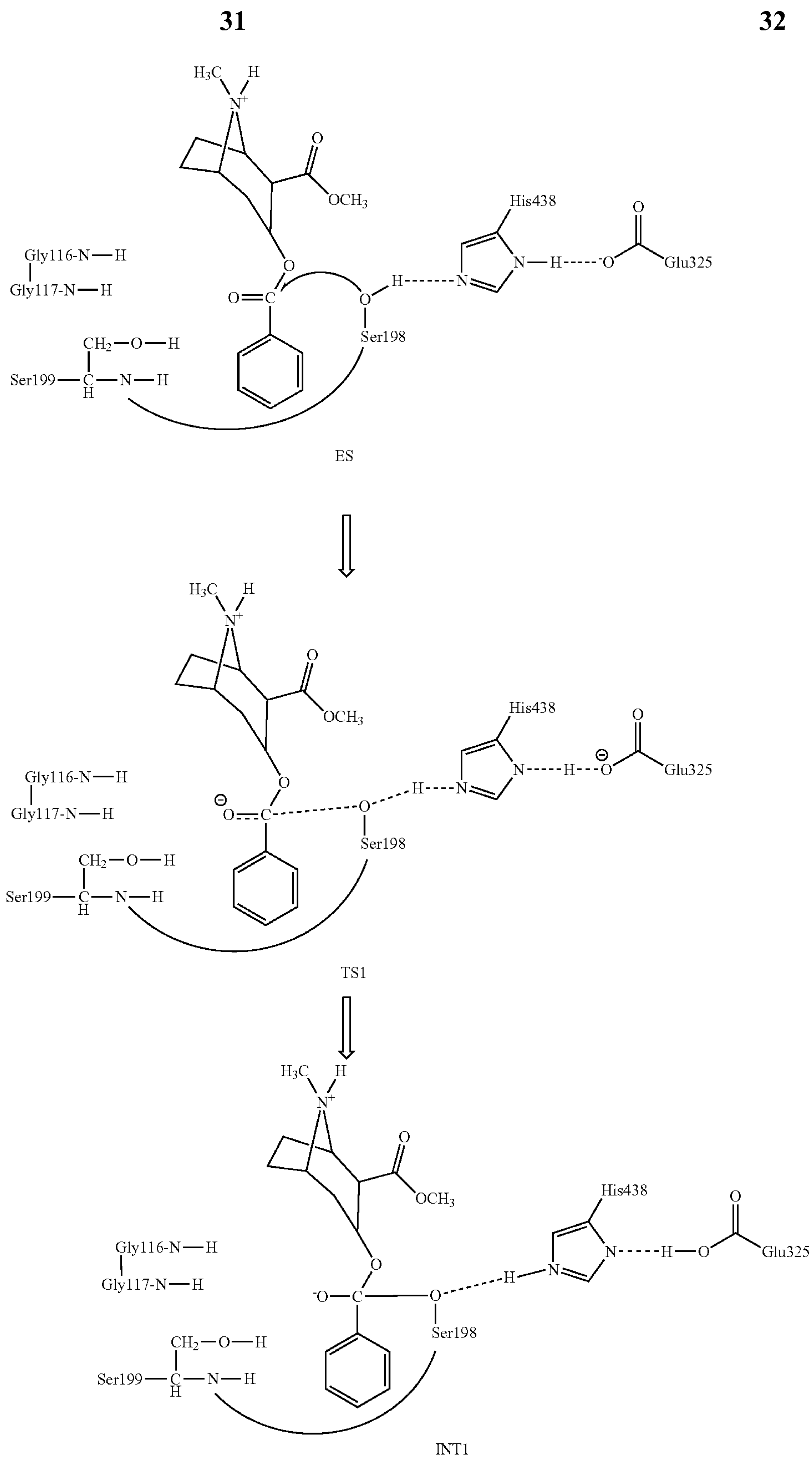
Scheme 4. Schematic representation of the first reaction step for (-)-cocaine hydrolysis catalyzed by a BChE mutant with an A199S mutation.
