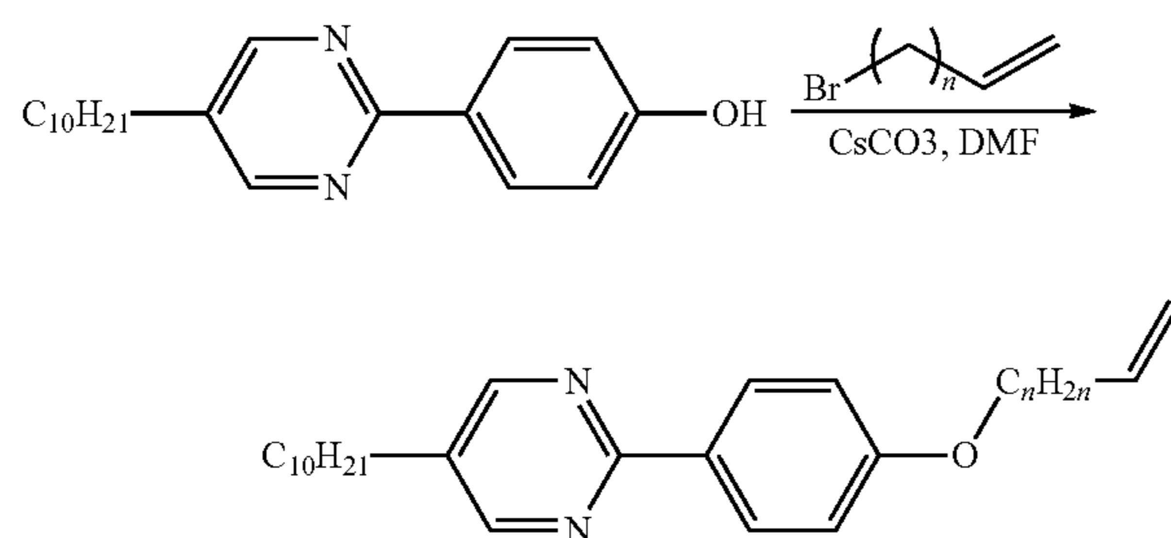
Scheme 6. Williamson ether synthesis of end-on phenyl pyrimidine mesogenic side groups.
