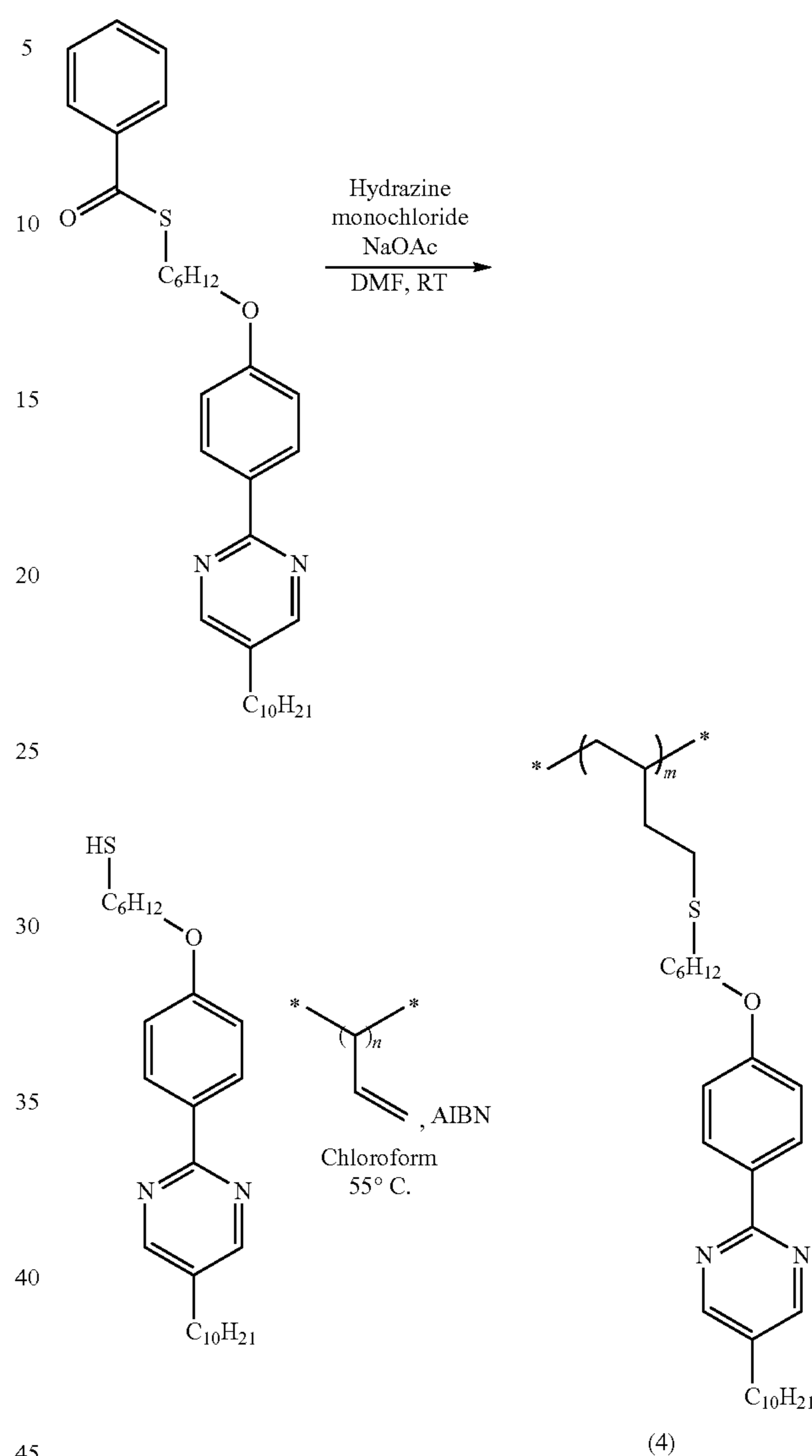
Scheme 9. Thioester cleavage into thiol, followed by direct, radical catalyzed thiol-ene coupling with 1,2-polybutadiene.
