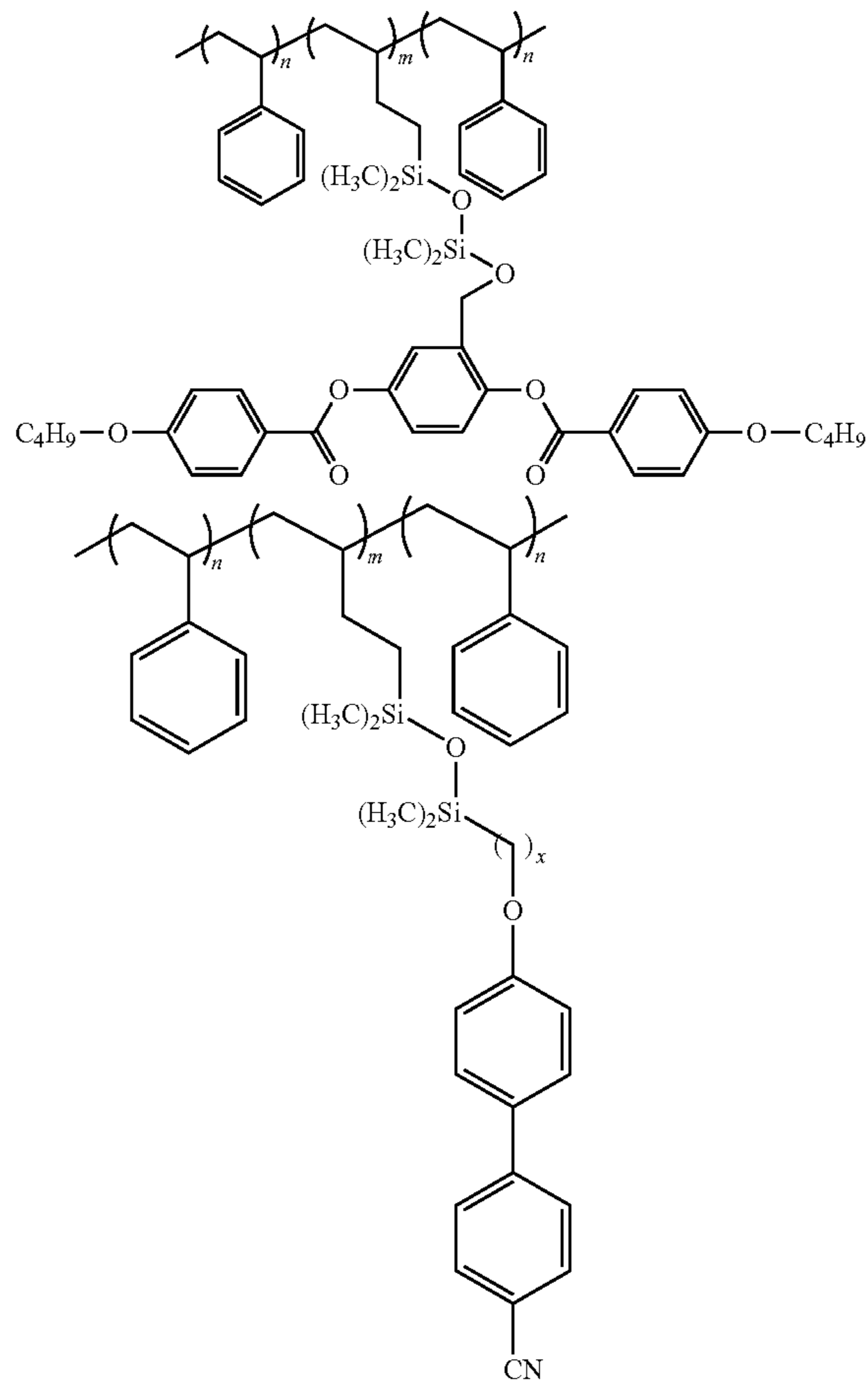
Scheme 13 Example Copolymers
