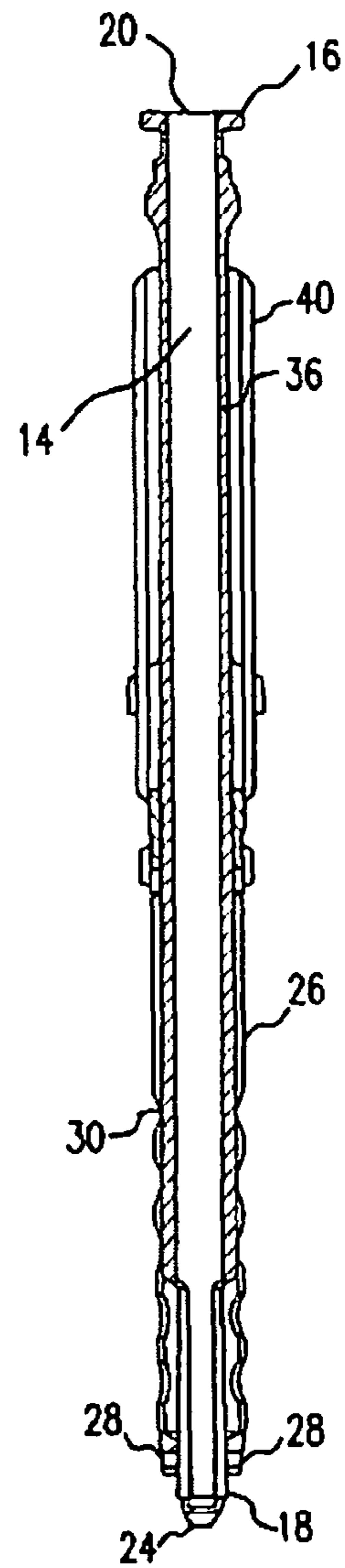
SECTION F-F
