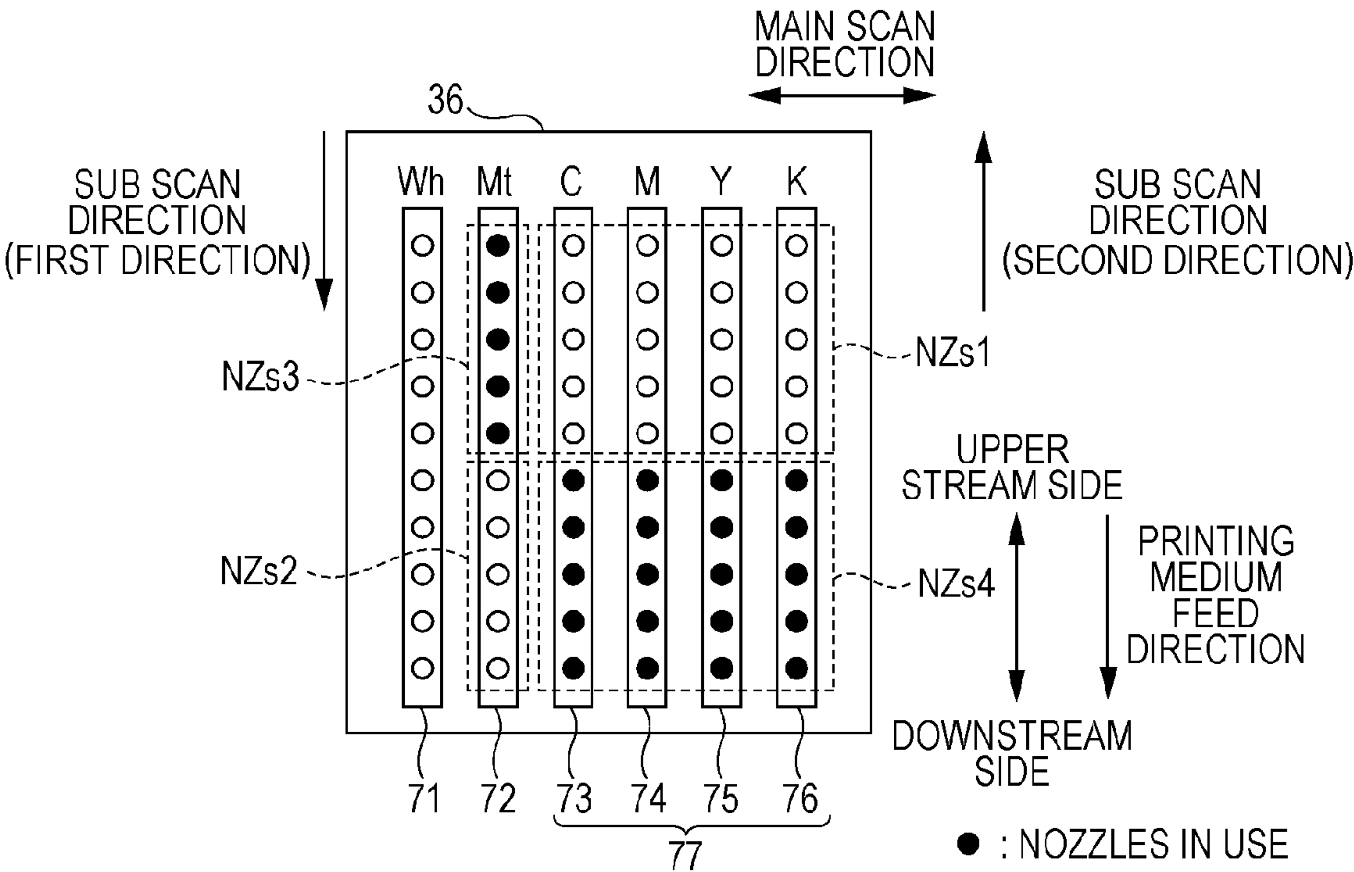
FIG. 8 THIRD NOZZLE USE SETTING
