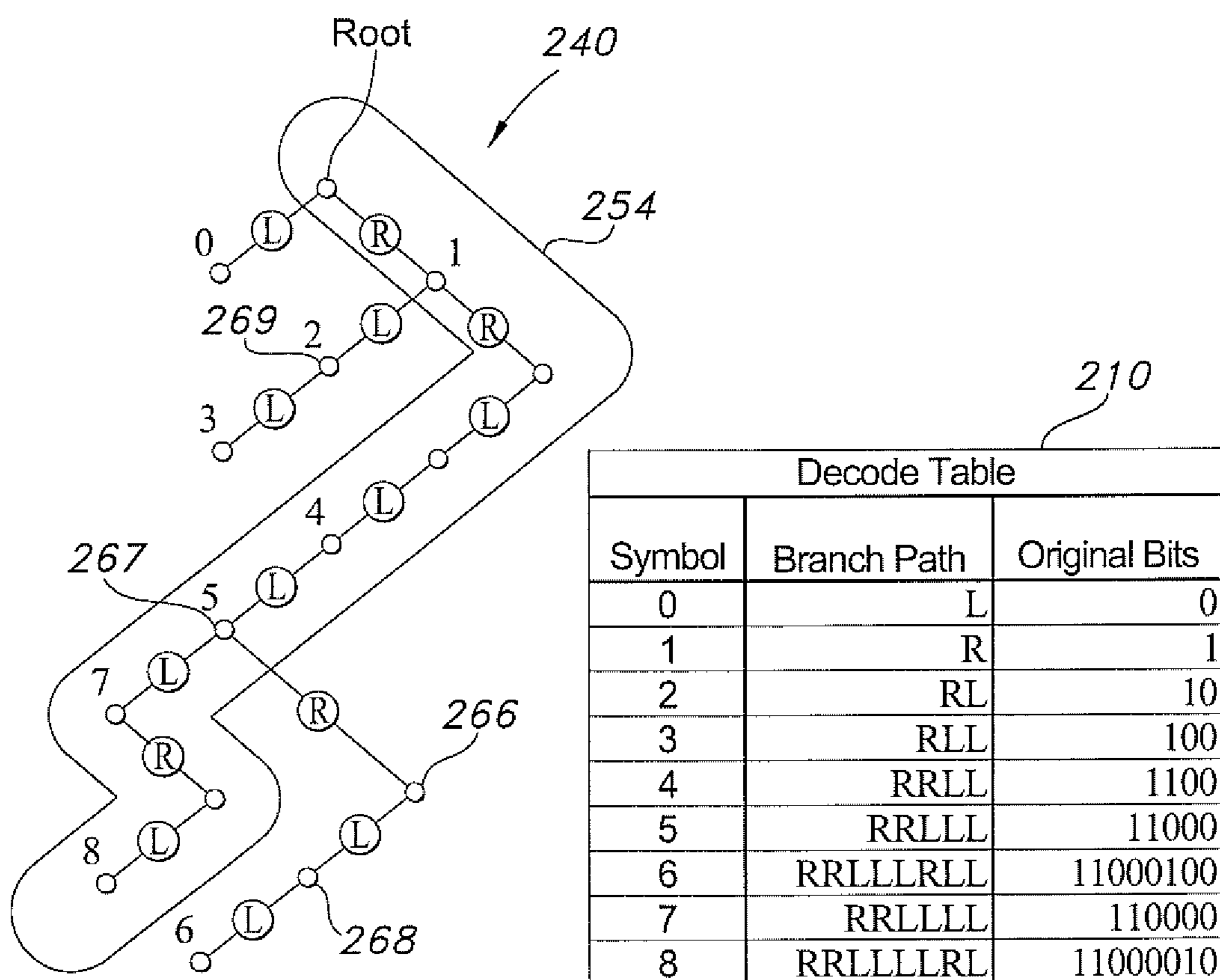
Decode Tree
