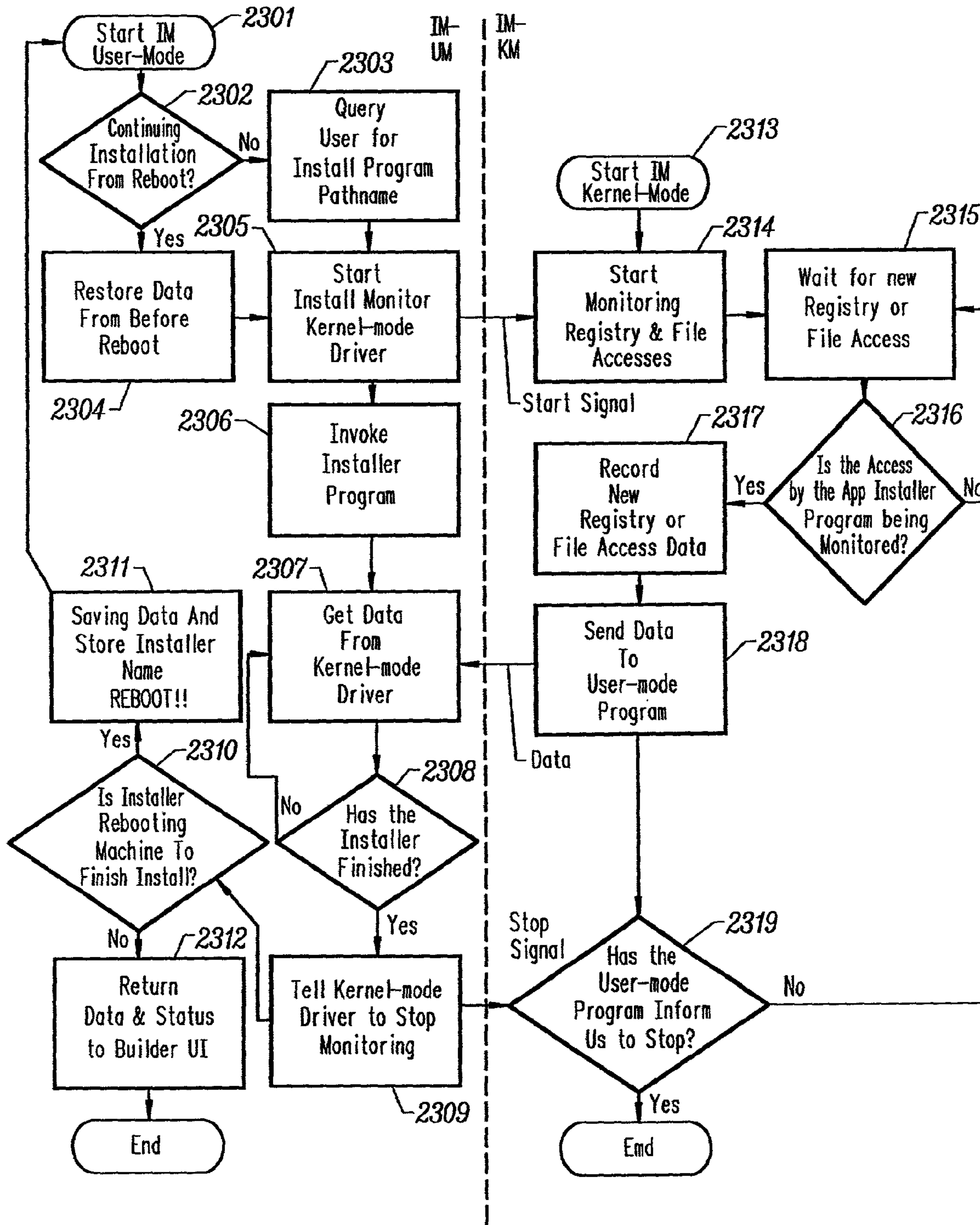
Builder Install Monitor (IM) Control Flow Diagram
