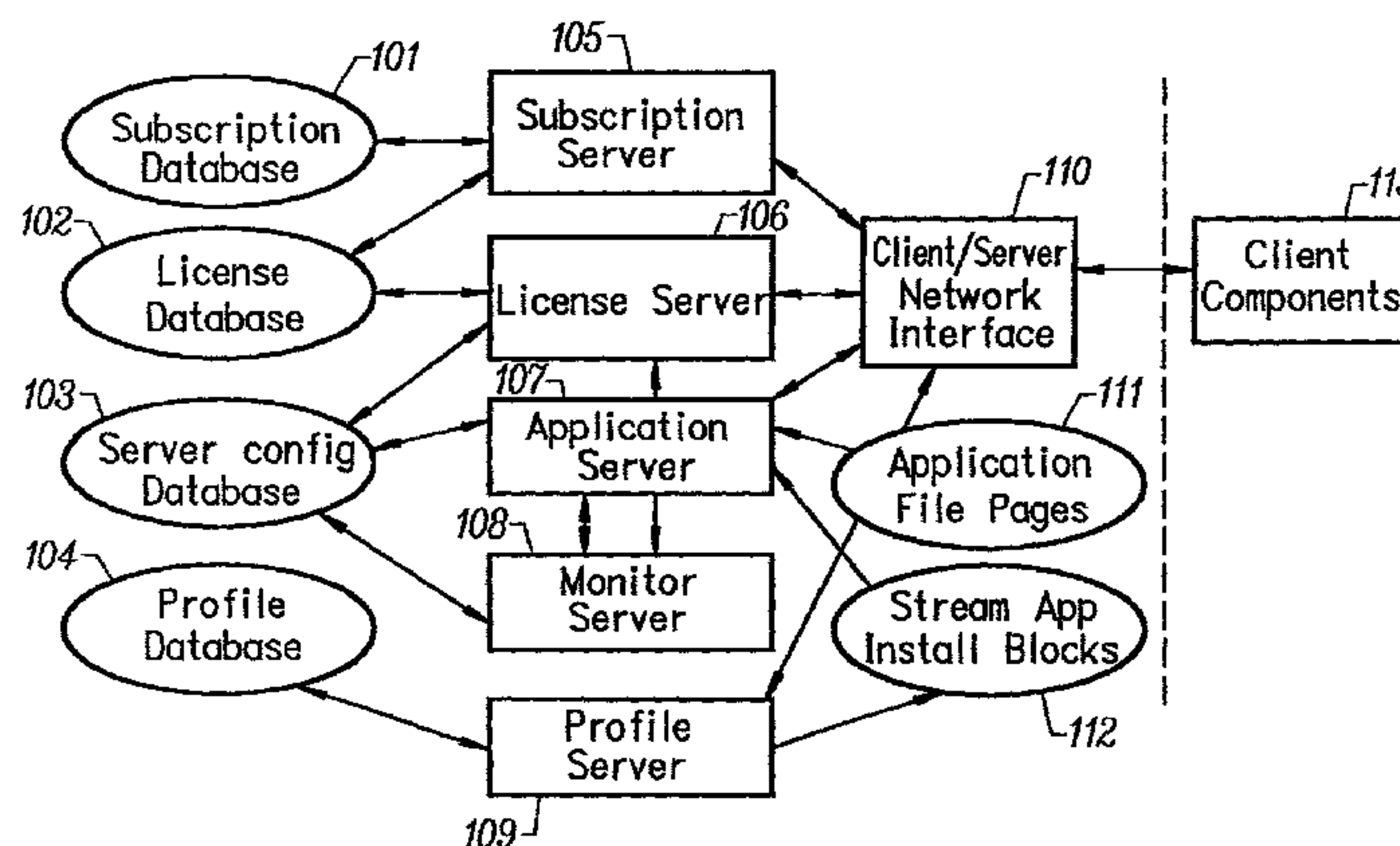
Server Components Supporting Application Delivery & Execution License
