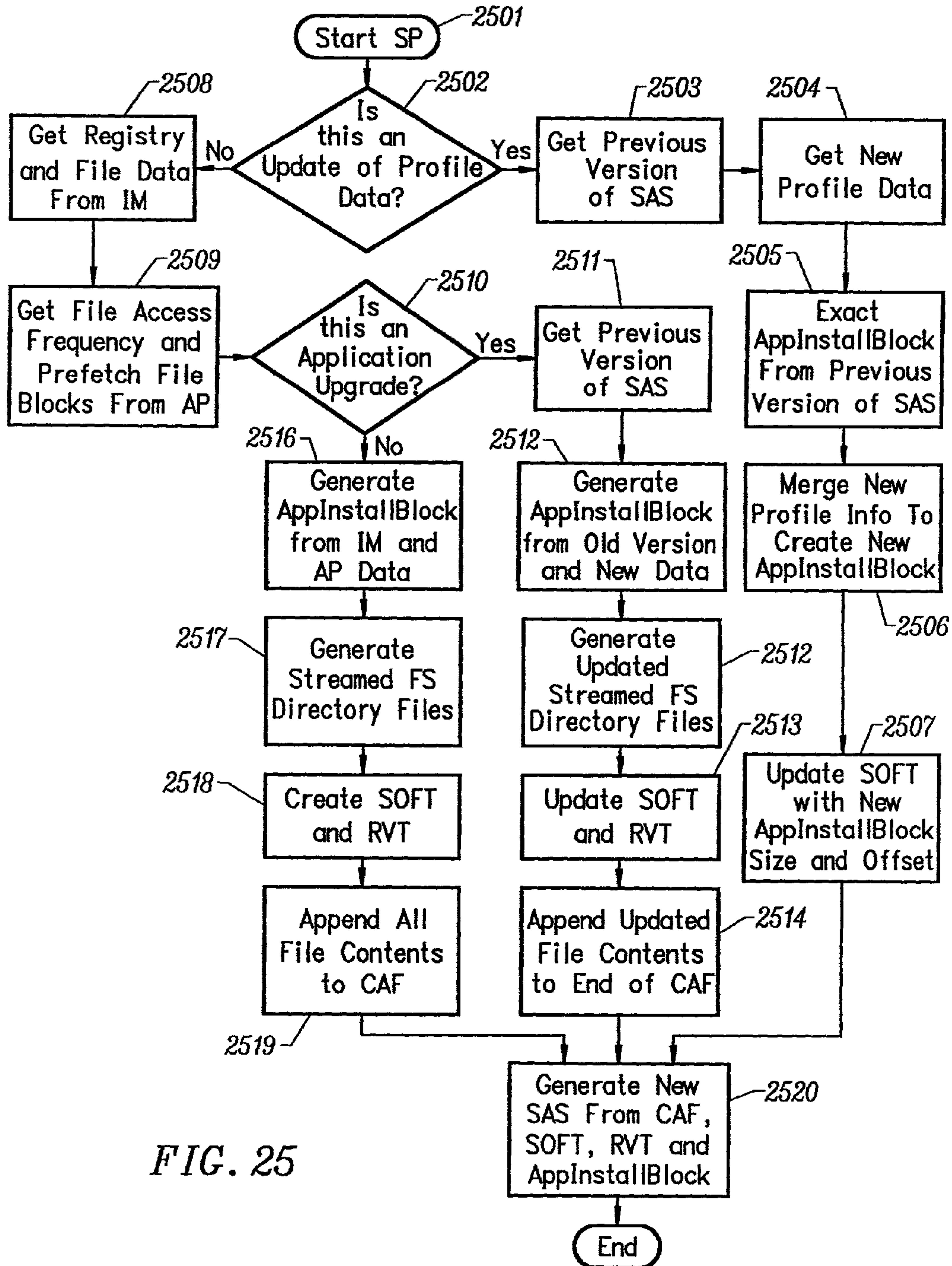
Builder SAS Packager (SP) Control Flow Diagram
