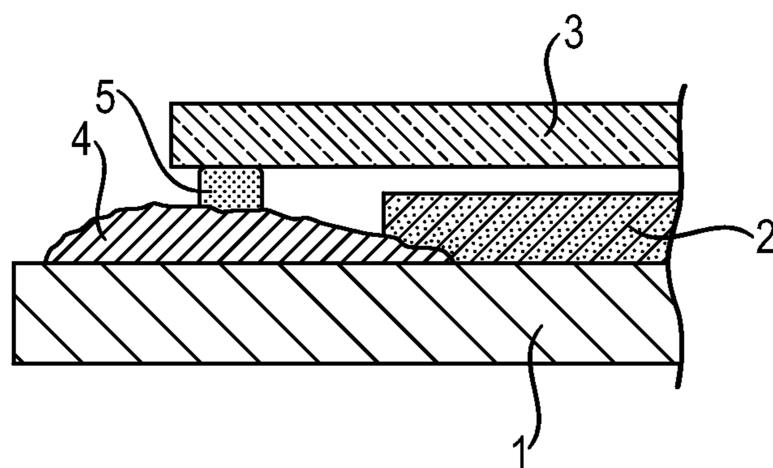
FIG. 2 (prior art)
