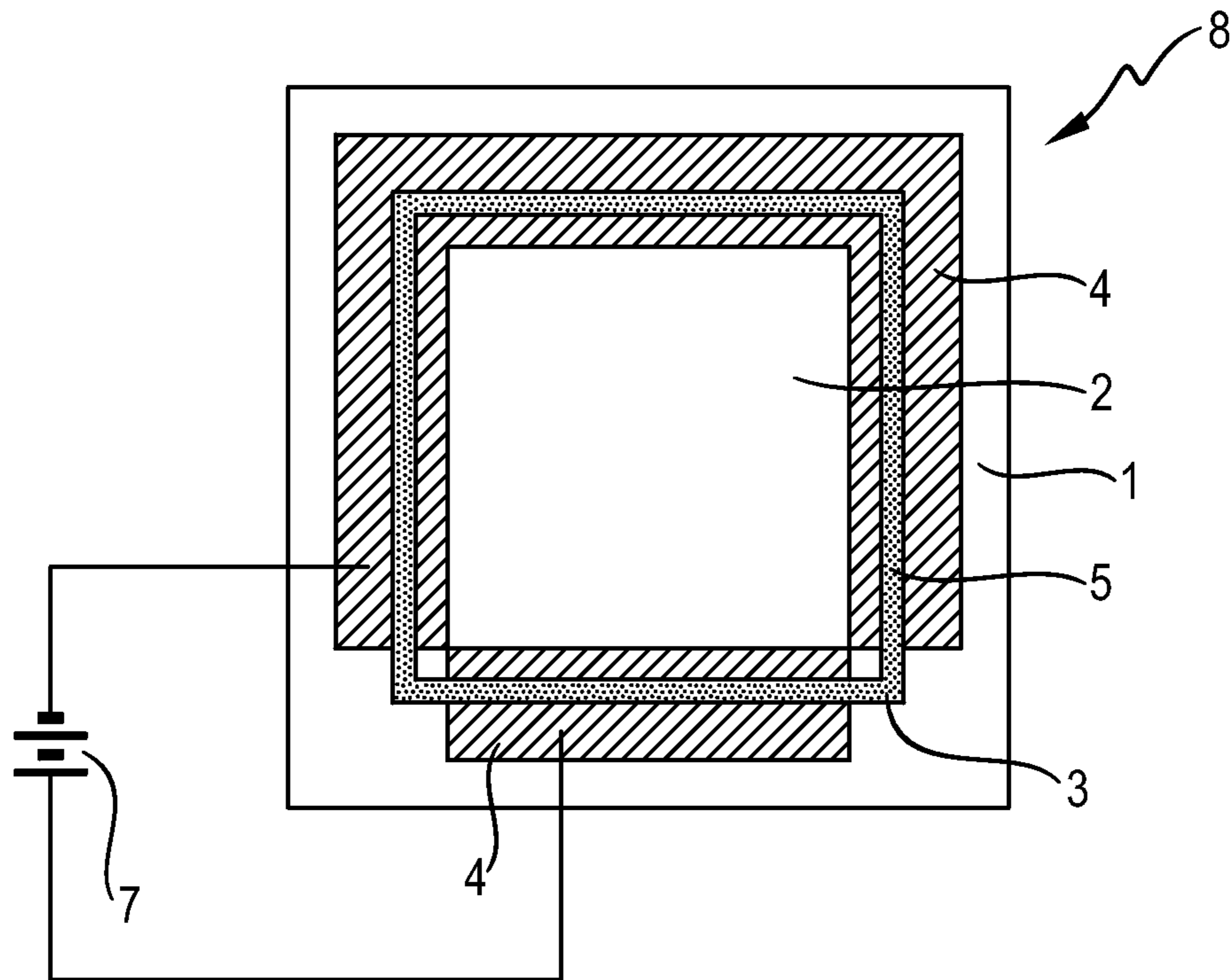
FIG. 1 (prior art)
