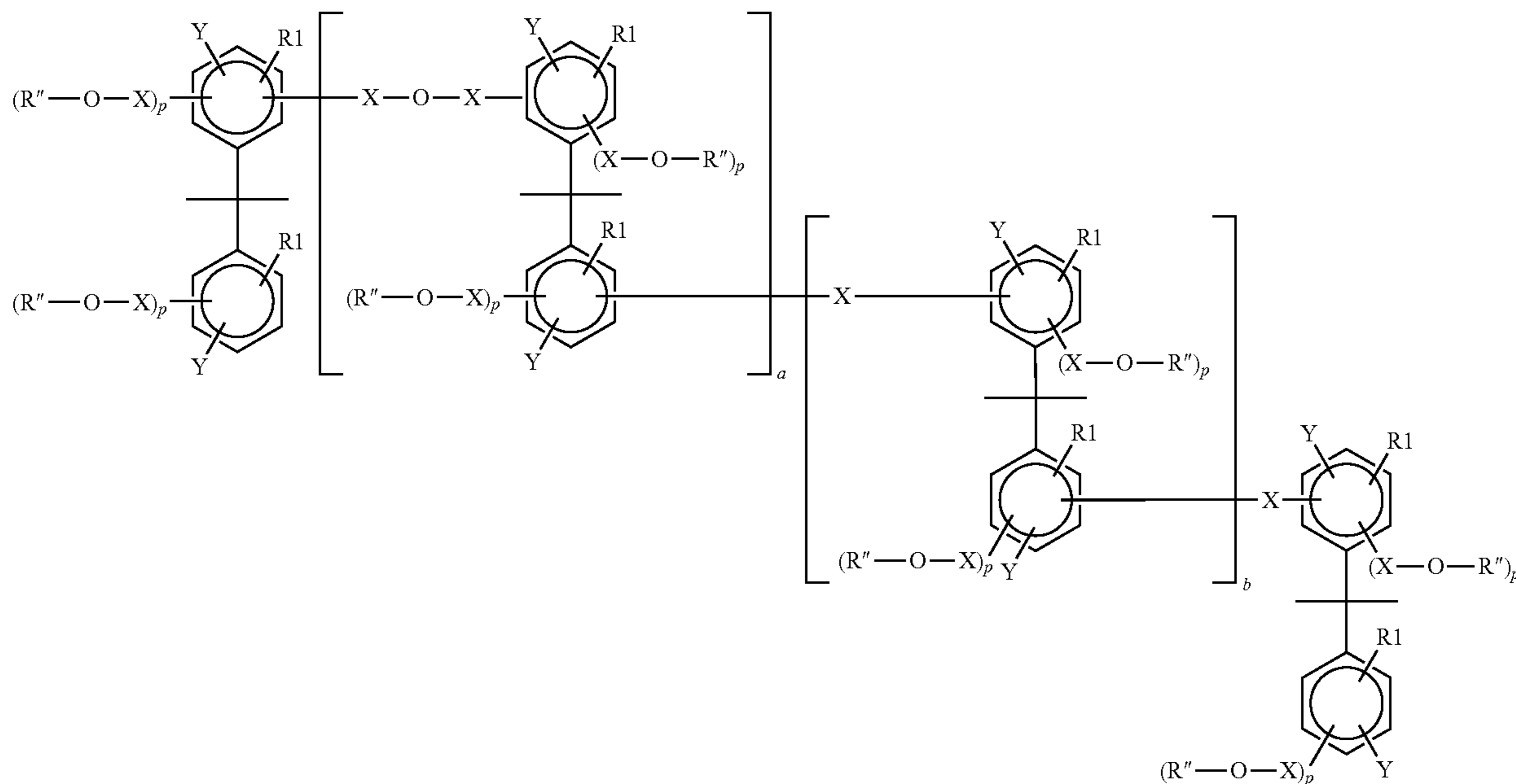
Formula (VI)
