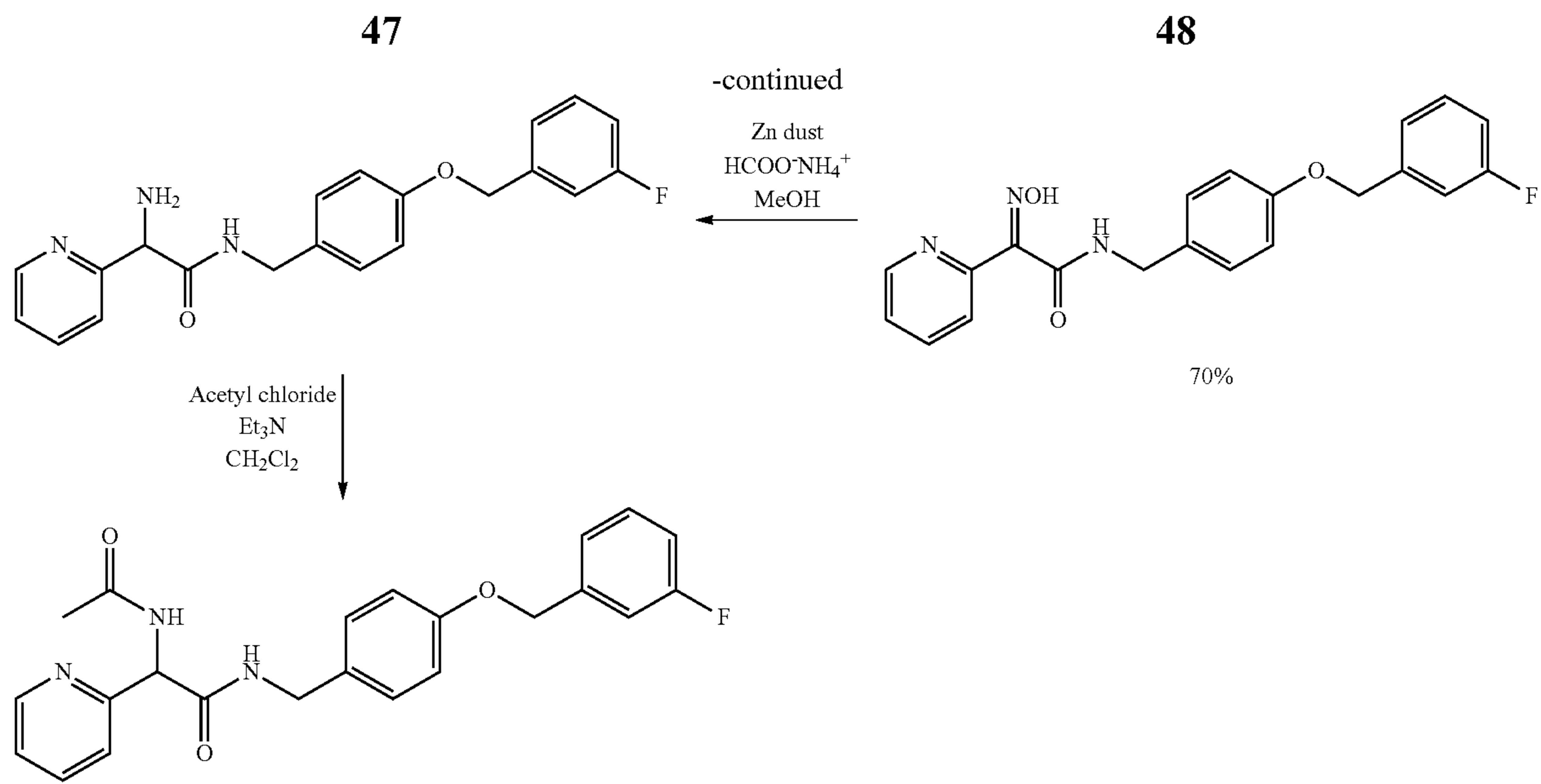
Scheme 6. Preparation of New Neurological Agent: 2-Acetamido-N-(4-(3-fluorobenzoyloxy)benzyl)-2-(thiazol-2-yl)acetamide (Method "F")
