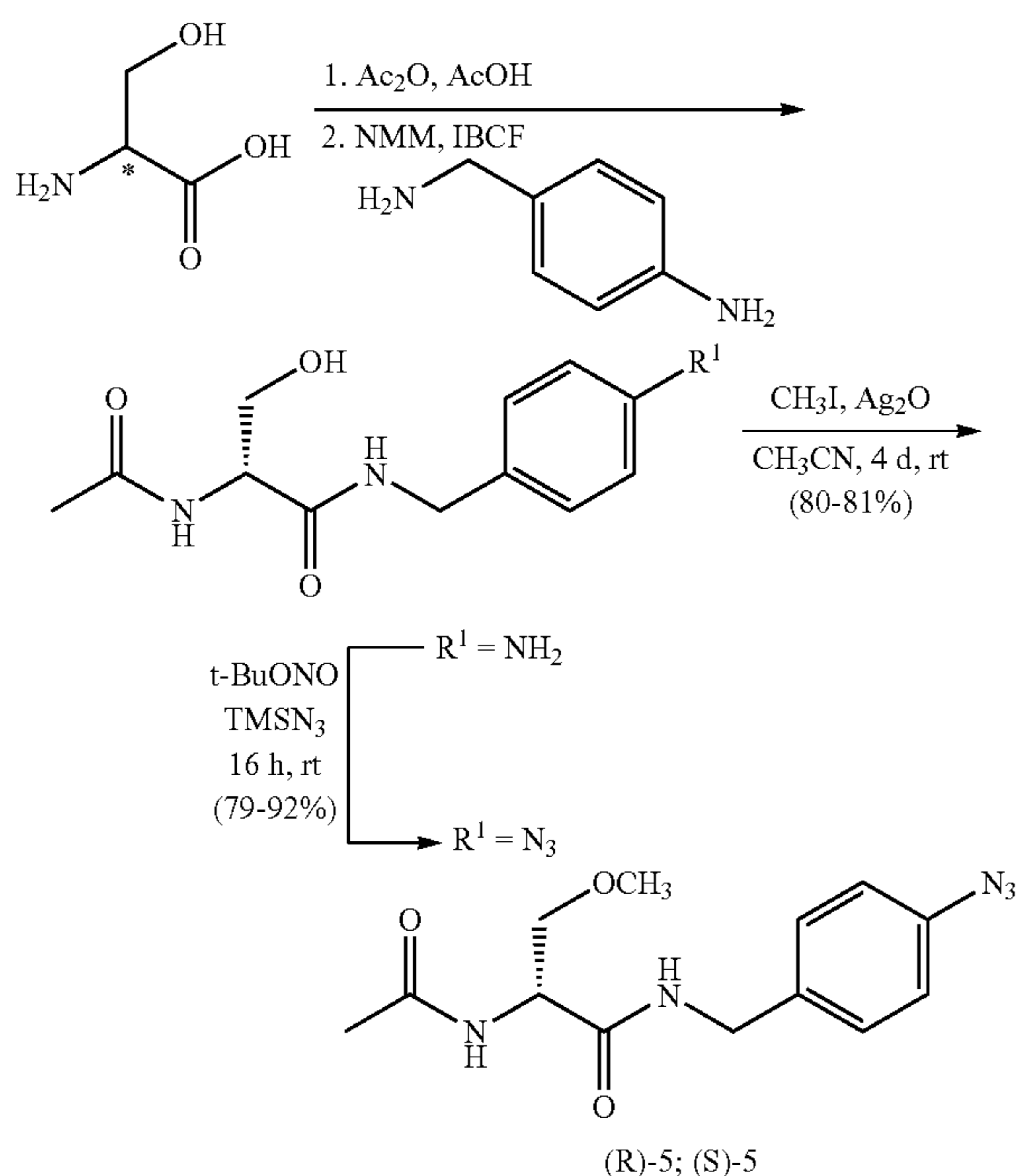
Scheme 3. Preparation of (R)-5 and (S)-5.
