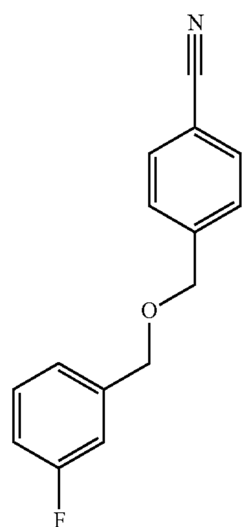
Preparation of 4-(((3-Fluoro)benzyloxy)methyl)benzonitrile
