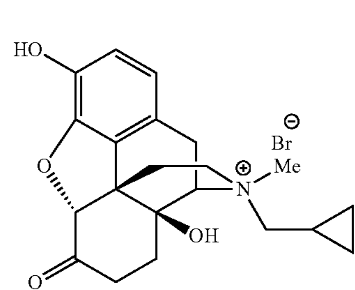
(-)-R-Naltrexone methobromide
