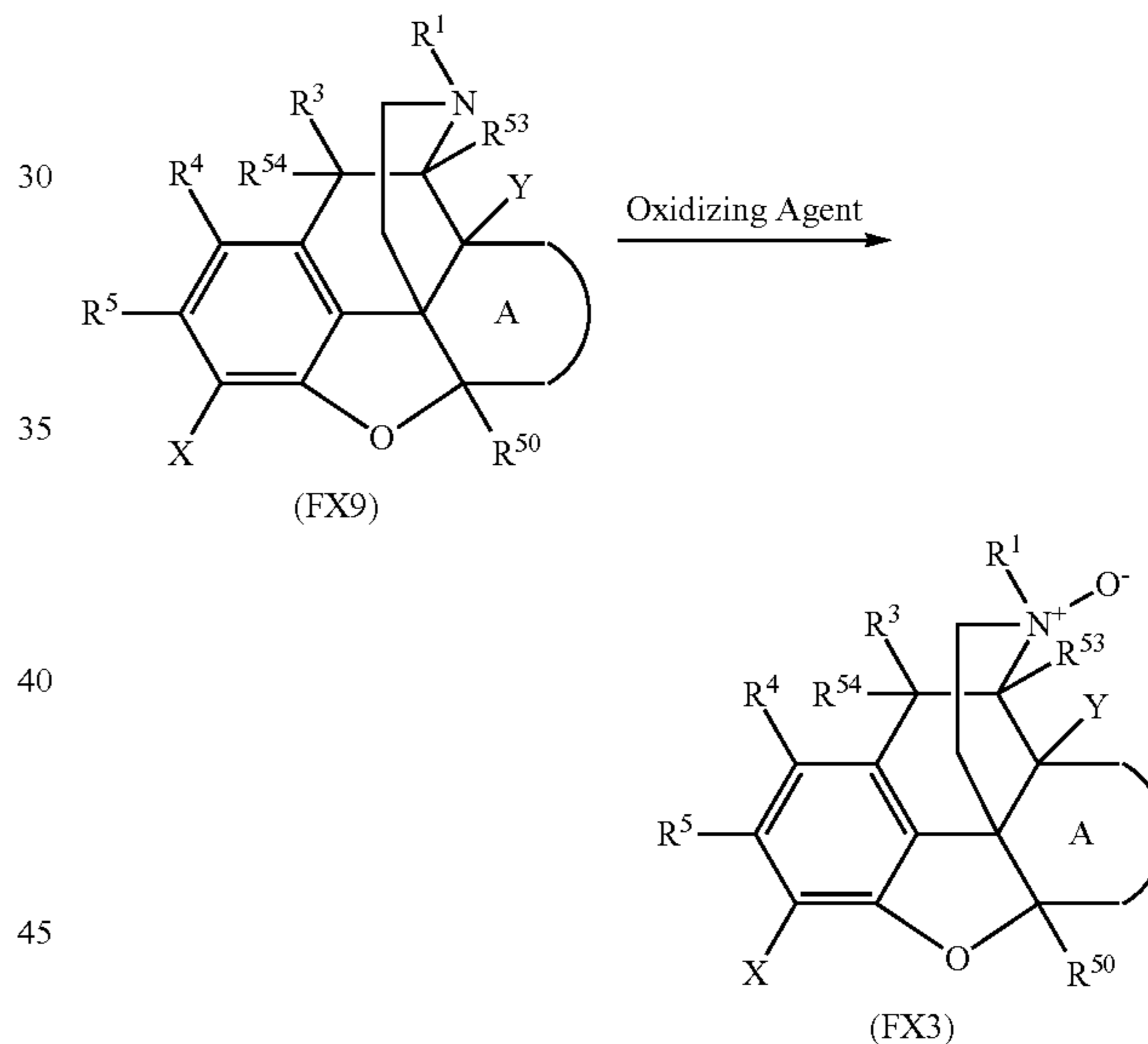
Reaction Scheme 7-1:
