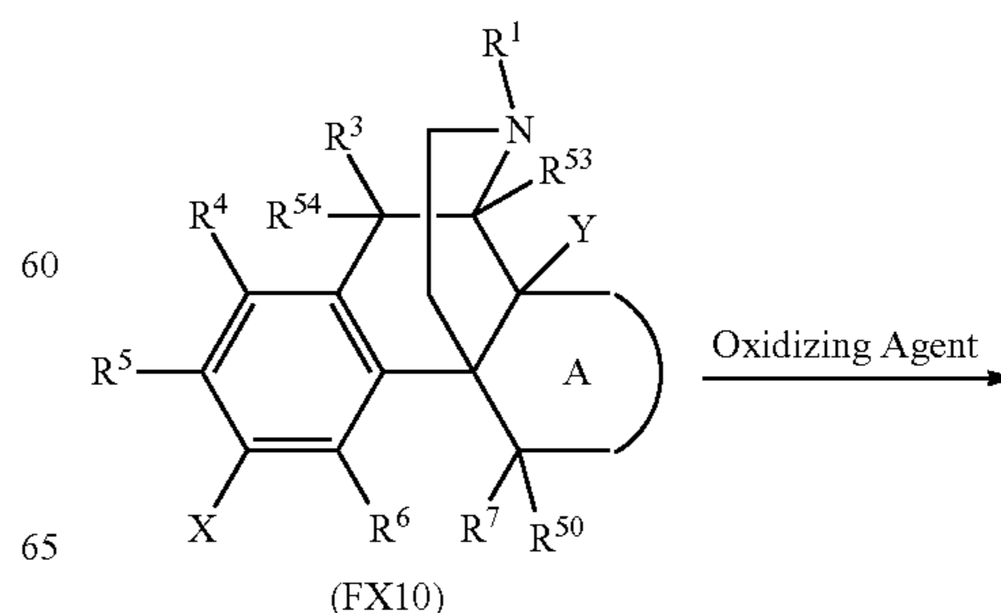
Reaction Scheme 7-2:
