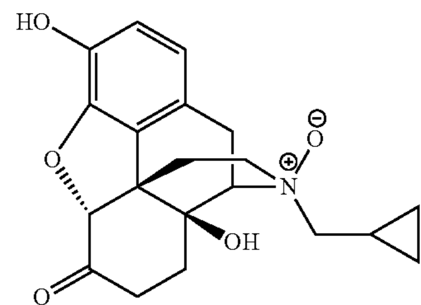
(-)-Naltrexone N-Oxide
