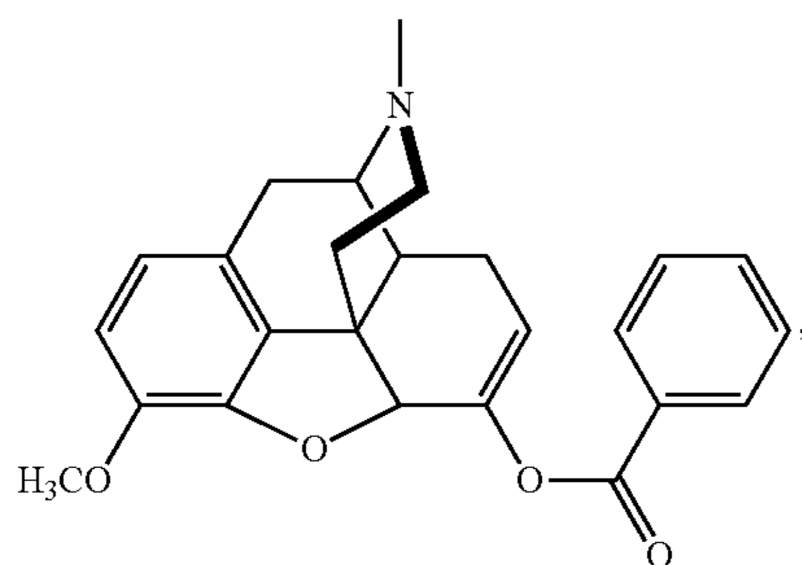
benzoate-hydrocodone (Bz-HC)
