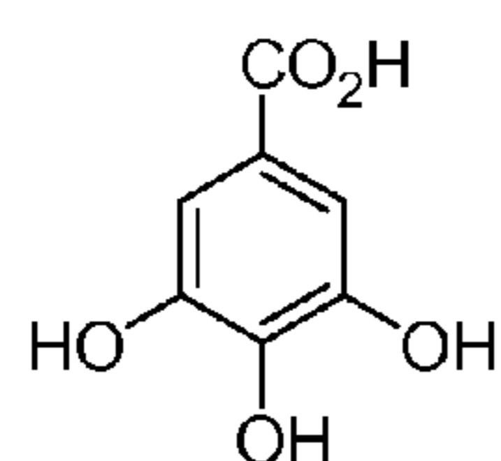
gallic acid
