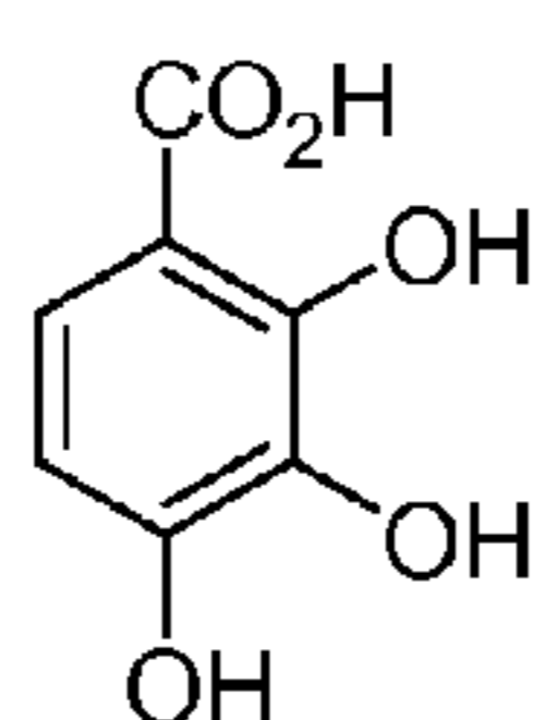
2,3,4-trihydroxybenzoic acid
