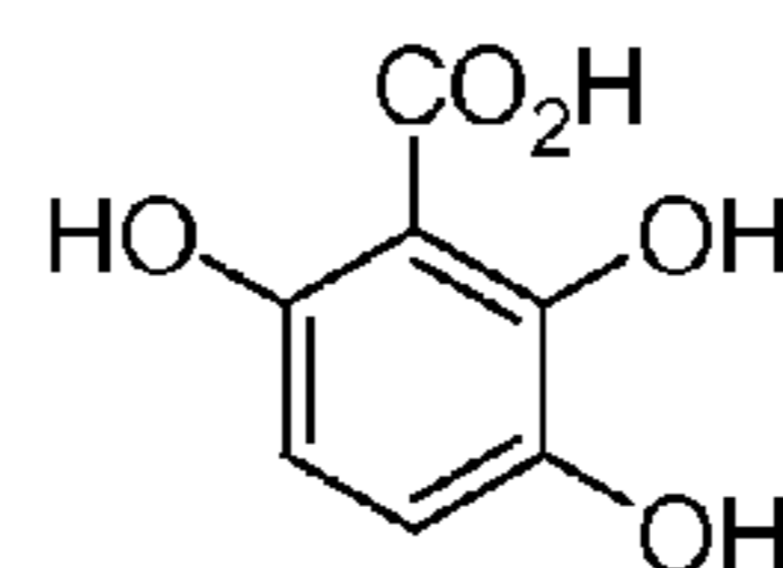
2,3,6-trihydroxybenzoic acid
