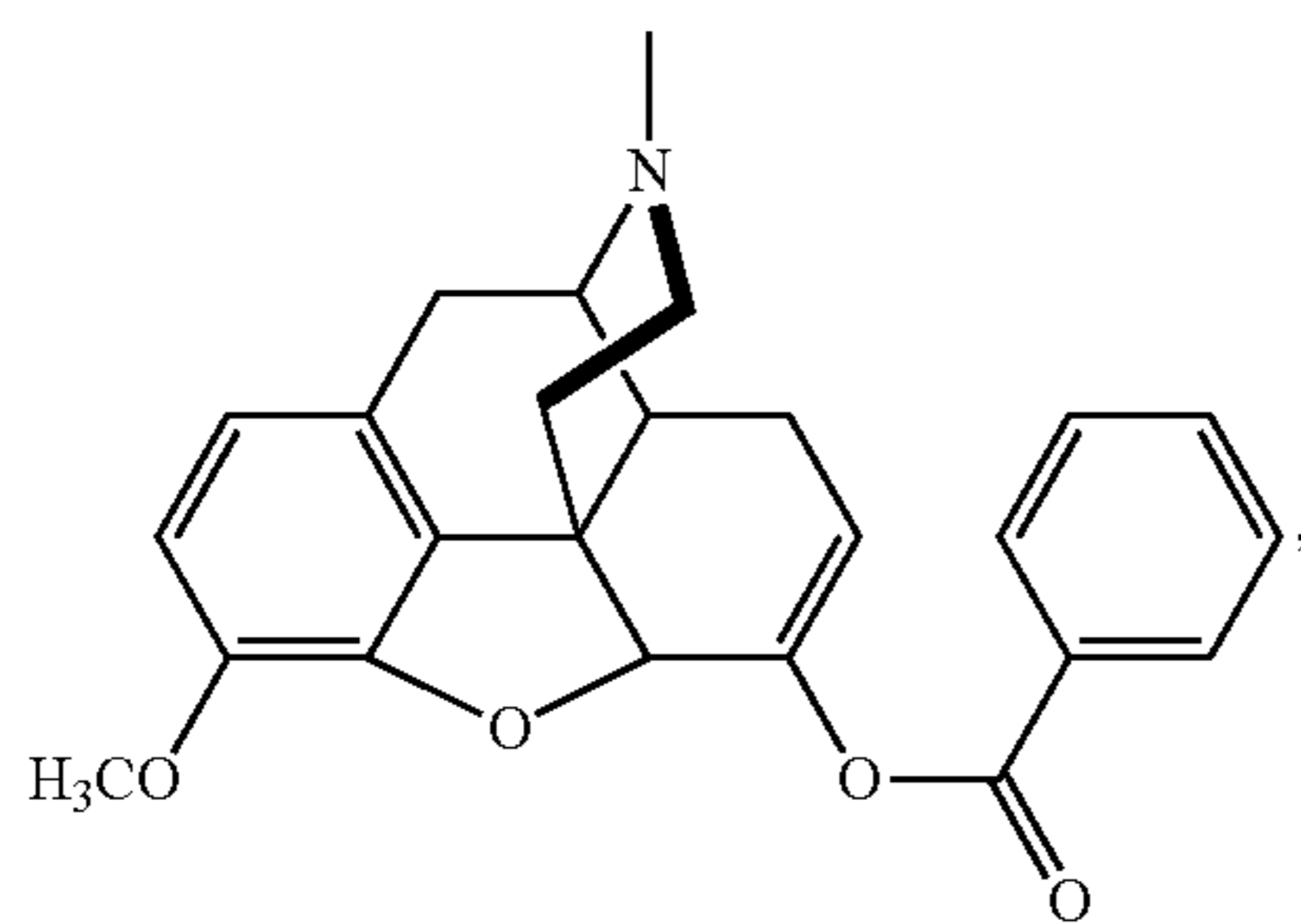
benzoate-hydrocodone (Bz-HC)
