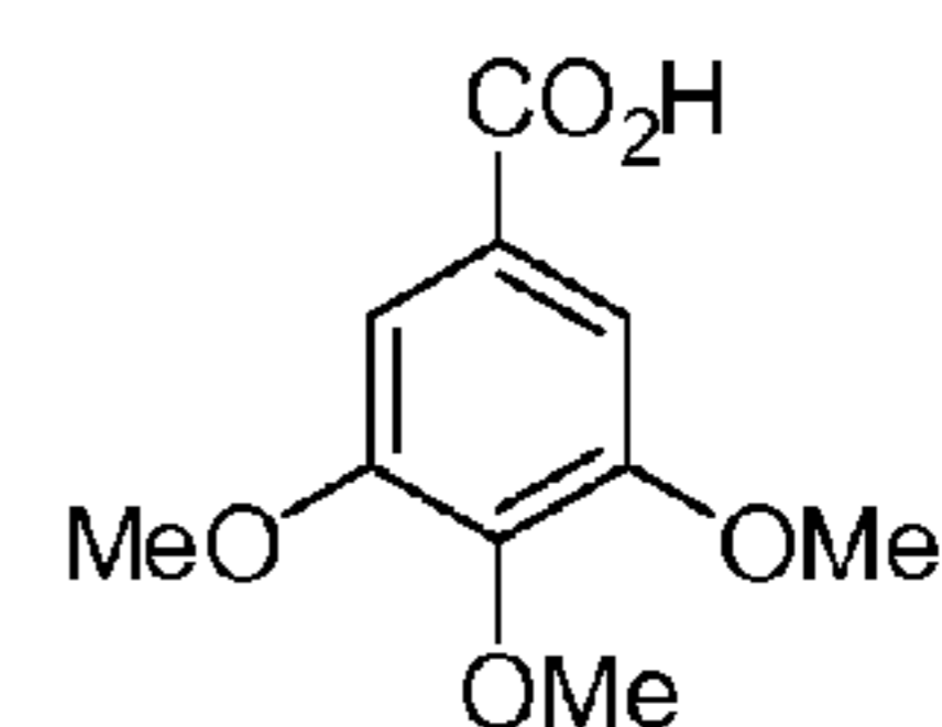
3,4,5-trimethoxybenzoic acid
