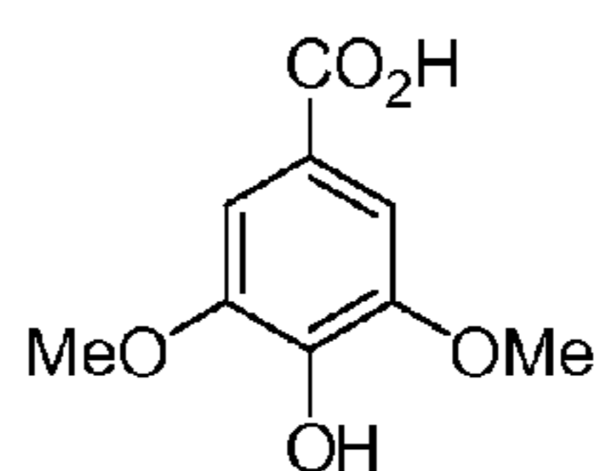
syringic acid
