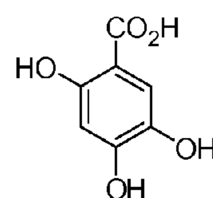
2,4,5-trihydroxybenzoic acid
