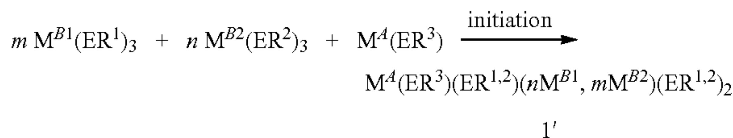
REACTION SCHEME 8:
