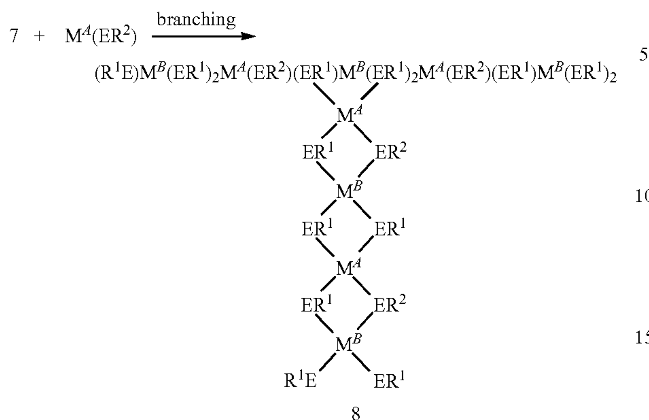
REACTION SCHEME 5:
