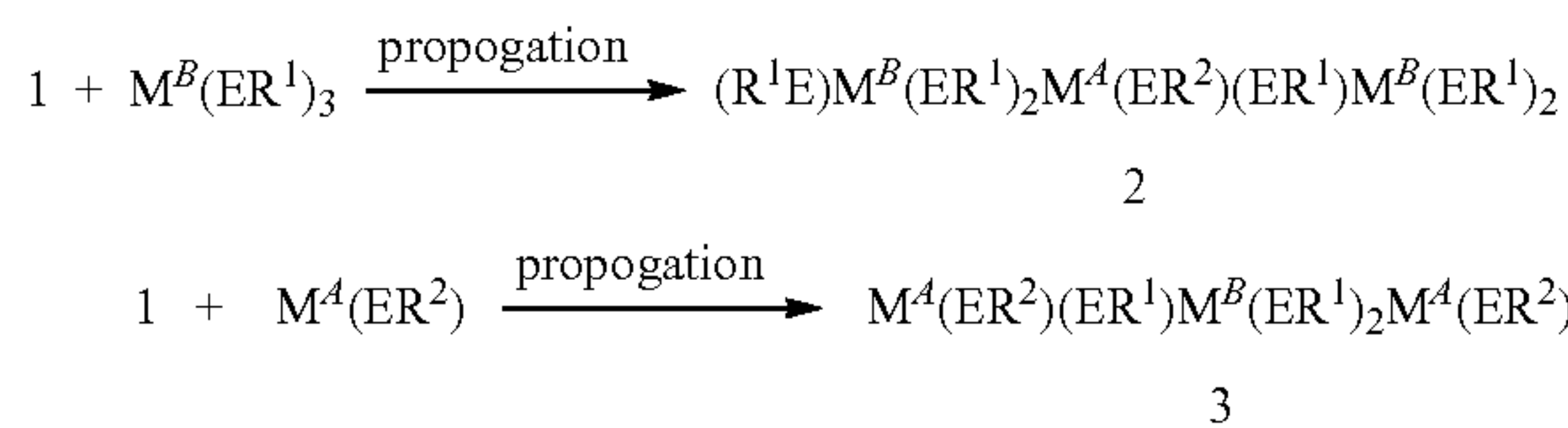
REACTION SCHEME 2:
