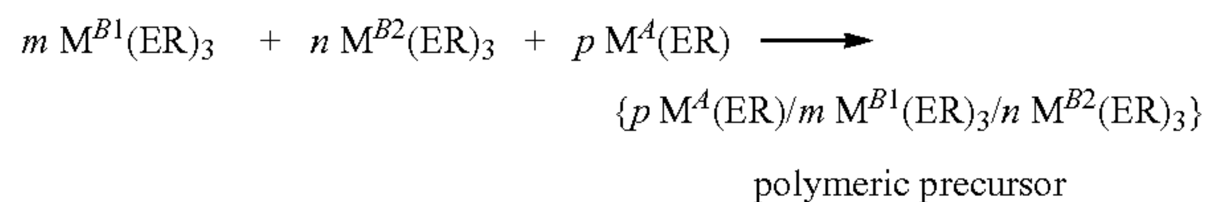
REACTION SCHEME 9:
