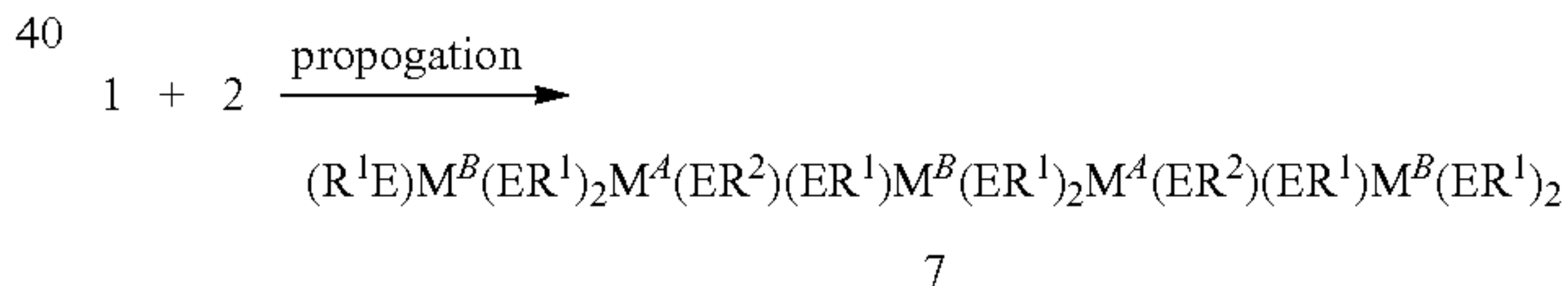
REACTION SCHEME 4:
