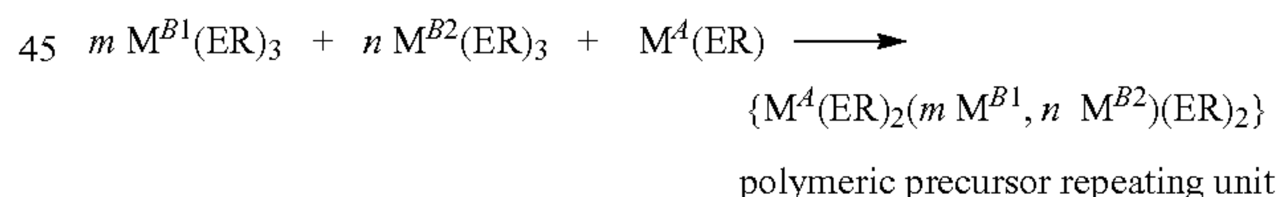
REACTION SCHEME 10:
