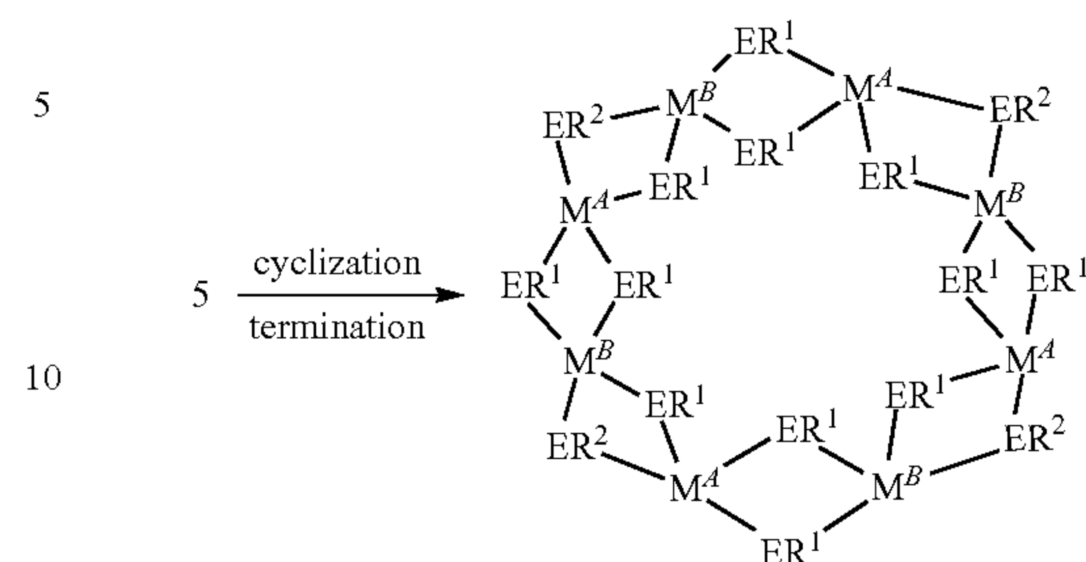
REACTION SCHEME 7:
