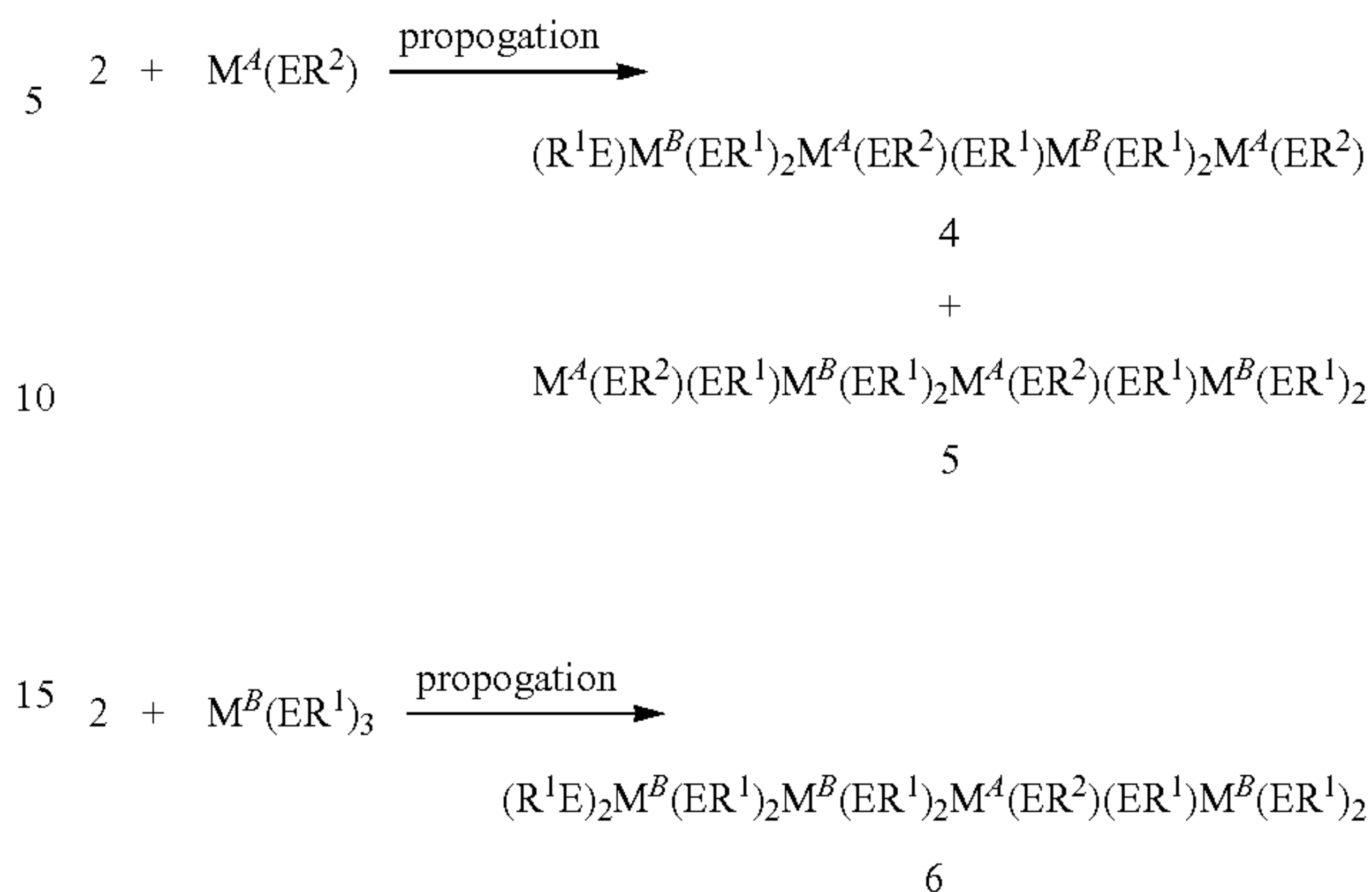
REACTION SCHEME 3:
