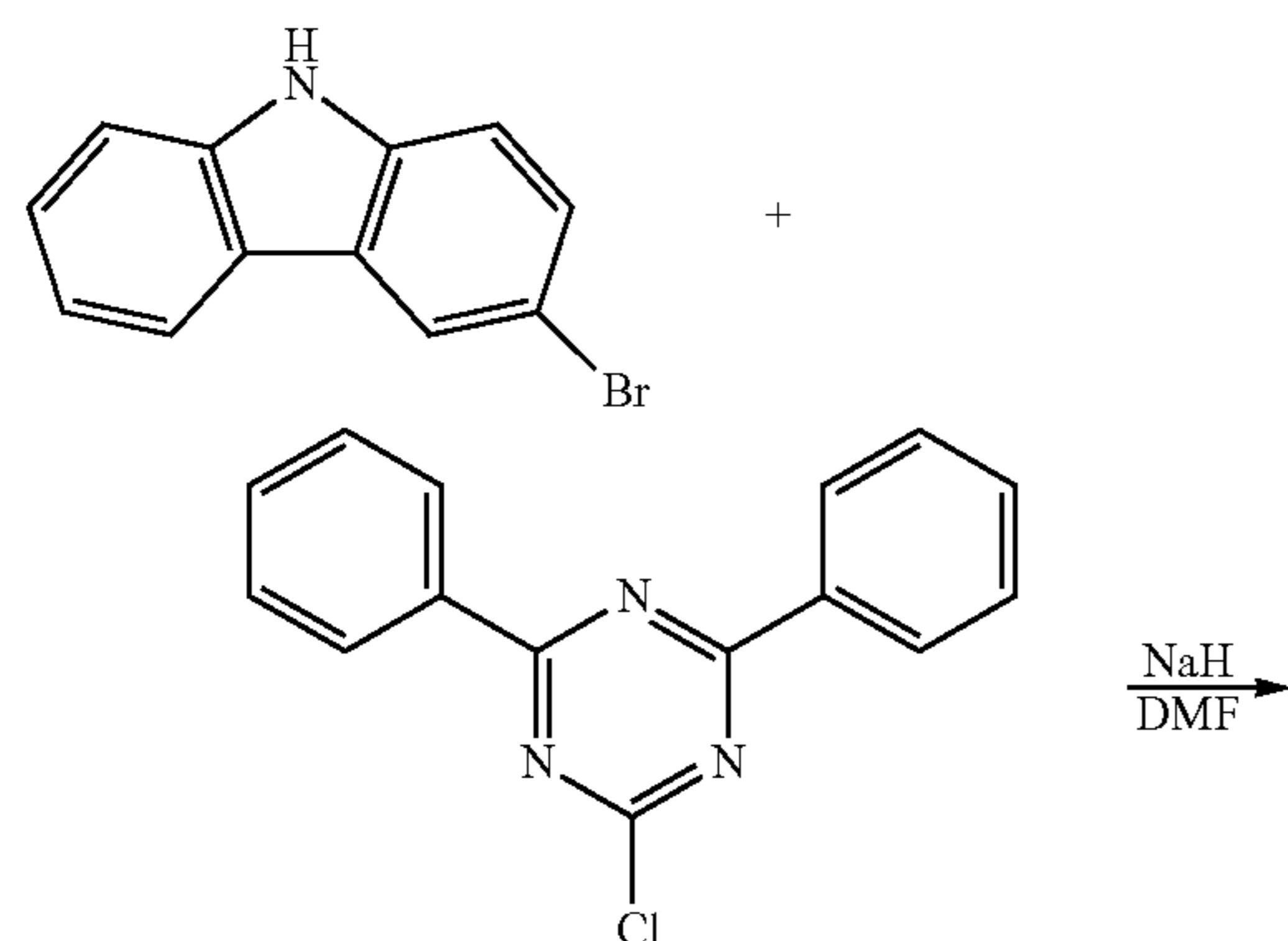
[Reaction Scheme 14]
