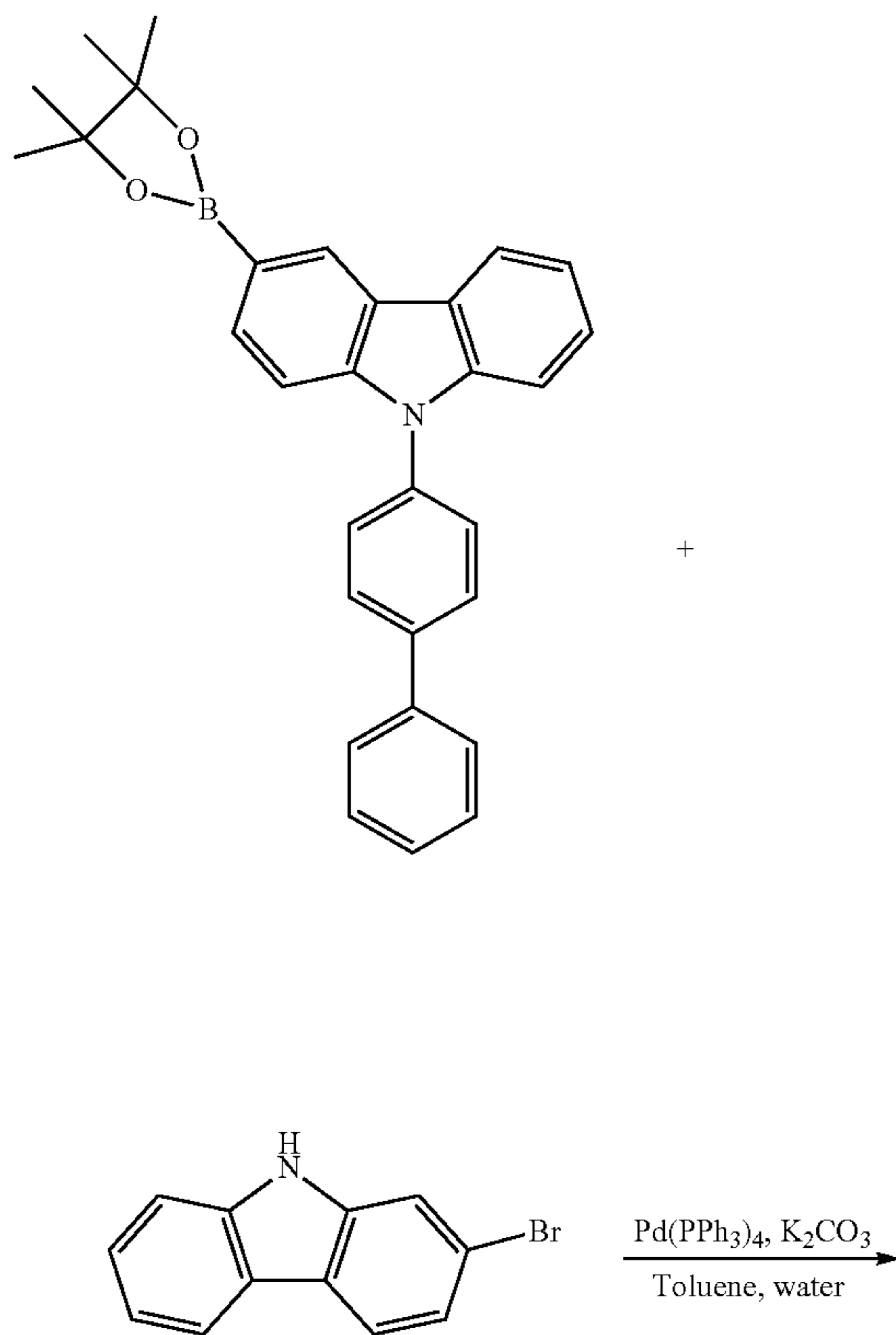
[Reaction Scheme 42]
