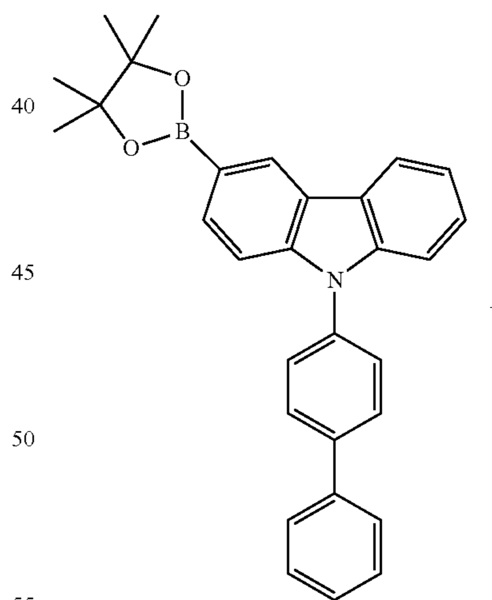
[Reaction Scheme 22]
