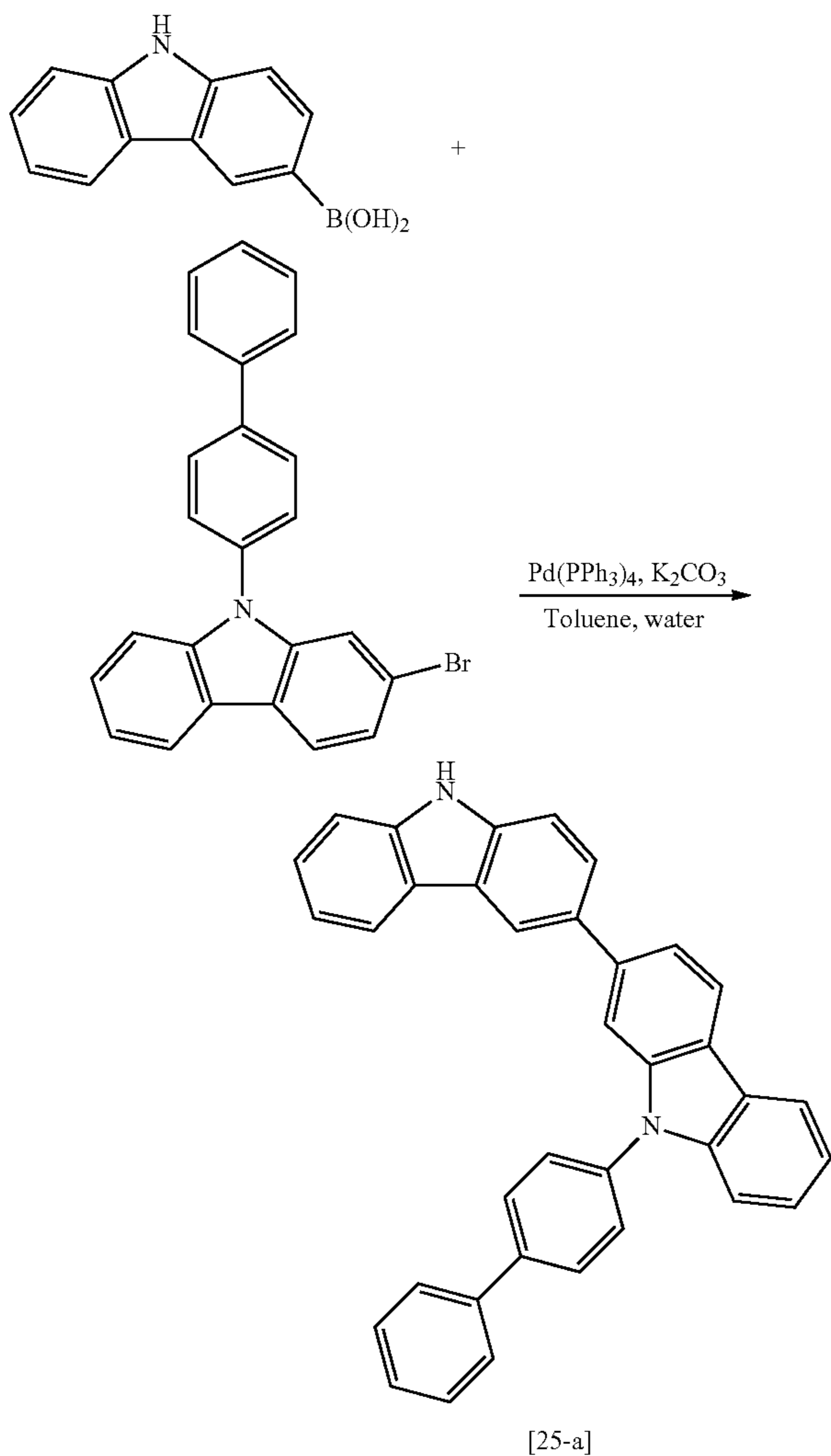
[Reaction Scheme 40]
