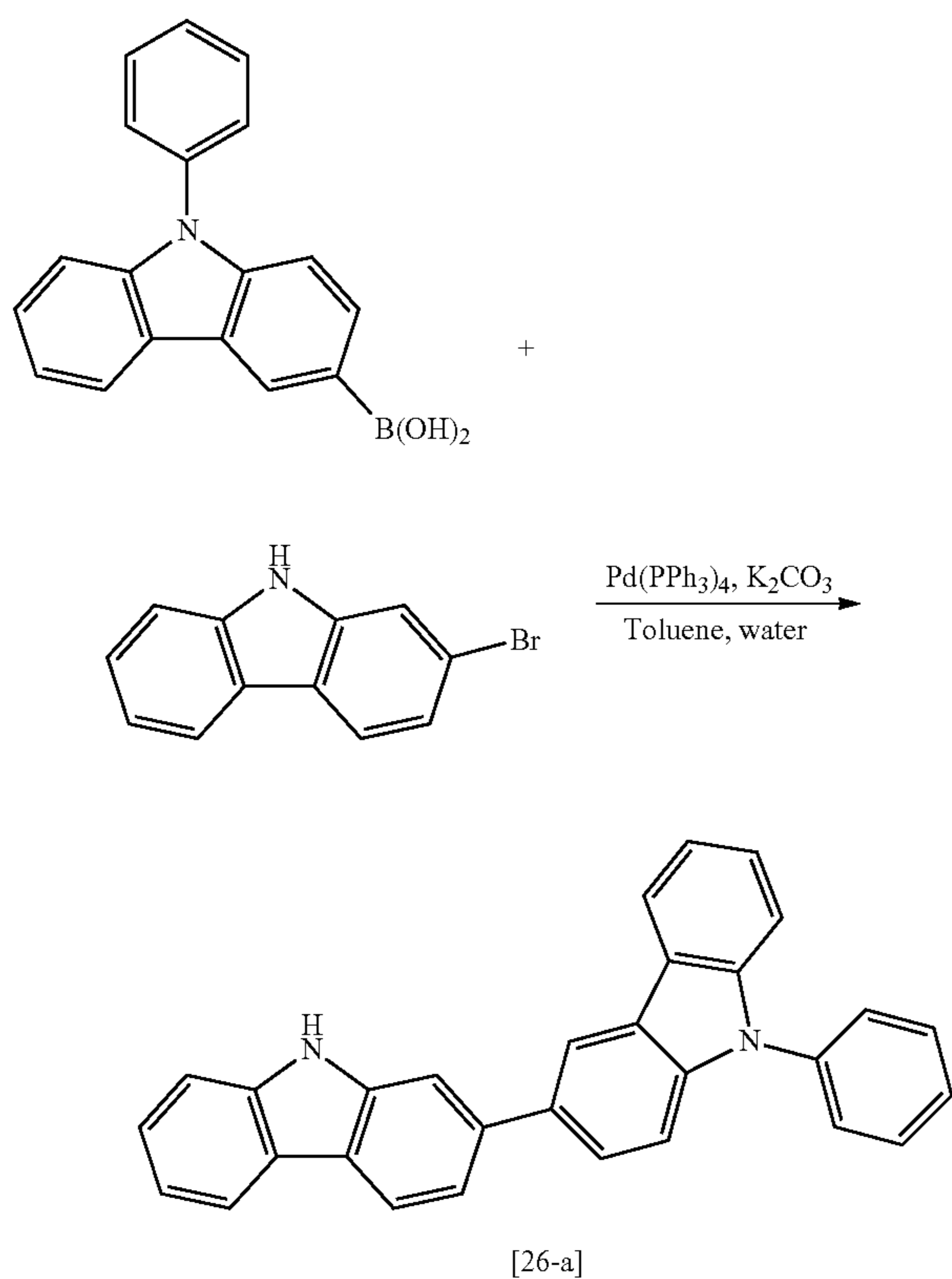
[Reaction Scheme 41]
