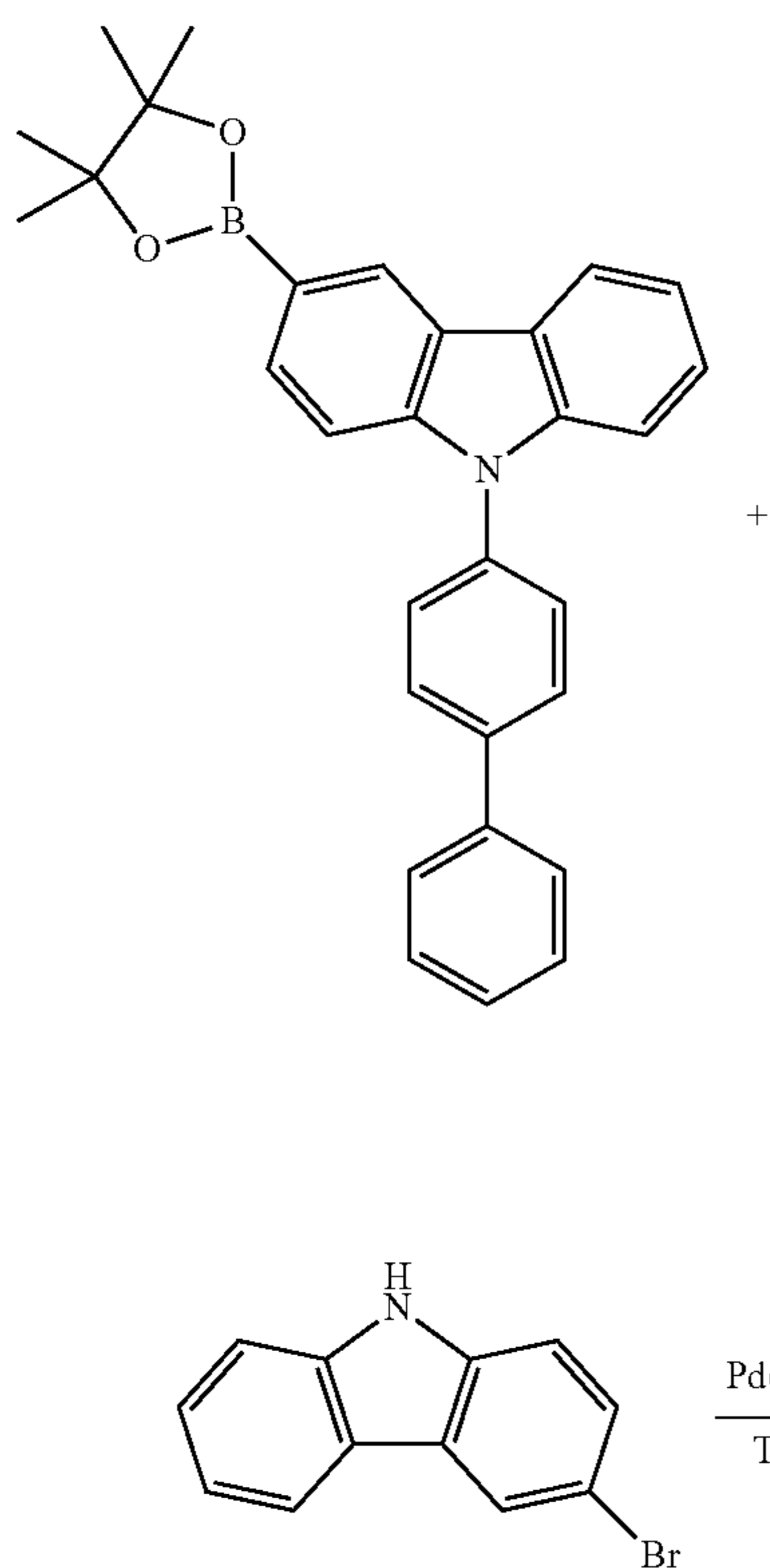
[Reaction Scheme 30]
