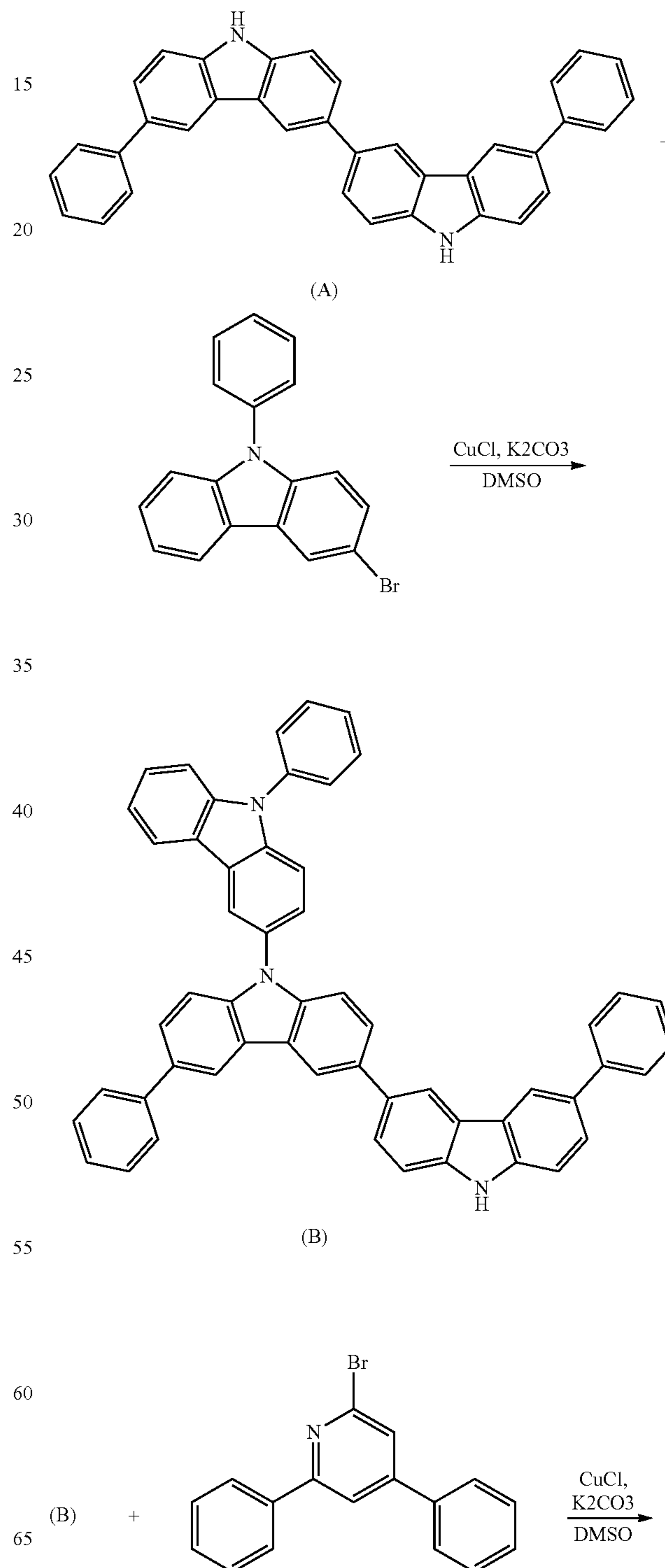
[Reaction Scheme 2]
