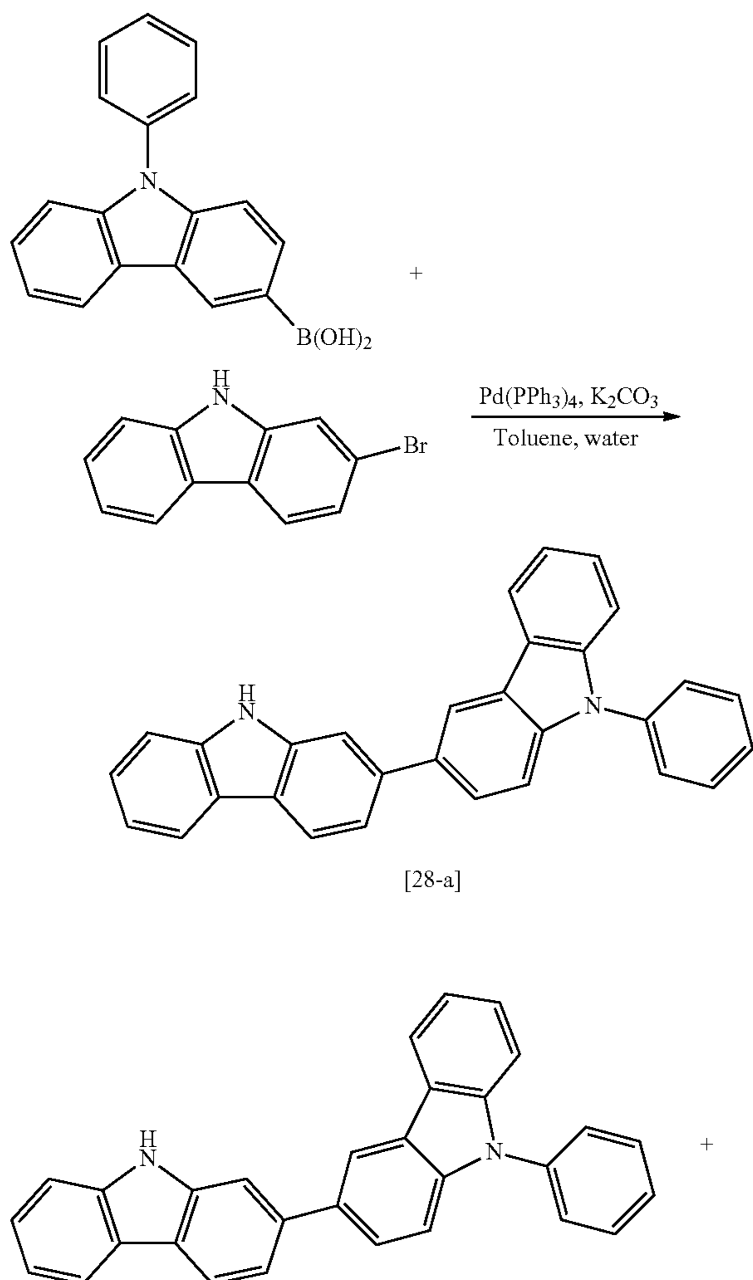
[Reaction Scheme 43]
