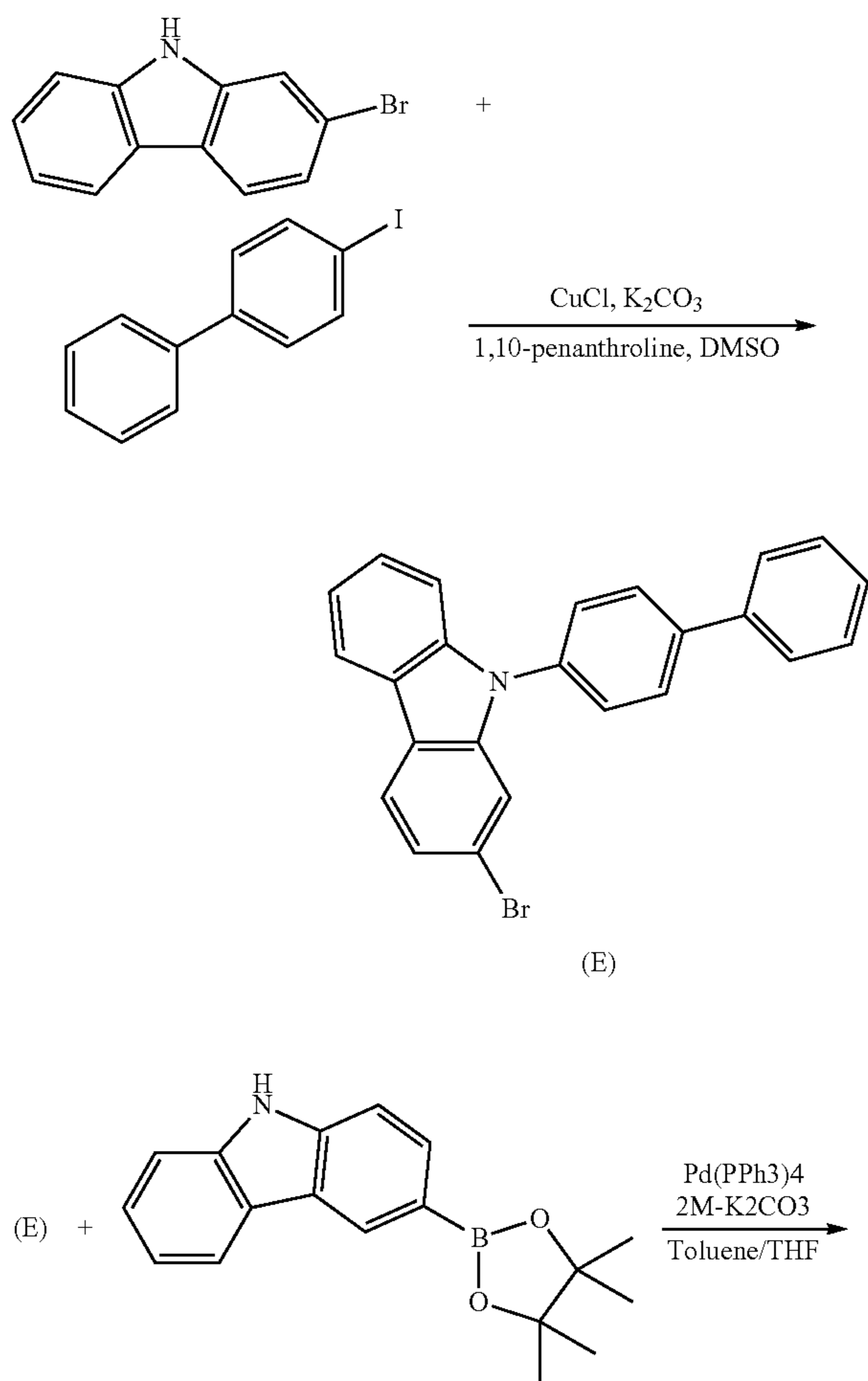
[Reaction Scheme 9]
