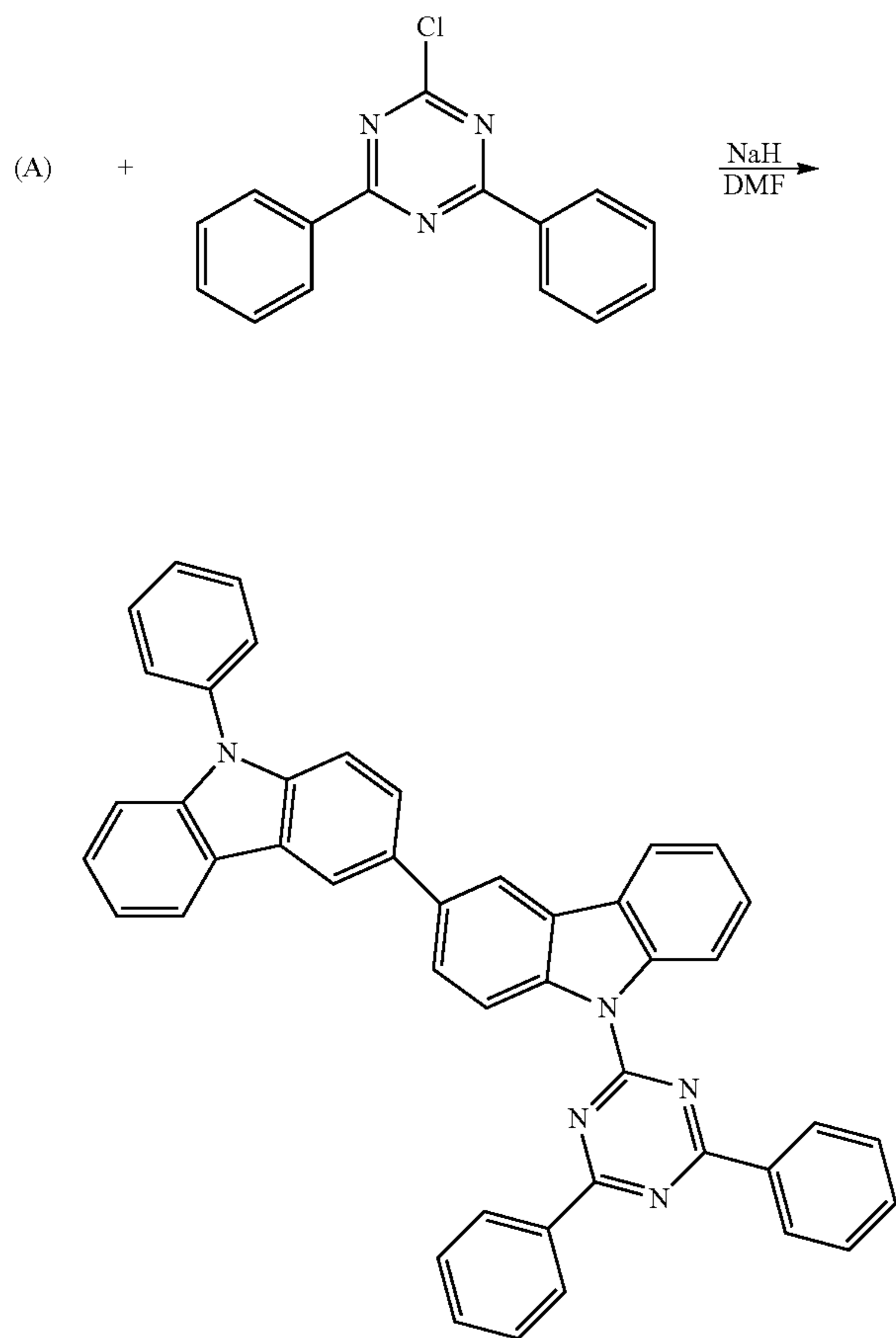
Synthesis of CF N-5
