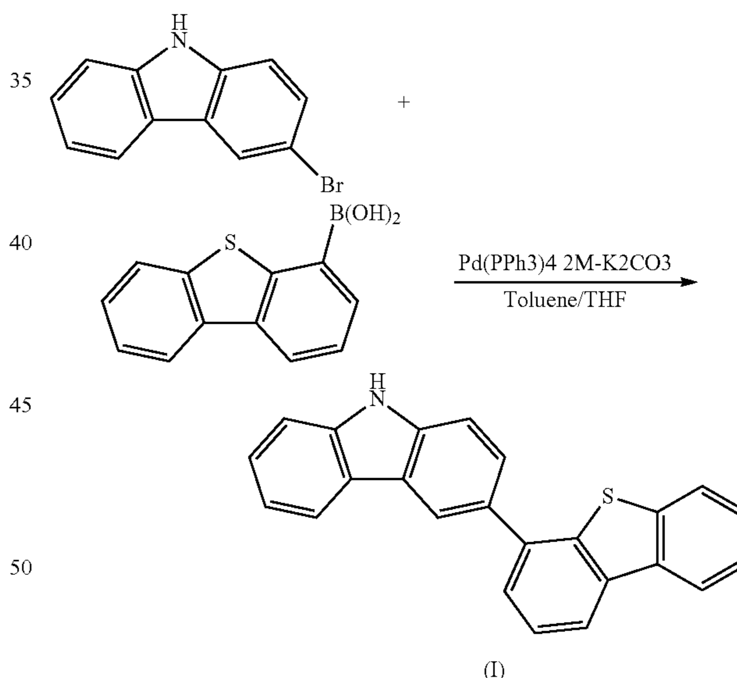
[Reaction Scheme 12]
