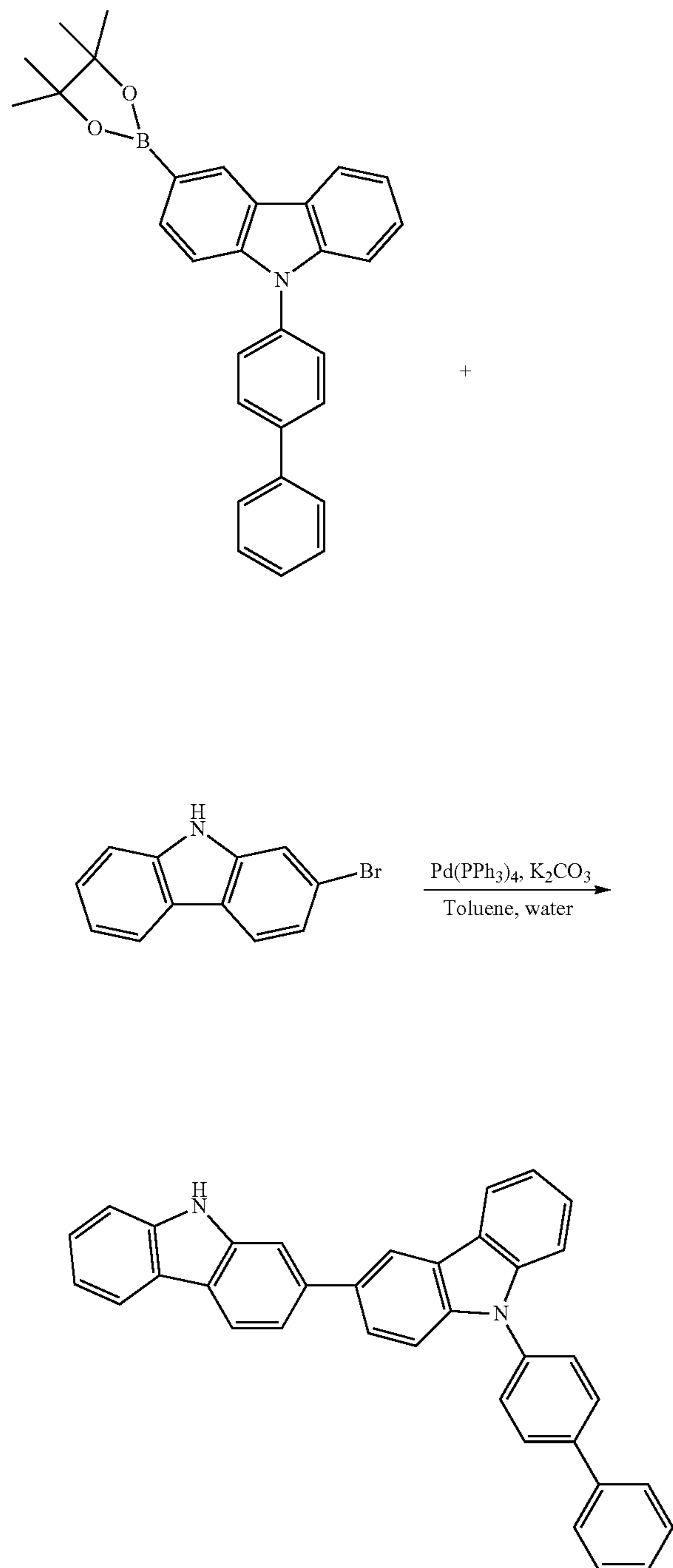
[Reaction Scheme 46]
