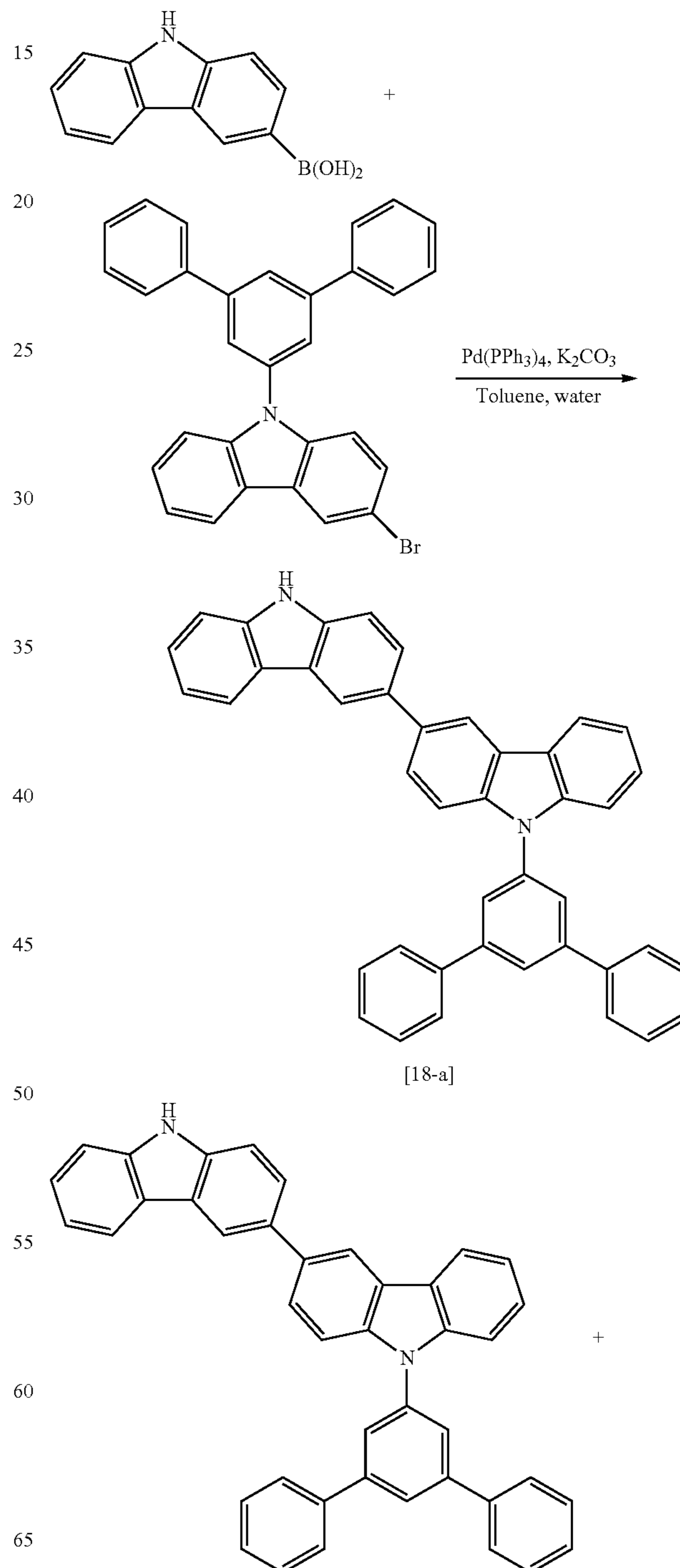
[Reaction Scheme 33]
